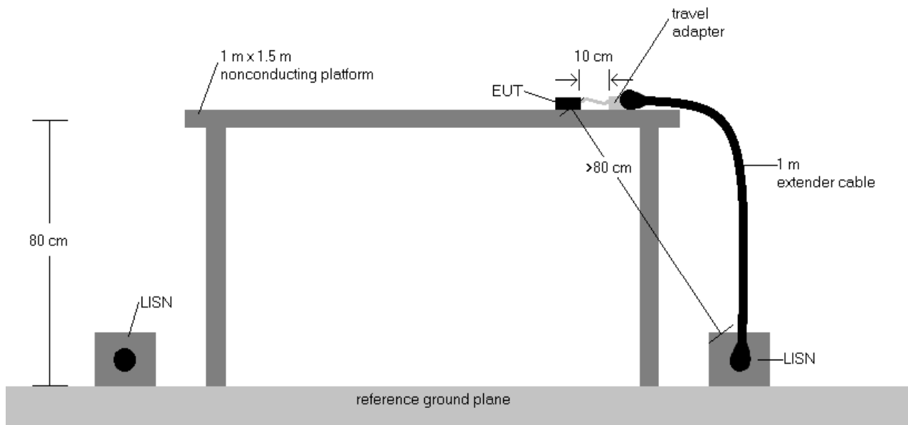
Figure 7-2. Test Instrument & Measurement Setup
