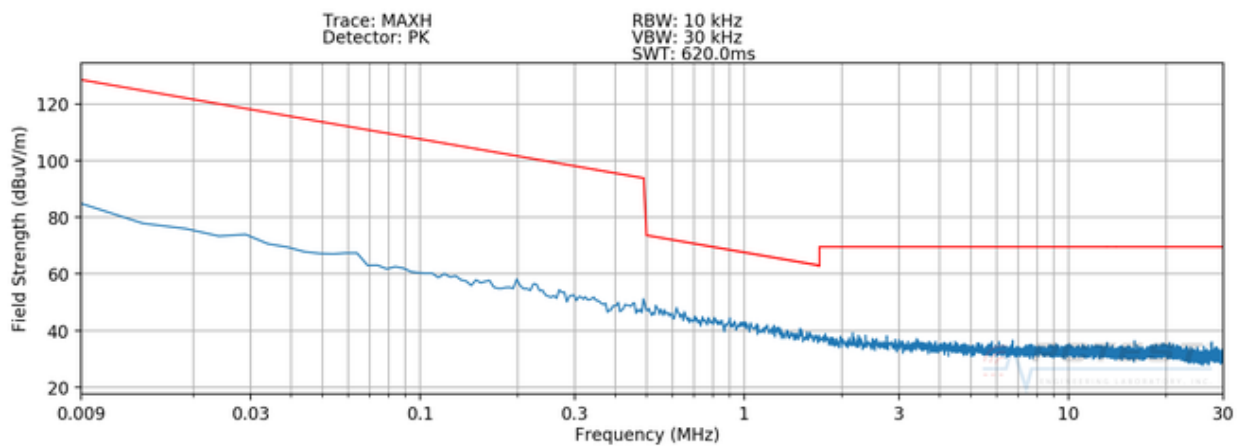
Plot 7-2. Radiated Spurious Plot 9kHz – 30MHz (Pol. Y – WPT - Digitizer Hover)
