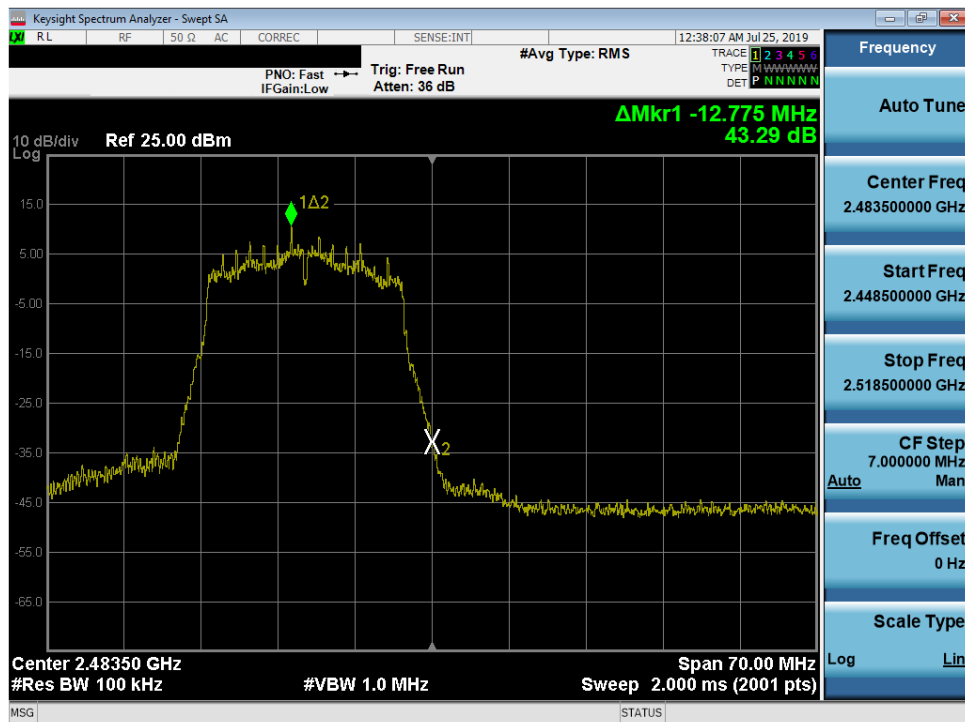
Plot 7-34. Band Edge Plot (802.11n (2.4GHz) – Ch. 13)
