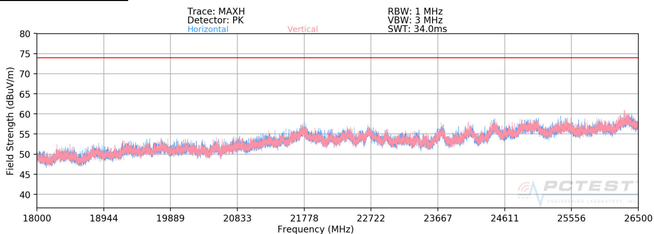
Plot 7-44. Radiated Spurious Plot above 18GHz
