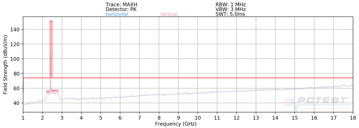
Plot 7-41. Radiated Spurious Plot above 1GHz (802.11b – Ch. 1)
