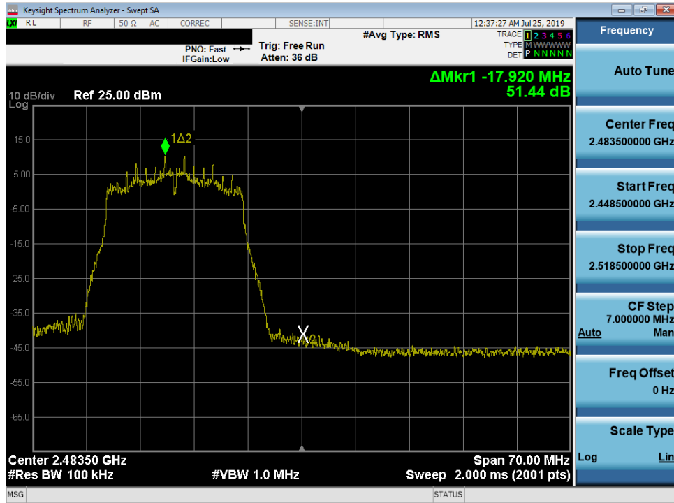
Plot 7-33. Band Edge Plot (802.11n (2.4GHz) – Ch. 12)
