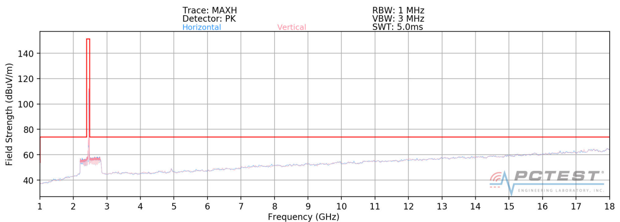
Plot 7-43. Radiated Spurious Plot above 1GHz (802.11b – Ch. 11)
