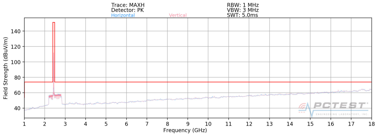
Plot 7-42. Radiated Spurious Plot above 1GHz (802.11b – Ch. 6)
