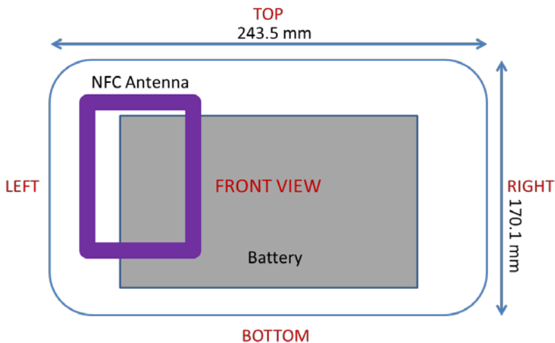
Figure F-1 NFC Antenna Location
