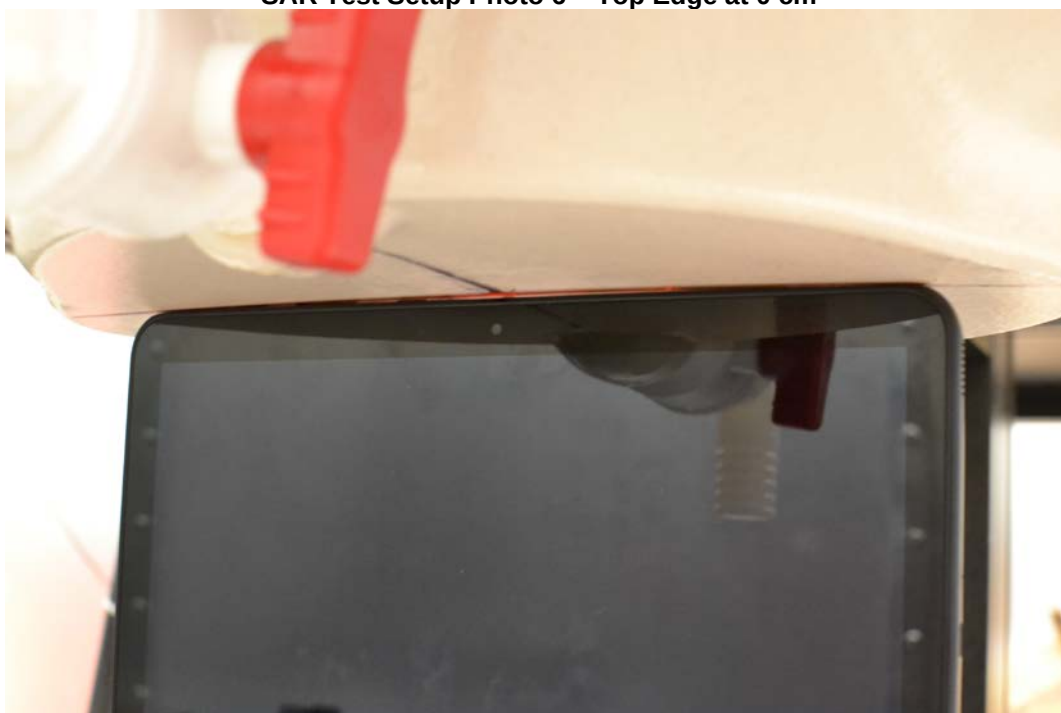
SAR Test Setup Photo 6 – Top Edge at 0 cm
