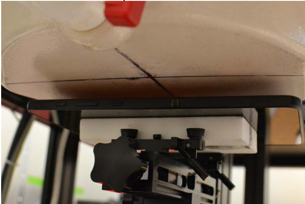
SAR Test Setup Photo 2 – Back Side at 0.8 cm
