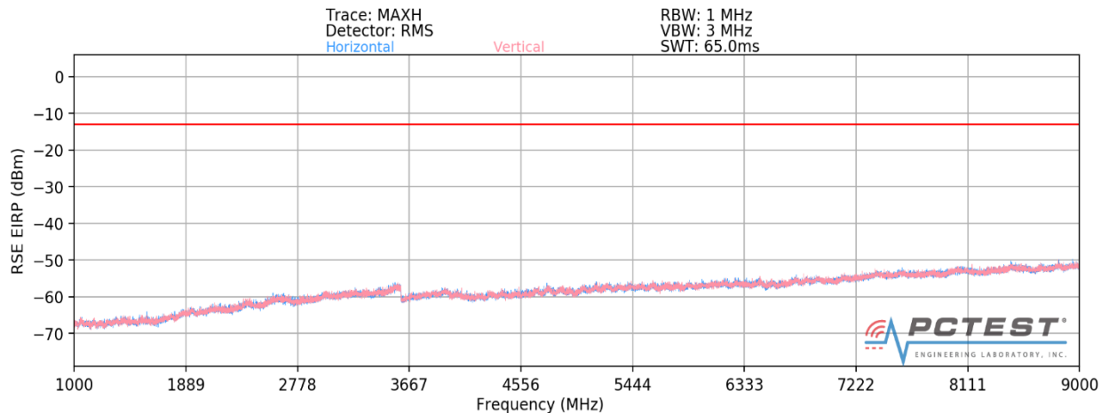
Plot 7-52. Radiated Spurious Plot above 1GHz (LTE Band 26)
