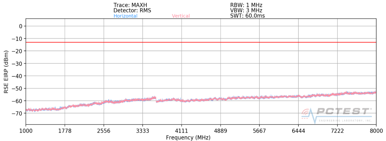
Plot 7-53. Radiated Spurious Plot above 1GHz (LTE Band 26)
