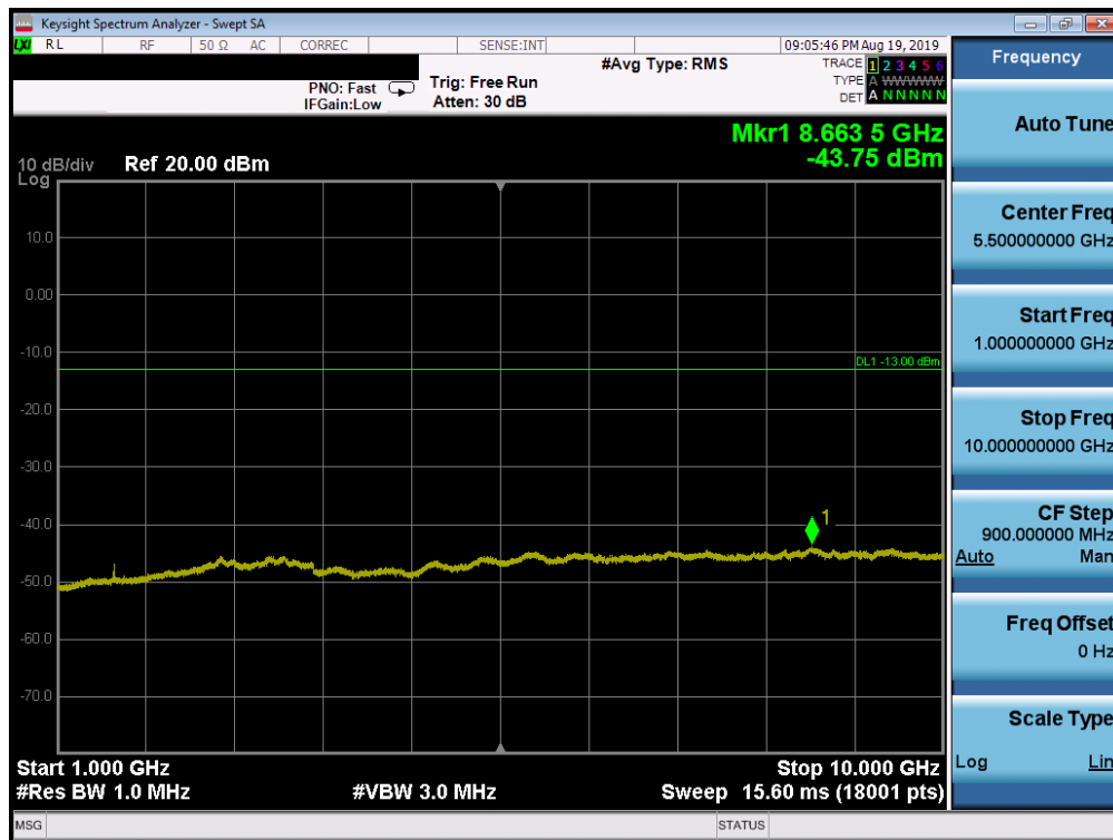
Plot 7-30. Conducted Spurious Plot (LTE Band 14, 5.0 MHz QPSK – RB Size 1, RB Offset 0 – Low Channel)
