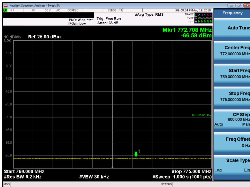
Plot 7-43. Lower Emission Mask Plot (LTE Band 14, 5MHz QPSK – RB Size 25)
