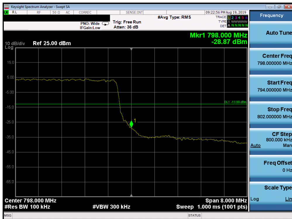
Plot 7-48. Upper Band Edge Plot (LTE Band 14, 10MHz QPSK – RB Size 50)
