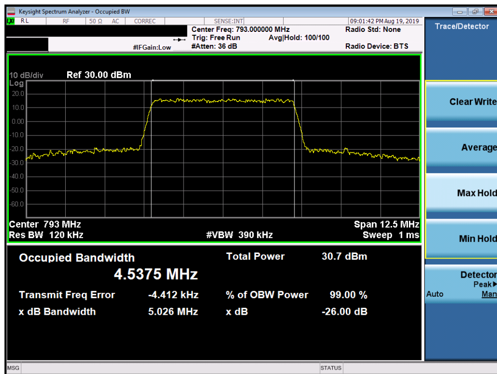
Plot 7-17. Occupied Bandwidth Plot (LTE Band 14, 5MHz 16-QAM – RB Size 25)
