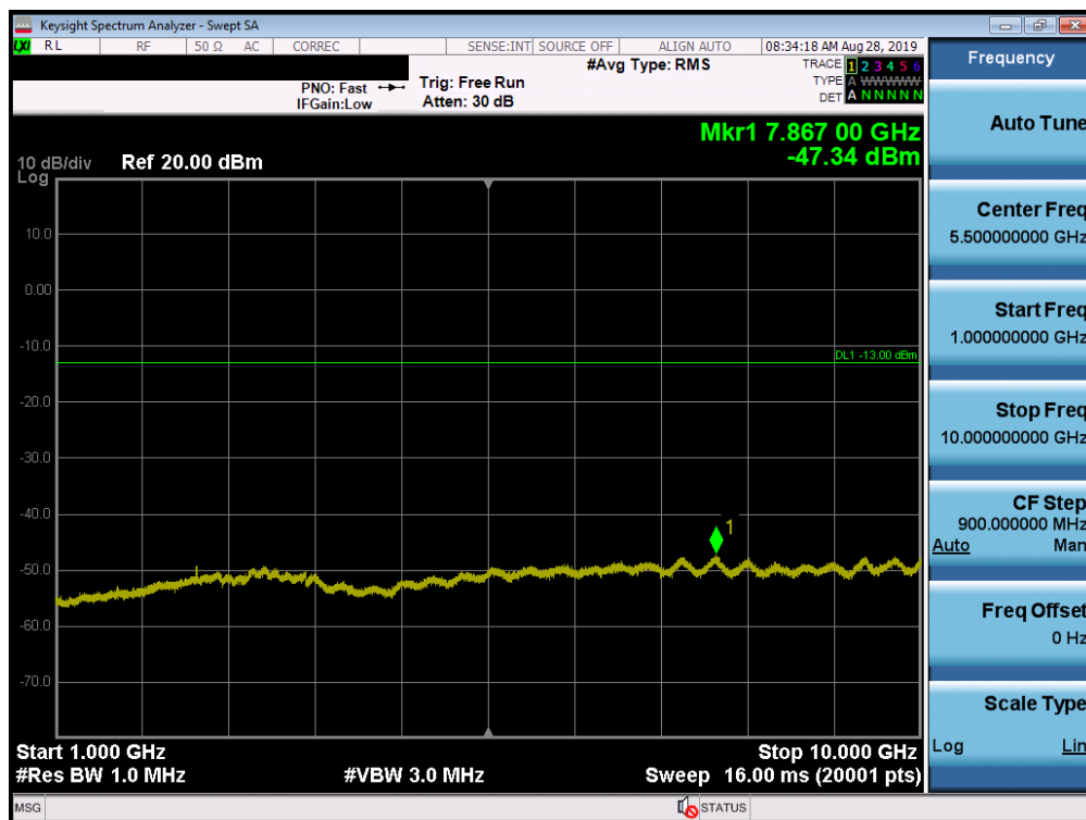
Plot 7-27. Conducted Spurious Plot (LTE Band 26, 5.0 MHz QPSK – RB Size 1, RB Offset 0 – High Channel)
