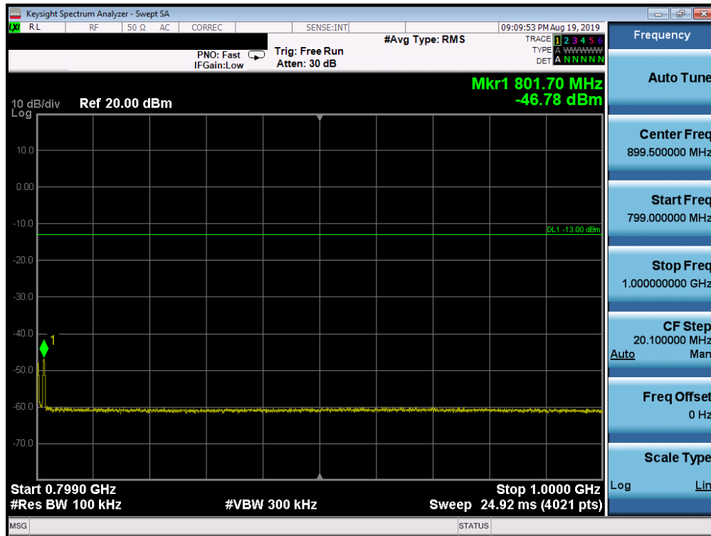
Plot 7-32. Conducted Spurious Plot (LTE Band 14, 5.0 MHz QPSK – RB Size 1, RB Offset 0 – High Channel)
