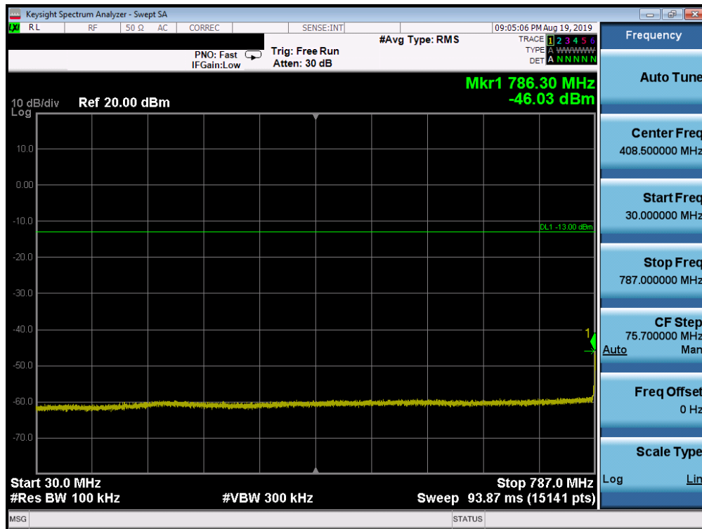
Plot 7-28. Conducted Spurious Plot (LTE Band 14, 5.0 MHz QPSK – RB Size 1, RB Offset 0 – Low Channel)
