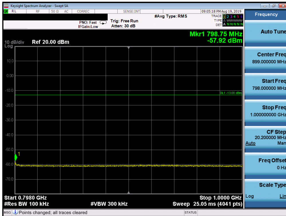
Plot 7-29. Conducted Spurious Plot (LTE Band 14, 5.0 MHz QPSK – RB Size 1, RB Offset 0 – Low Channel)
