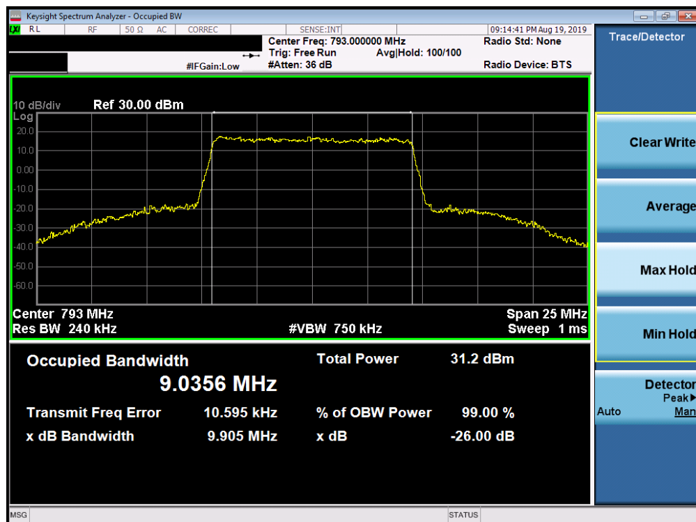
Plot 7-20. Occupied Bandwidth Plot (LTE Band 14, 10MHz 16-QAM – RB Size 50)
