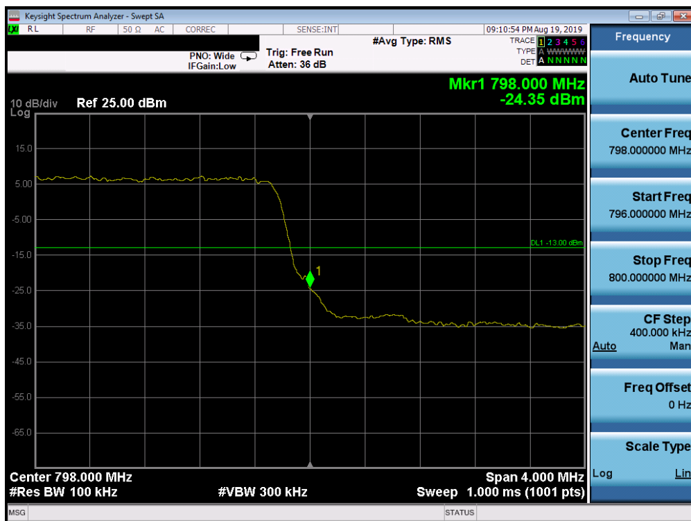
Plot 7-44. Upper Band Edge Plot (LTE Band 14, 5MHz QPSK – RB Size 25)
