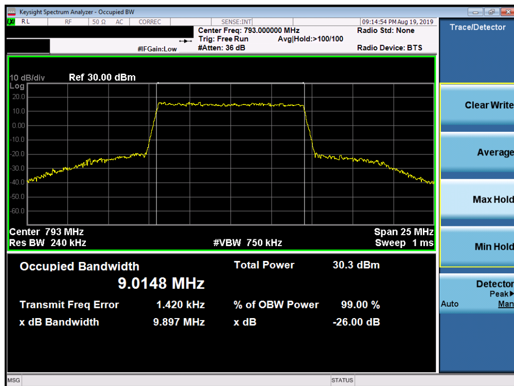
Plot 7-21. Occupied Bandwidth Plot (LTE Band 14, 10MHz 64-QAM – RB Size 50)
