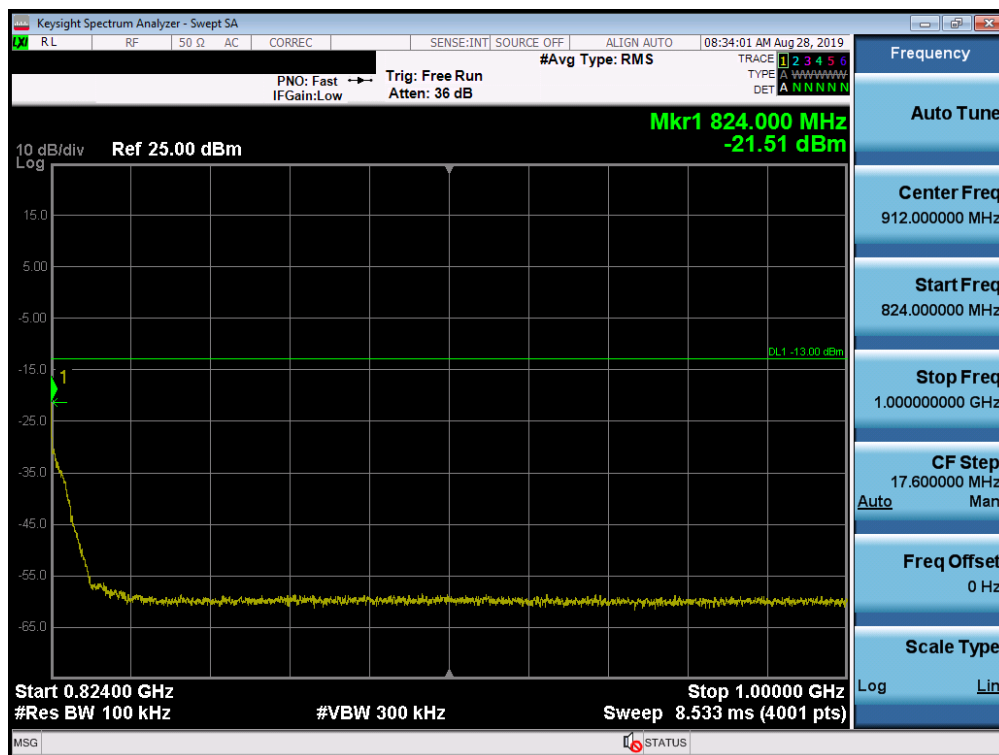
Plot 7-26. Conducted Spurious Plot (LTE Band 26, 5.0 MHz QPSK – RB Size 1, RB Offset 0 – High Channel)
