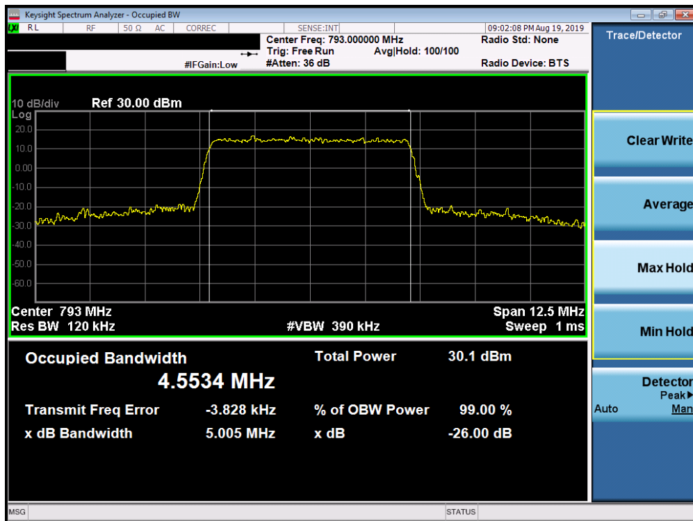
Plot 7-18. Occupied Bandwidth Plot (LTE Band 14, 5MHz 64-QAM – RB Size 25)
