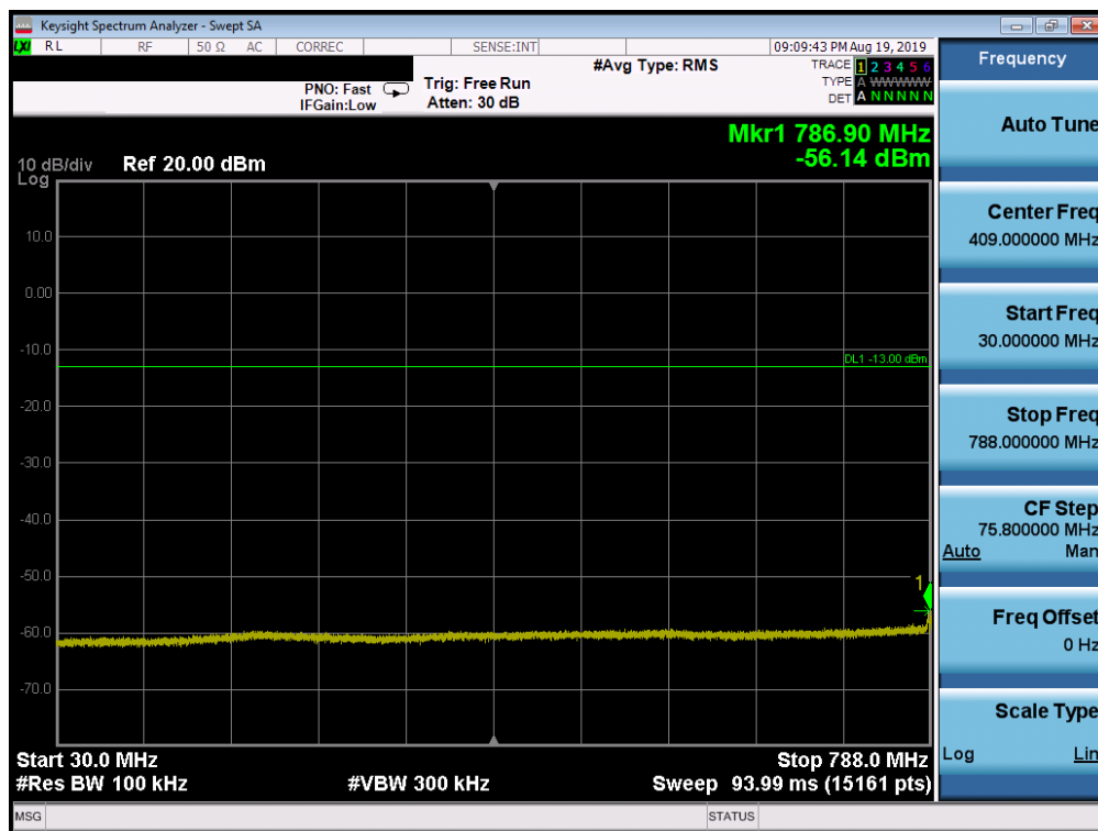
Plot 7-31. Conducted Spurious Plot (LTE Band 14, 5.0 MHz QPSK – RB Size 1, RB Offset 0 – High Channel)
