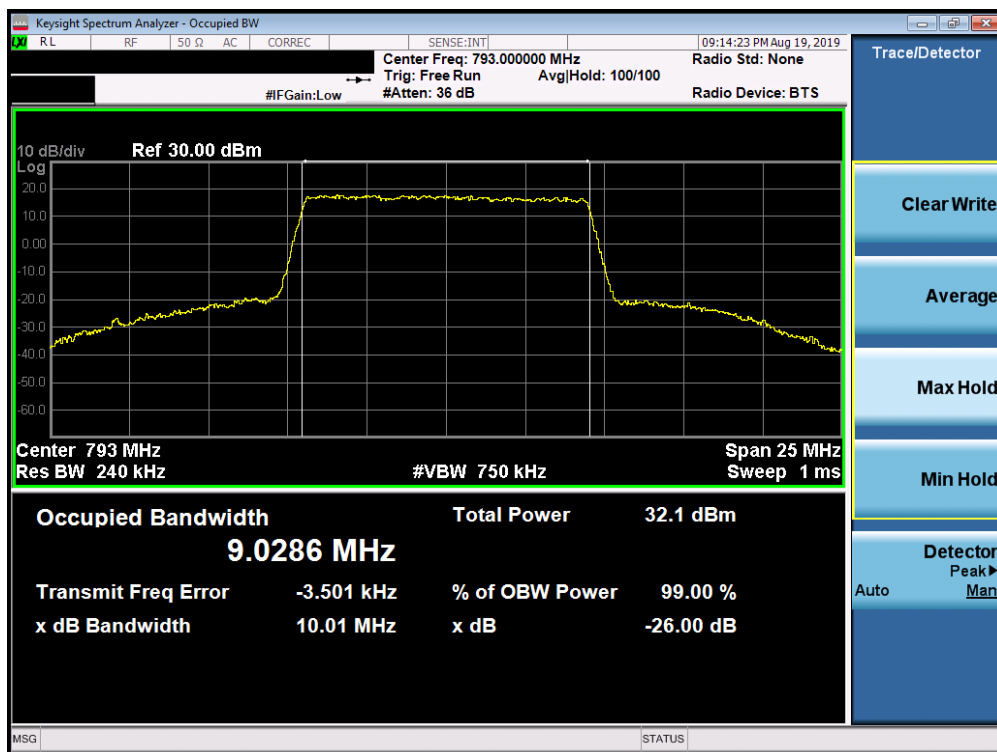
Plot 7-19. Occupied Bandwidth Plot (LTE Band 14, 10MHz QPSK – RB Size 50)
