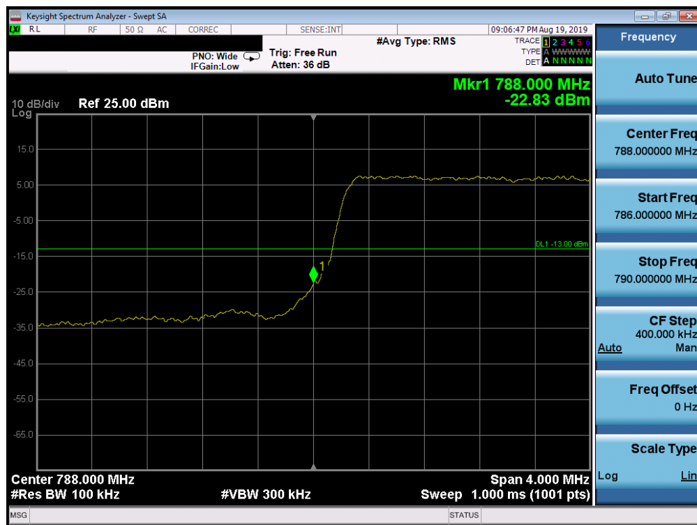
Plot 7-42. Lower Band Edge Plot (LTE Band 14, 5MHz QPSK – RB Size 25)
