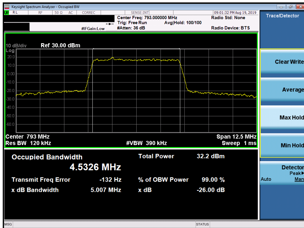
Plot 7-16. Occupied Bandwidth Plot (LTE Band 14, 5MHz QPSK – RB Size 25)
