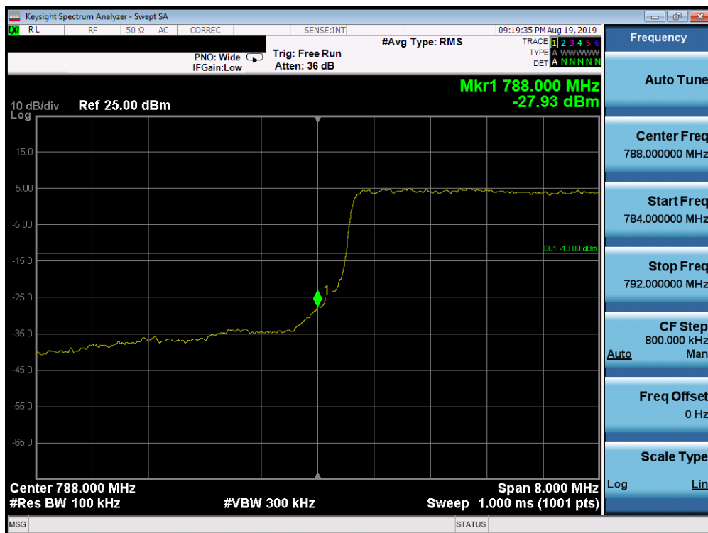
Plot 7-46. Lower Band Edge Plot (LTE Band 14, 10MHz QPSK – RB Size 50)
