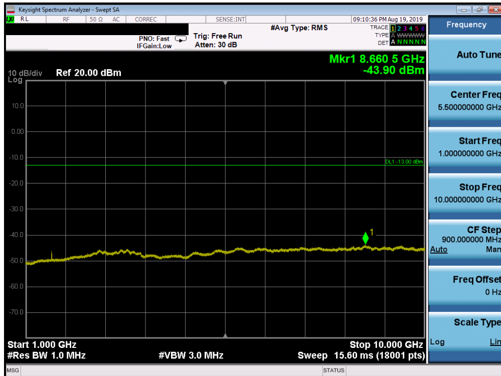
Plot 7-33. Conducted Spurious Plot (LTE Band 14, 5.0 MHz QPSK – RB Size 1, RB Offset 0 – High Channel)
