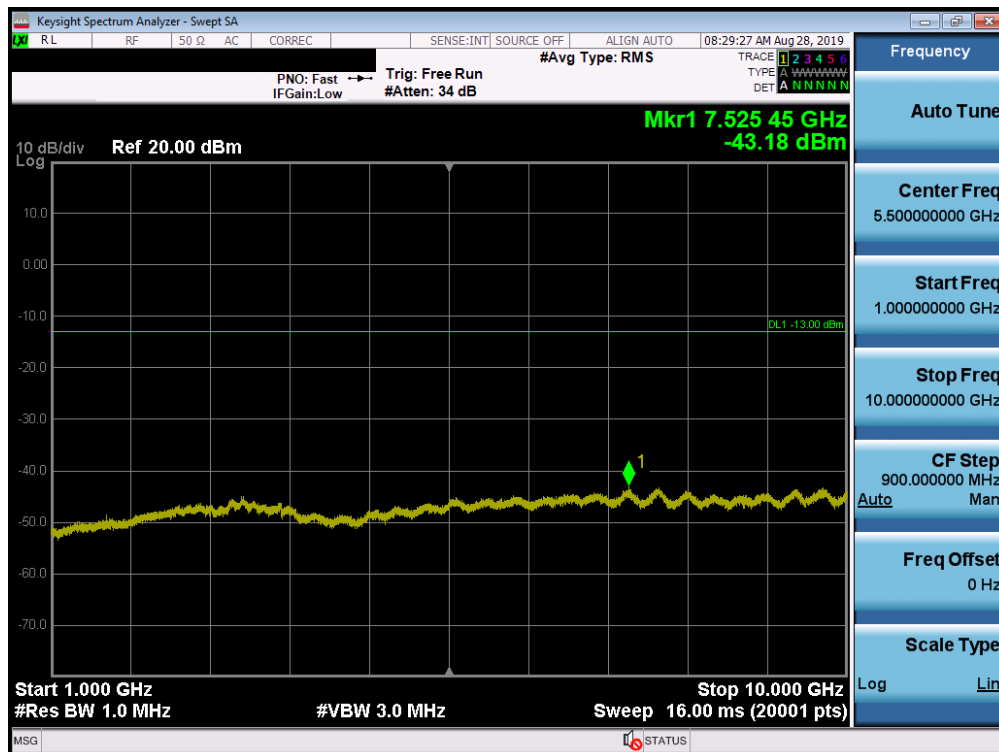
Plot 7-24. Conducted Spurious Plot (LTE Band 26, 5.0 MHz QPSK – RB Size 1, RB Offset 0 – Low Channel)
