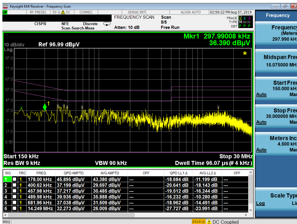
Plot 7-8. Line-Conducted Test Plot (N) – Digitizer Hover
