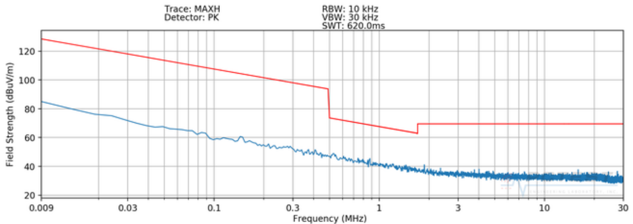
Plot 7-5. Radiated Spurious Plot 9kHz – 30MHz (Pol. Y – WPT - Digitizer S-Pen Click)
