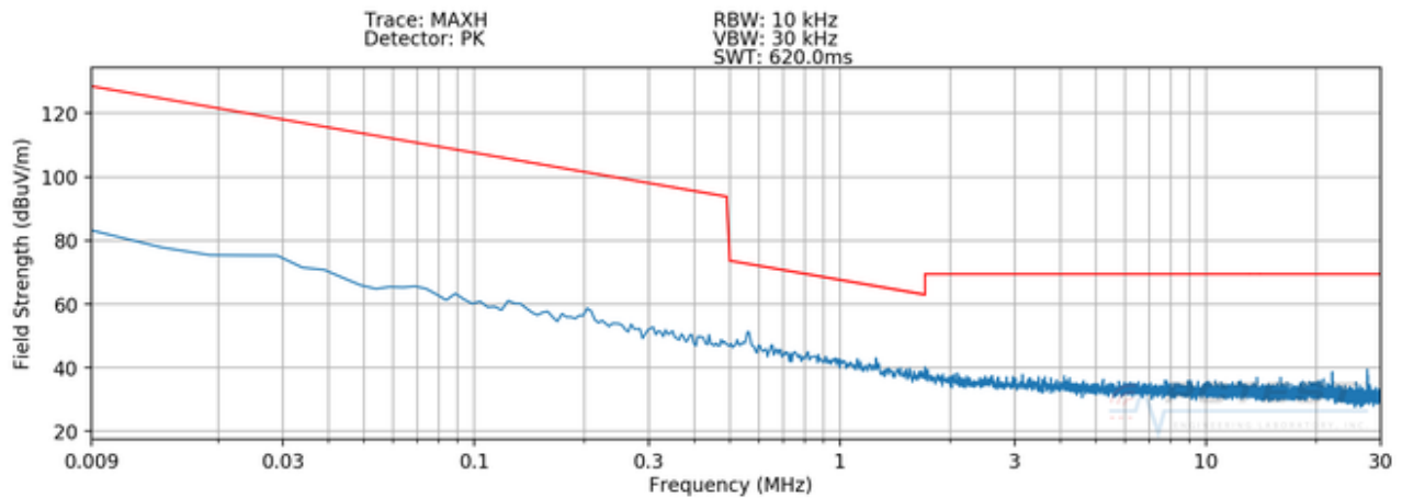
Plot 7-3. Radiated Spurious Plot 9kHz – 30MHz (Pol. Z – WPT - Digitizer Hover)
