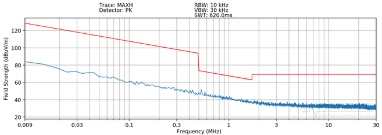
Plot 7-4. Radiated Spurious Plot 9kHz – 30MHz (Pol. X – WPT – Digitizer S-Pen Click)
