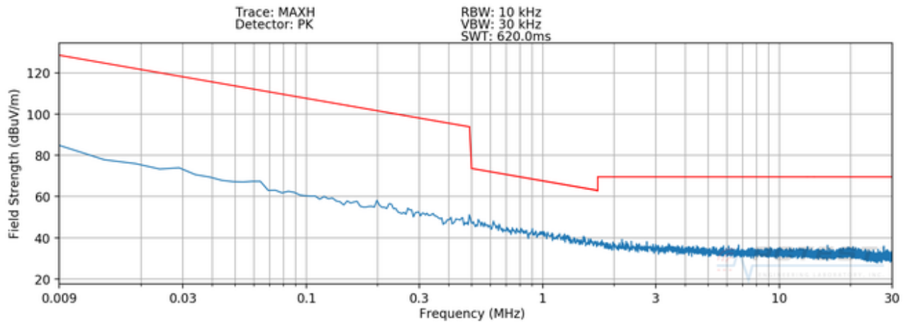
Plot 7-2. Radiated Spurious Plot 9kHz – 30MHz (Pol. Y – WPT - Digitizer Hover)
