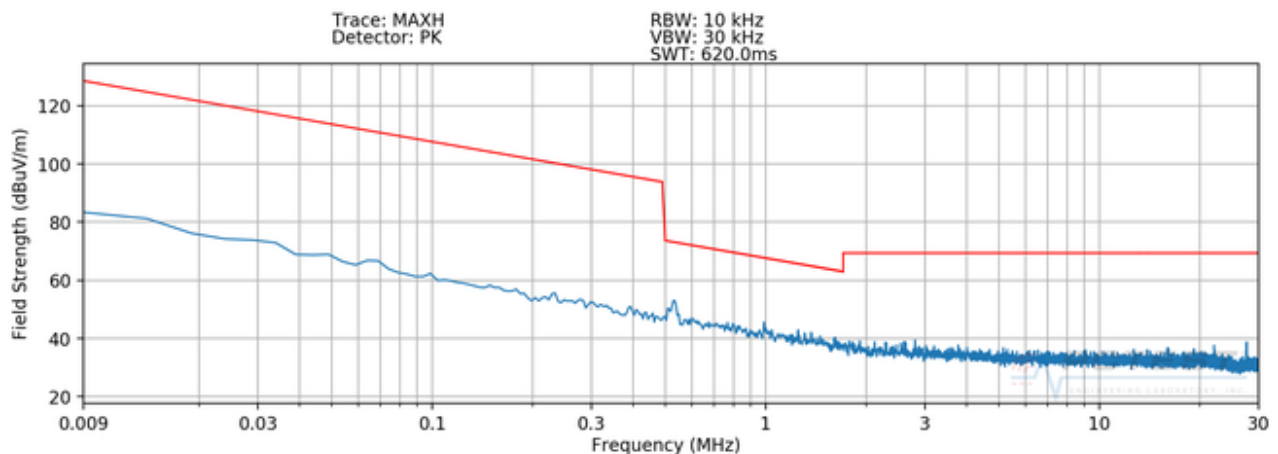
Plot 7-6. Radiated Spurious Plot 9kHz – 30MHz (Pol. Z – WPT - Digitizer S-Pen Click)
