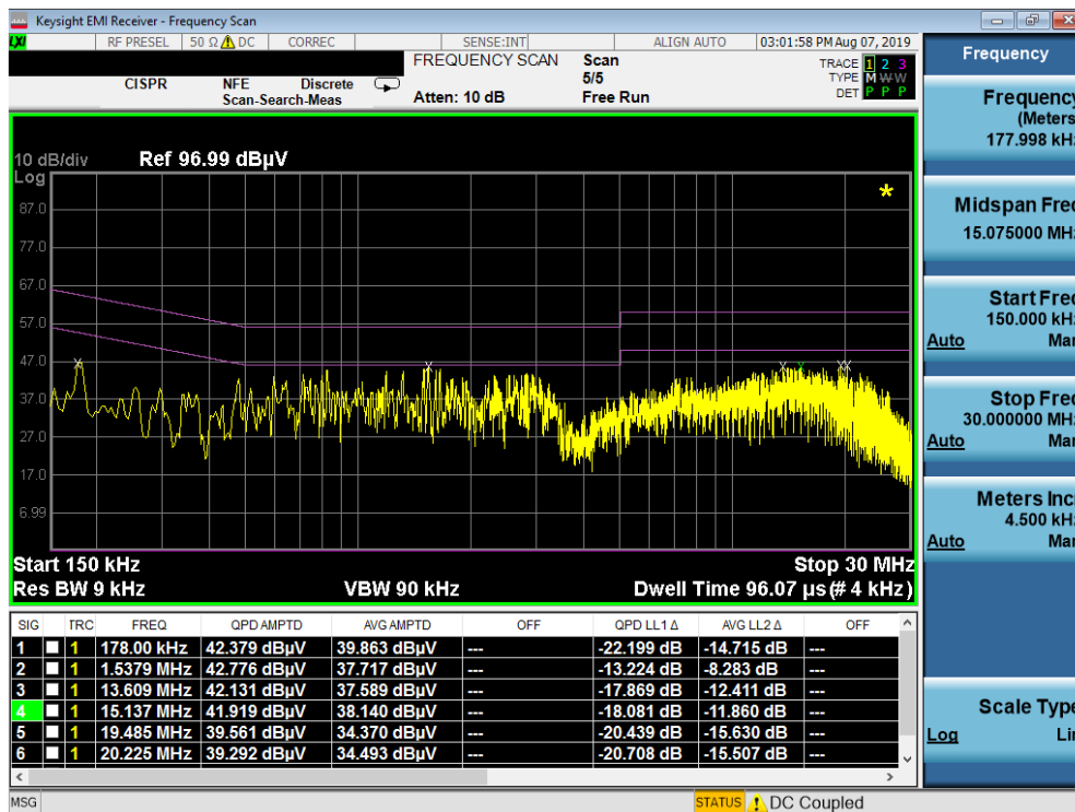
Plot 7-9. Line-Conducted Test Plot (L1) – Digitizer S-Pen Click
