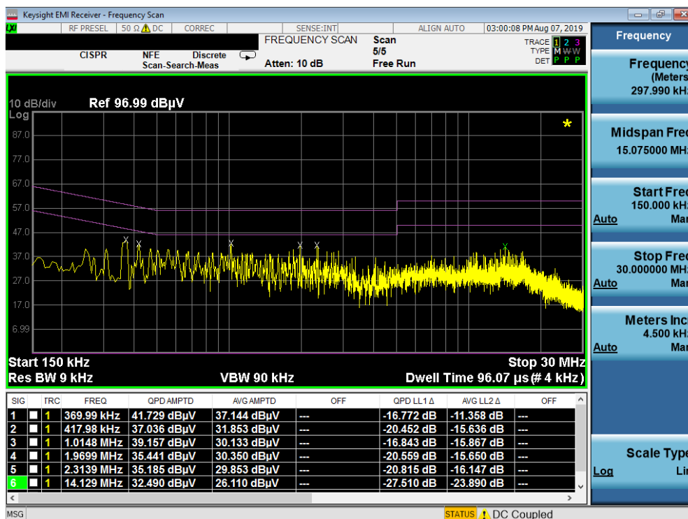
Plot 7-10. Line-Conducted Test Plot (N) – Digitizer S-Pen Click
