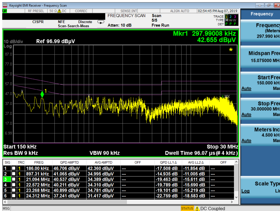
Plot 7-7. Line-Conducted Test Plot (L1) – Digitizer Hover
