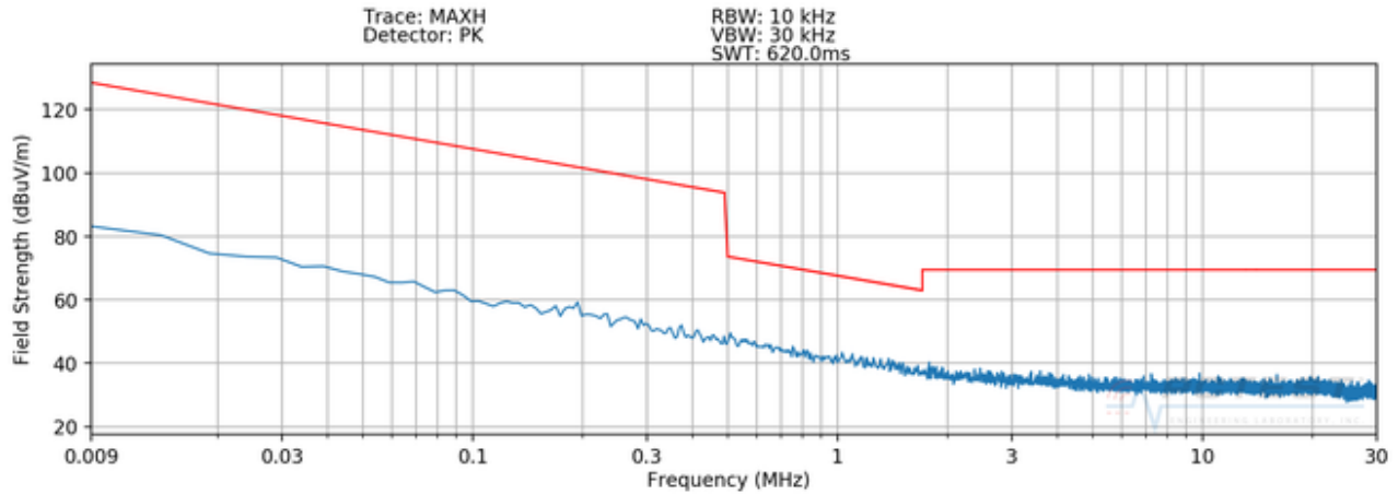
Plot 7-1. Radiated Spurious Plot 9kHz – 30MHz (Pol. X – WPT – Digitizer Hover)
