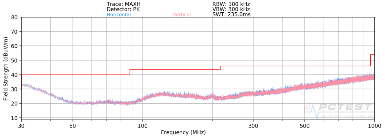
Plot 7-45. Radiated Spurious Plot below 1GHz
