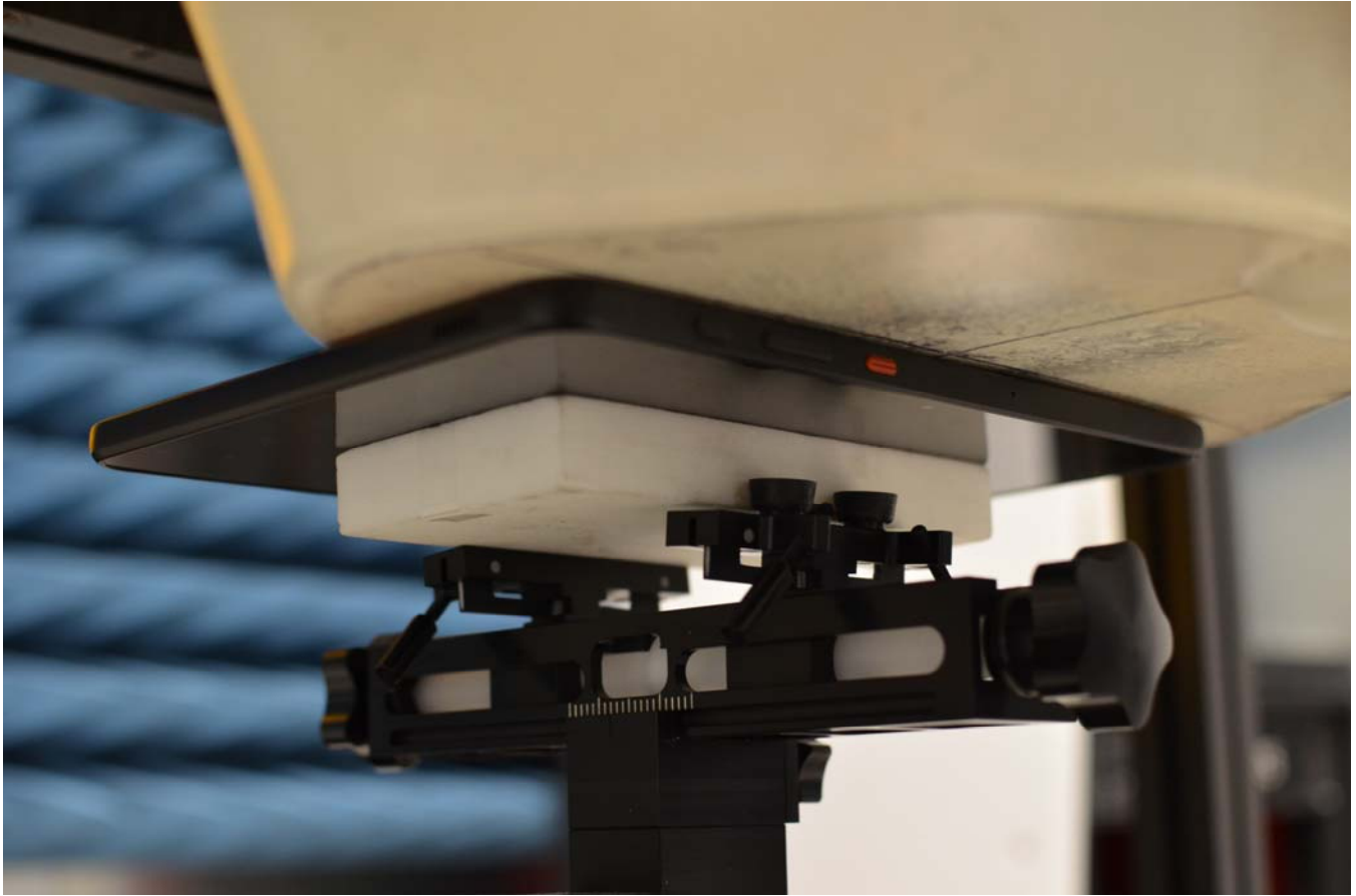
SAR Test Setup Photo 3 – Back Side at 0 cm
