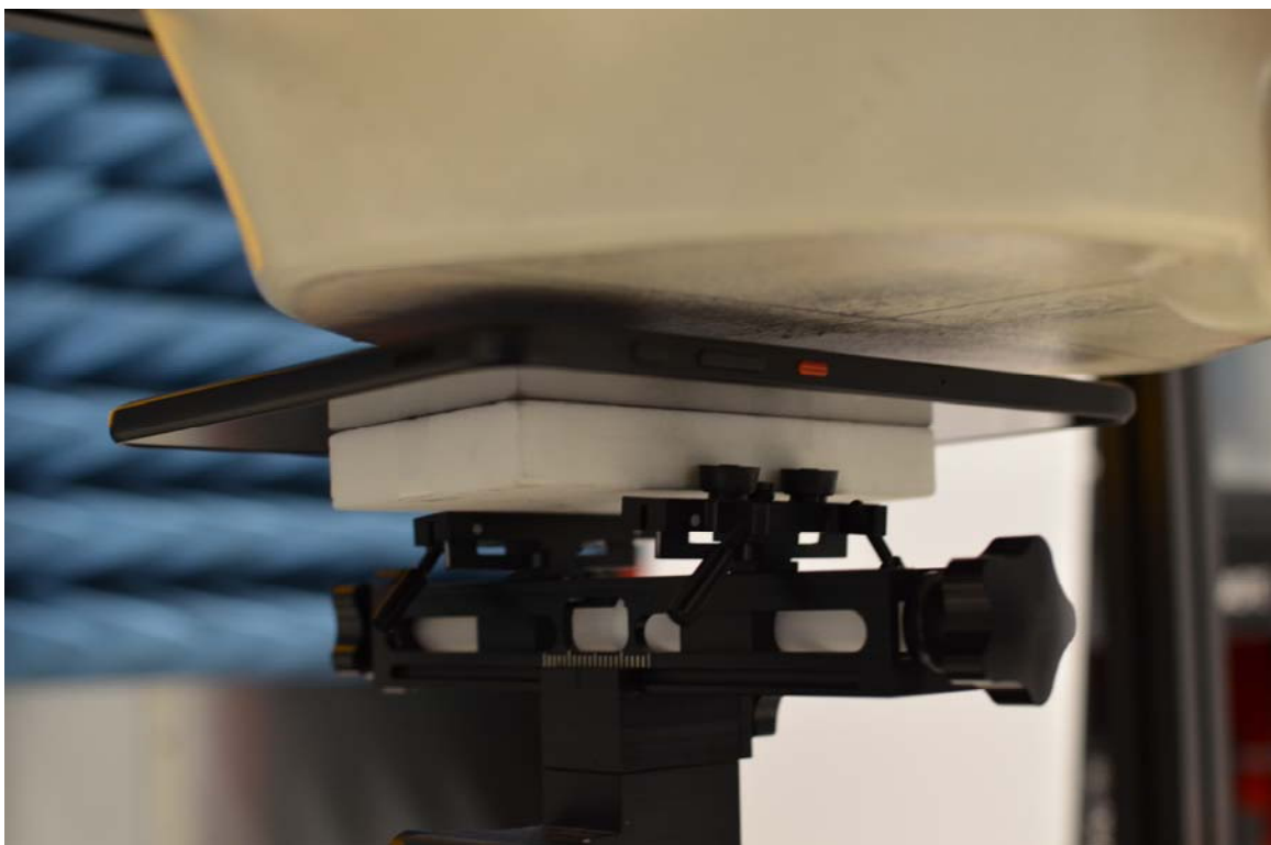
SAR Test Setup Photo 2 – Backside at 0.8 cm
