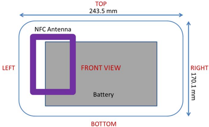
Figure F-2 NFC Antenna Locations
