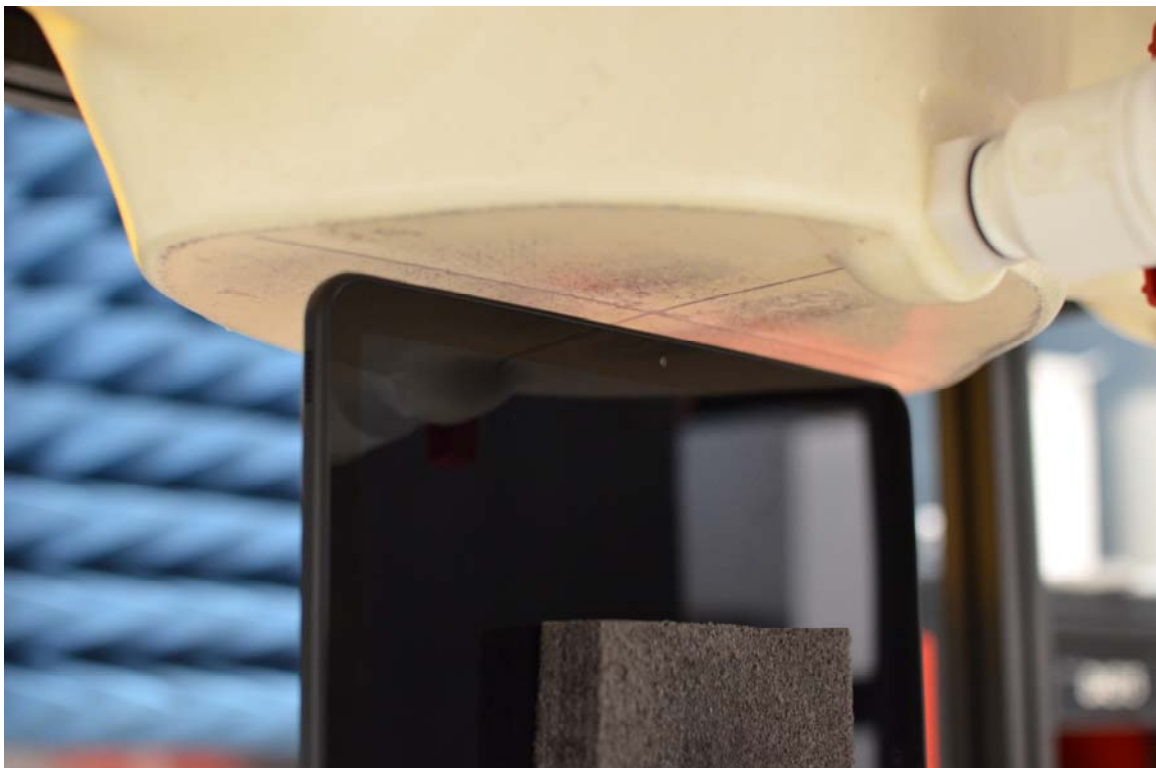
SAR Test Setup Photo 5 – Top Edge at 0.6 cm
