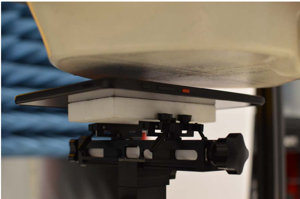
SAR Test Setup Photo 1 – Back Side at 1.5 cm
