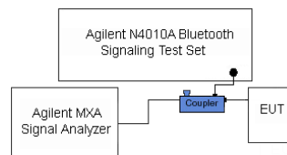
Figure 7-2 Power Measurement Setup
