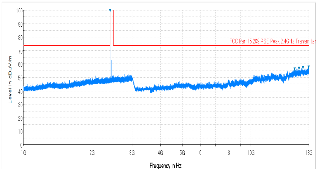
Plot 6-43. Radiated Spurious Plot above 1GHz (BT – Ch. 0, Ant. Pol. V)
