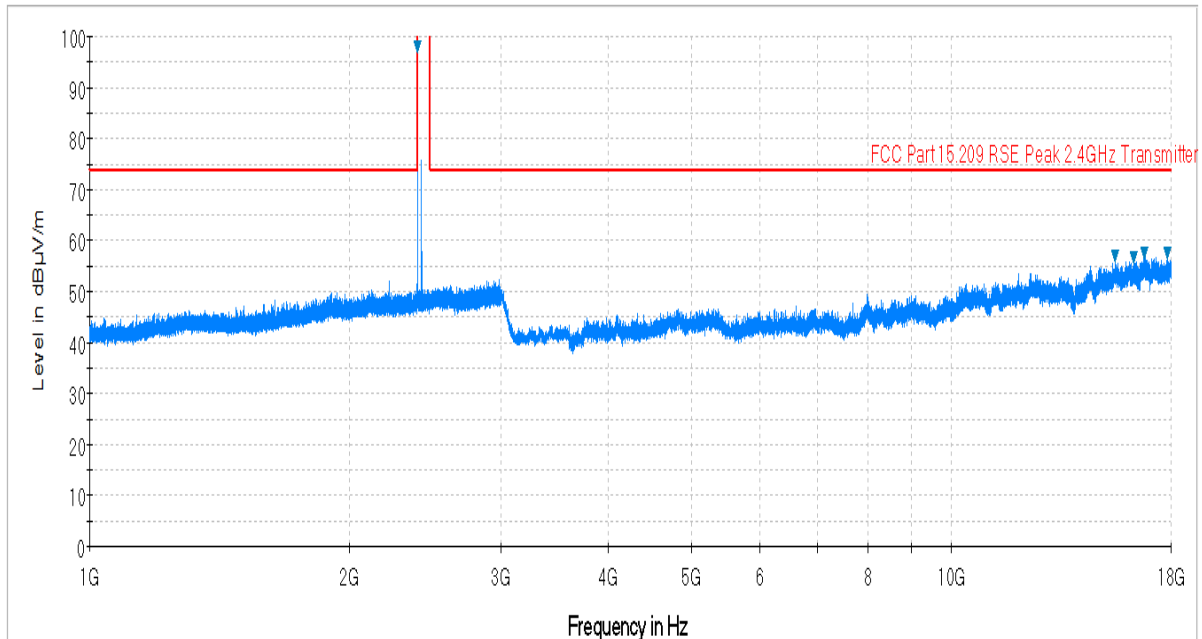
Plot 6-42. Radiated Spurious Plot above 1GHz (BT – Ch. 0, Ant. Pol. H)
