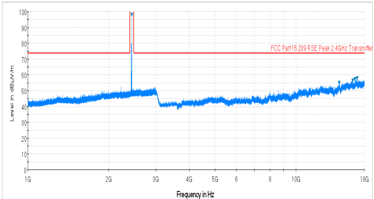
Plot 6-45. Radiated Spurious Plot above 1GHz (BT – Ch. 39, Ant. Pol. V)
