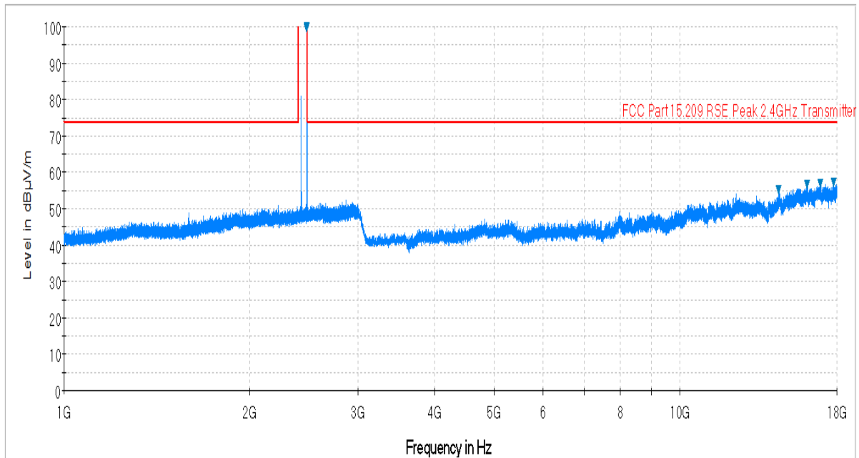
Plot 6-47. Radiated Spurious Plot above 1GHz (BT – Ch. 78, Ant. Pol. V)
