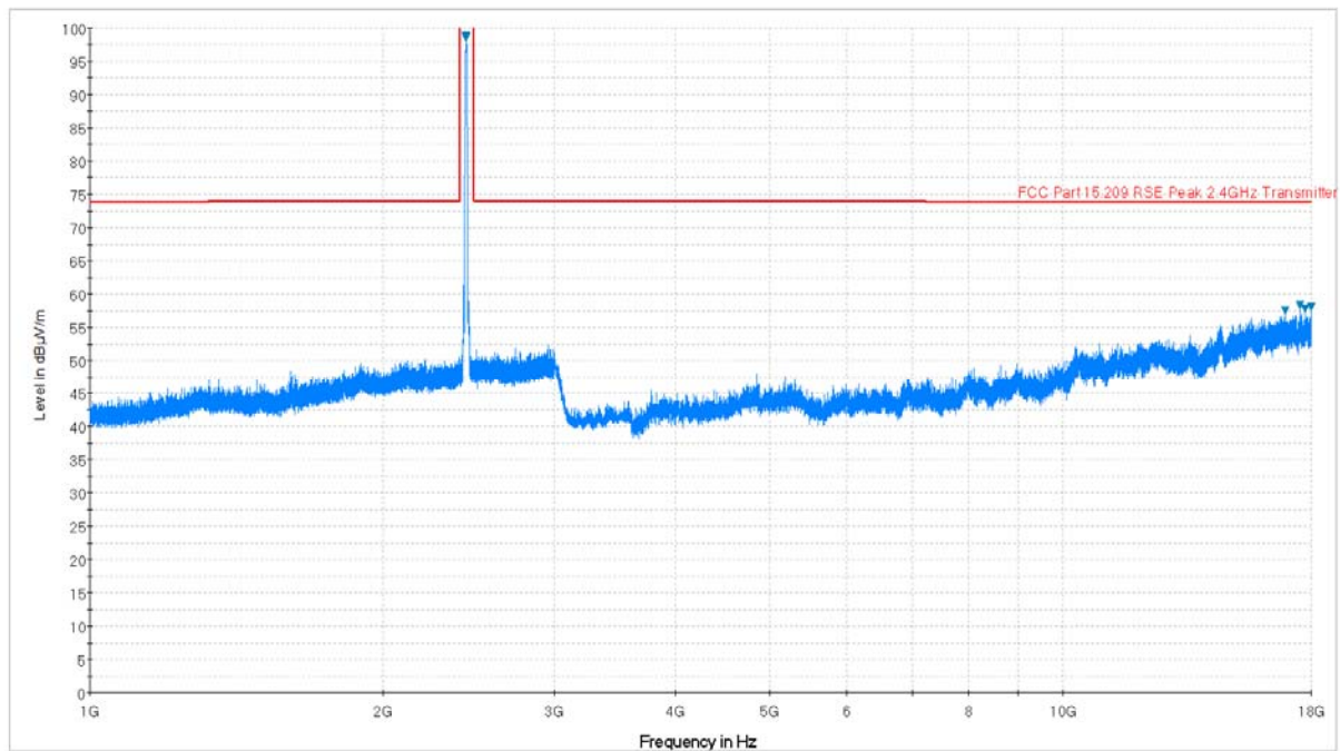
Plot 6-33. Radiated Spurious Plot above 1GHz (802.11b – Ch. 6, Ant. Pol. H)
