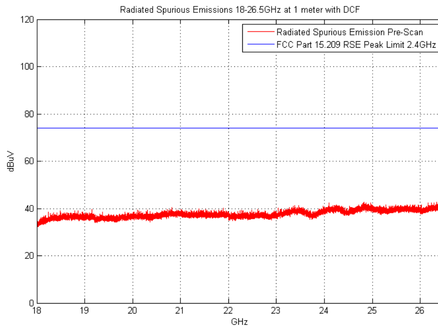
Plot 6-38. Radiated Spurious Plot above 18GHz (Pol. V)
