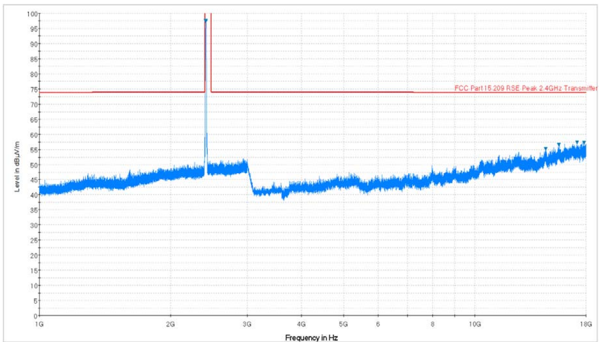
Plot 6-32. Radiated Spurious Plot above 1GHz (802.11b – Ch. 1, Ant. Pol. V)
