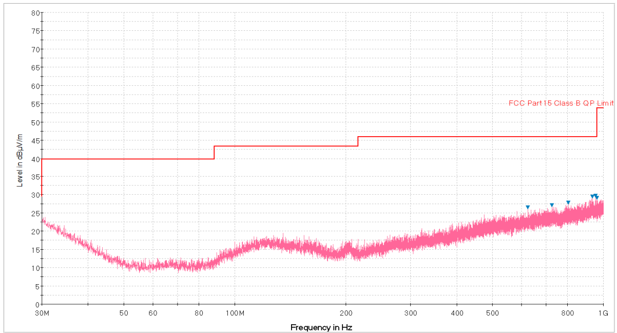
Plot 6-44. Radiated Spurious Plot below 1GHz (Pol. V)
