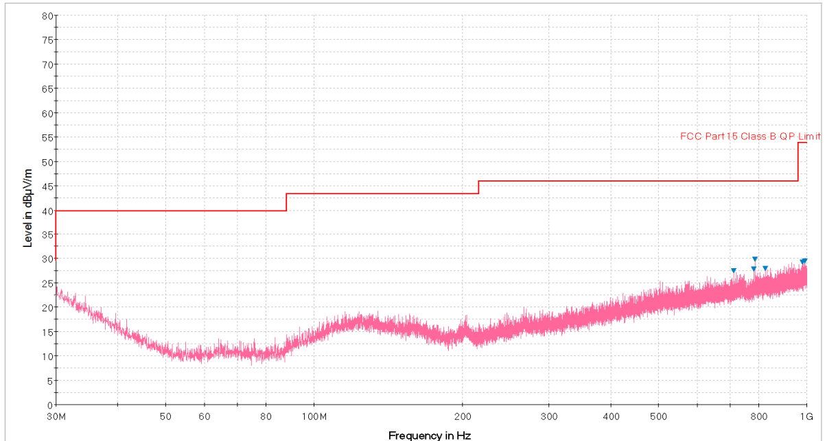
Plot 6-43. Radiated Spurious Plot below 1GHz (Pol. H)
