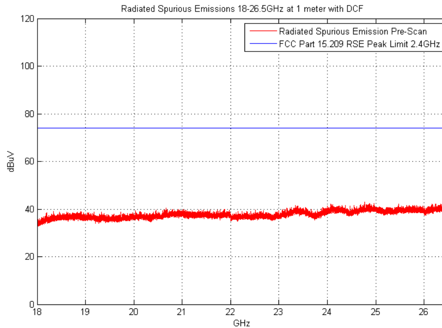
Plot 6-37. Radiated Spurious Plot above 18GHz (Pol. H)
