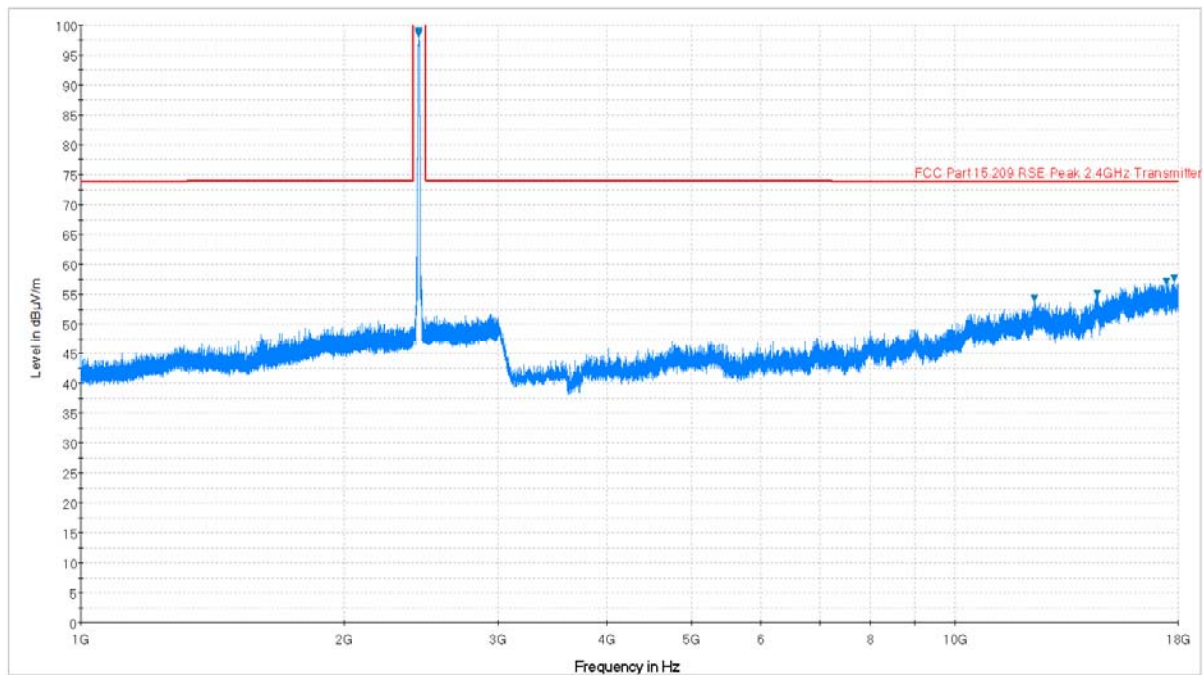
Plot 6-34. Radiated Spurious Plot above 1GHz (802.11b – Ch. 6, Ant. Pol. V)
