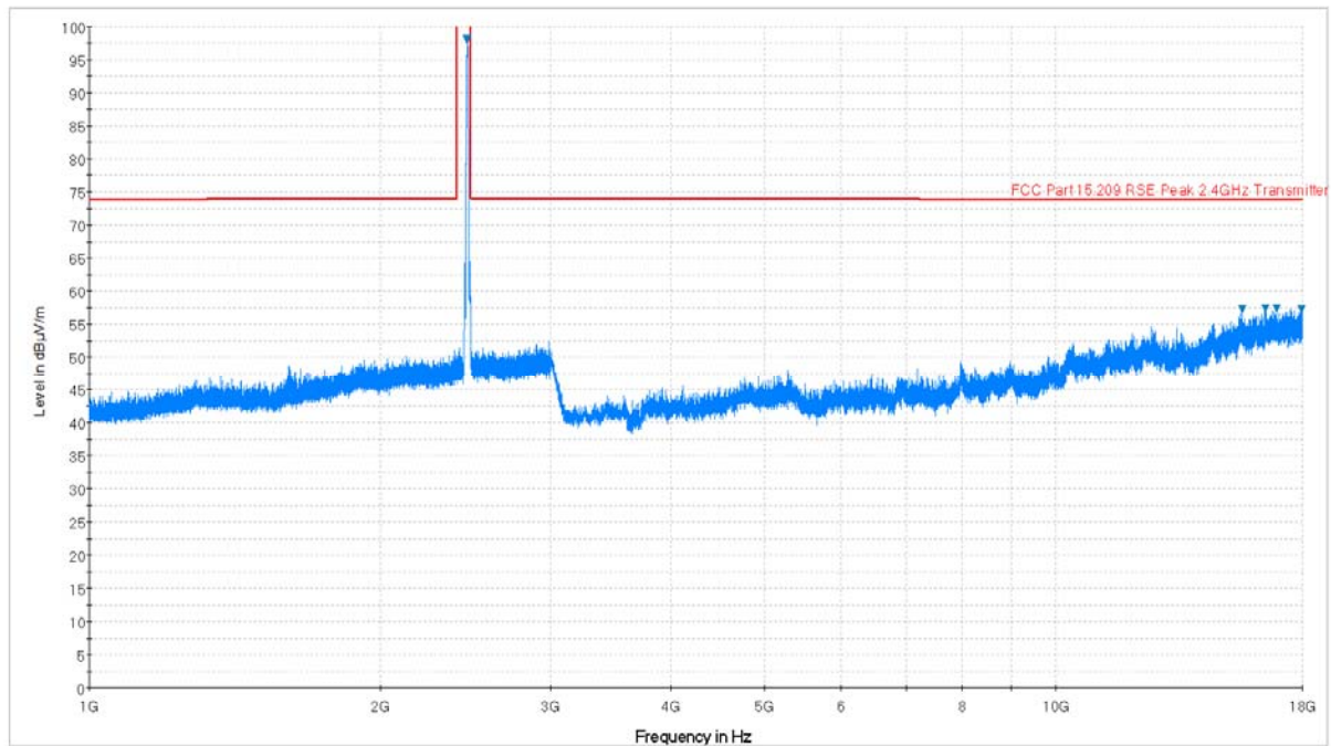
Plot 6-36. Radiated Spurious Plot above 1GHz (802.11b – Ch. 11, Ant. Pol. V)
