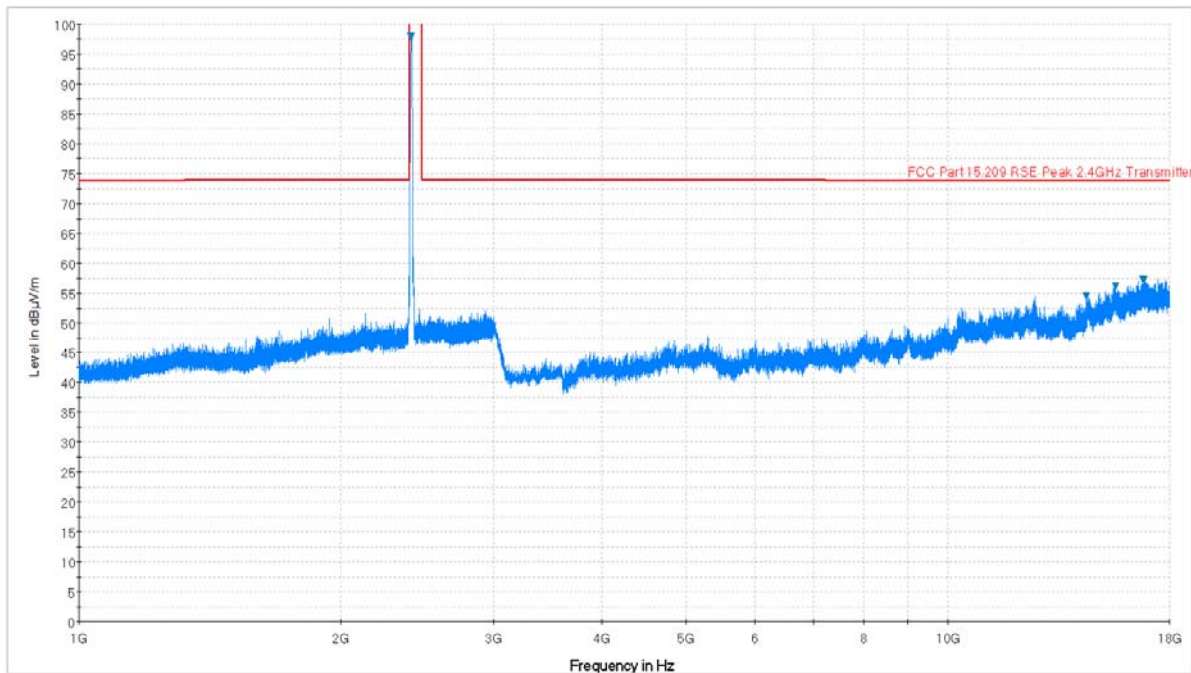
Plot 6-31. Radiated Spurious Plot above 1GHz (802.11b – Ch. 1, Ant. Pol. H)
