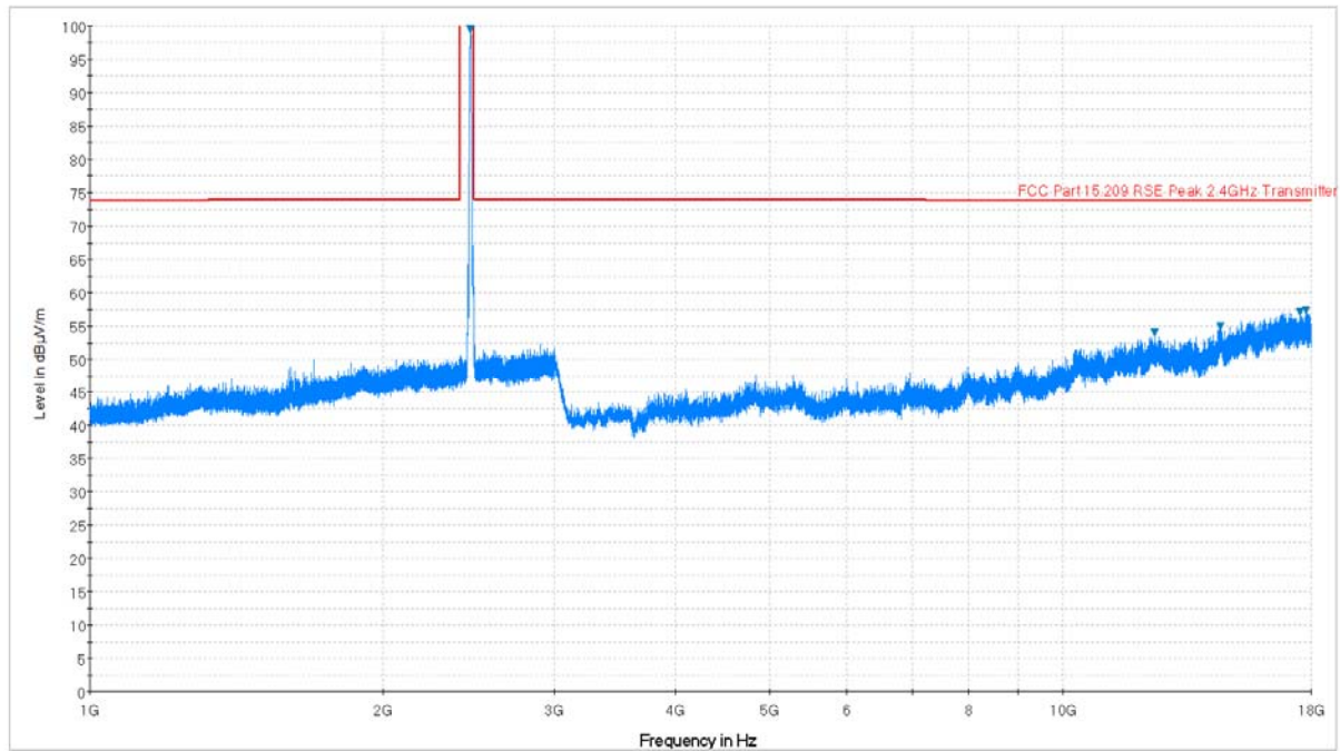
Plot 6-35. Radiated Spurious Plot above 1GHz (802.11b – Ch. 11, Ant. Pol. H)
