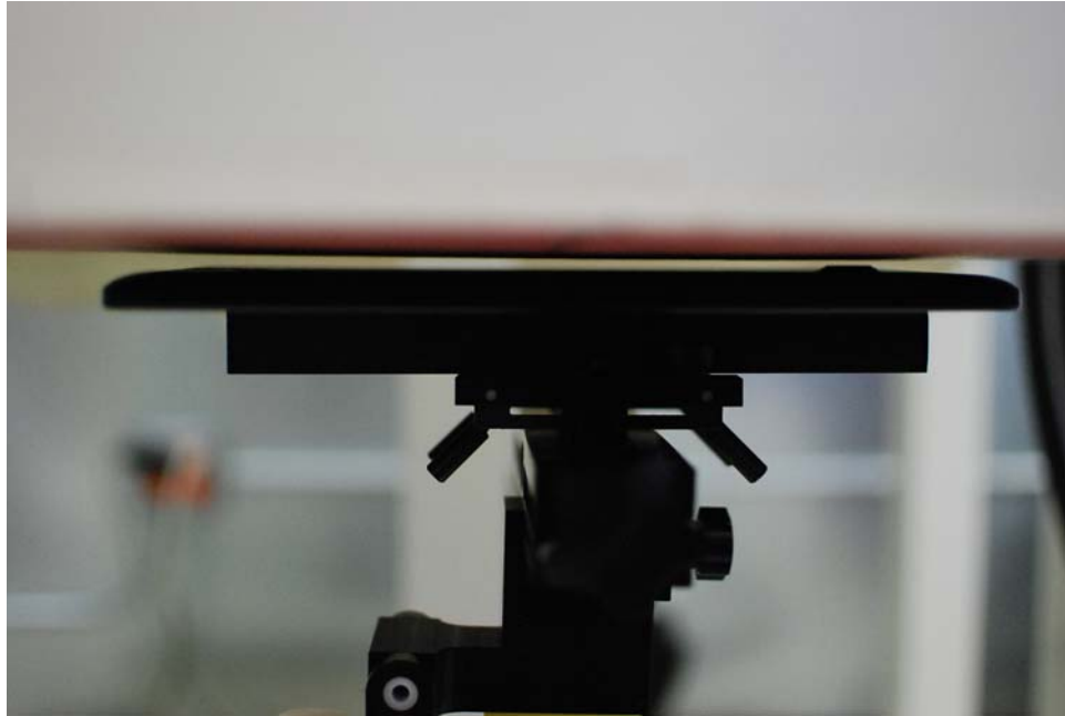
SAR Test Setup Photo 1: Back Side at 0.3 cm
