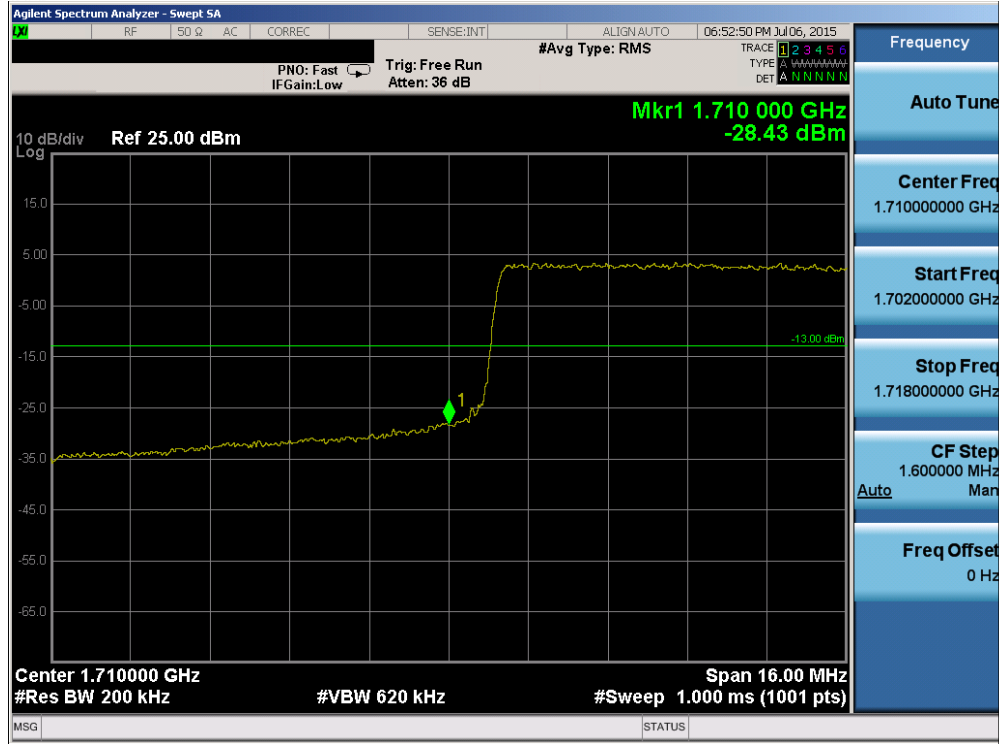
Plot 6-84. Lower Band Edge Plot (Band 4 – 20.0MHz QPSK – RB Size 100)
