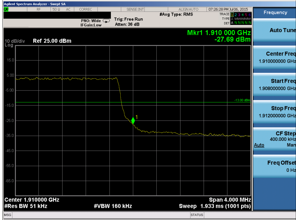
Plot 6-98. Upper Band Edge Plot (Band 2 – 5.0MHz QPSK – RB Size 25)
