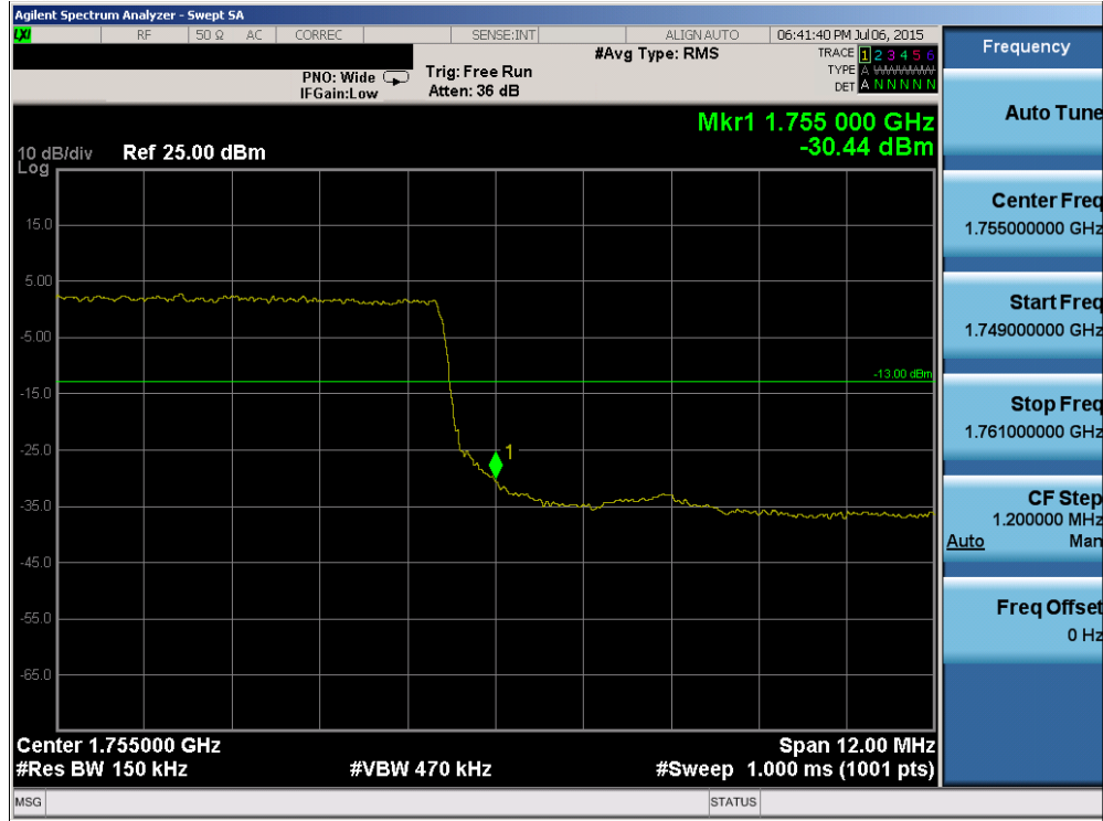
Plot 6-82. Upper Band Edge Plot (Band 4 – 15.0MHz QPSK – RB Size 75)
