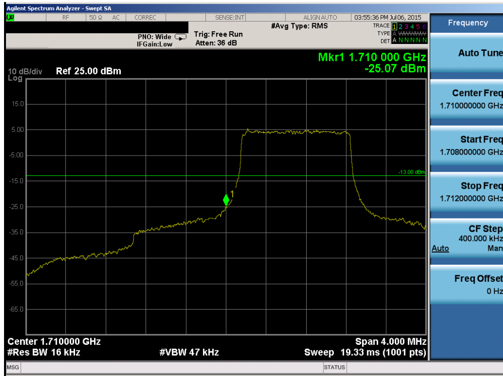
Plot 6-64. Lower Band Edge Plot (Band 4 – 1.4MHz QPSK – RB Size 6)
