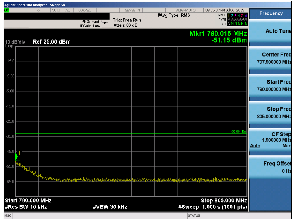
Plot 6-63. Upper Emission Mask Edge Plot (Band 13 – 10.0MHz QPSK – RB Size 50)
