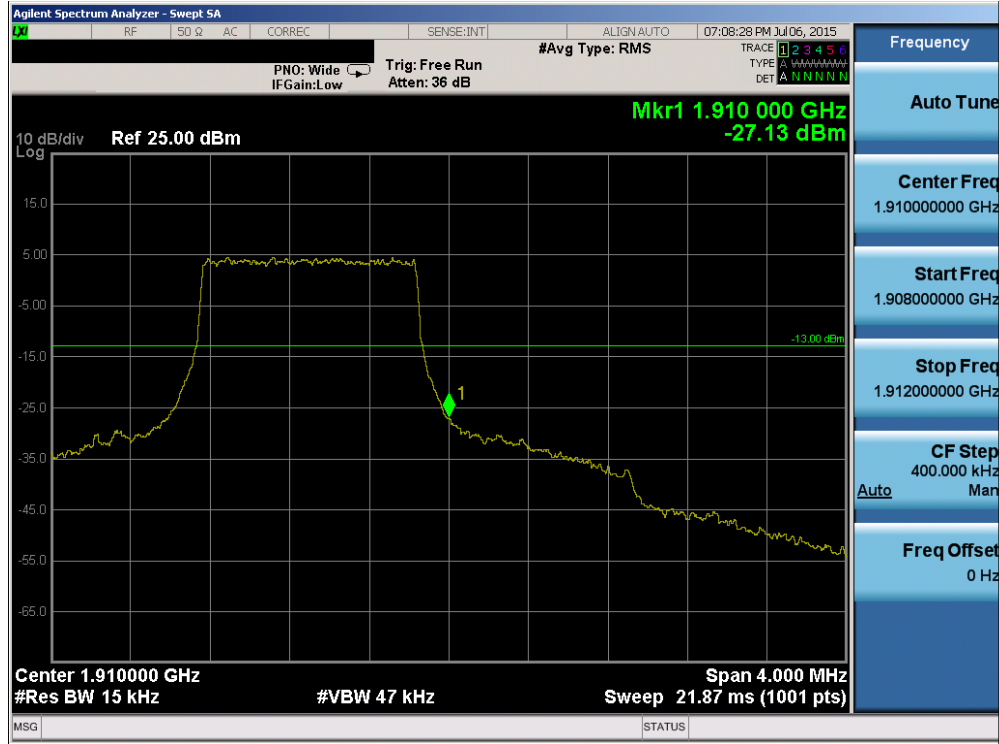
Plot 6-90. Upper Band Edge Plot (Band 2 – 1.4MHz QPSK – RB Size 6)
