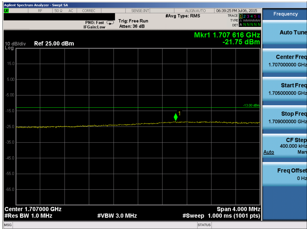
Plot 6-81. Lower Extended Band Edge Plot (Band 4 – 15.0MHz QPSK – RB Size 75)
