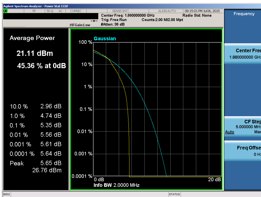
Plot 6-113. PAR Plot (Band 2 – 1.4MHz 16-QAM – RB Size 6)
