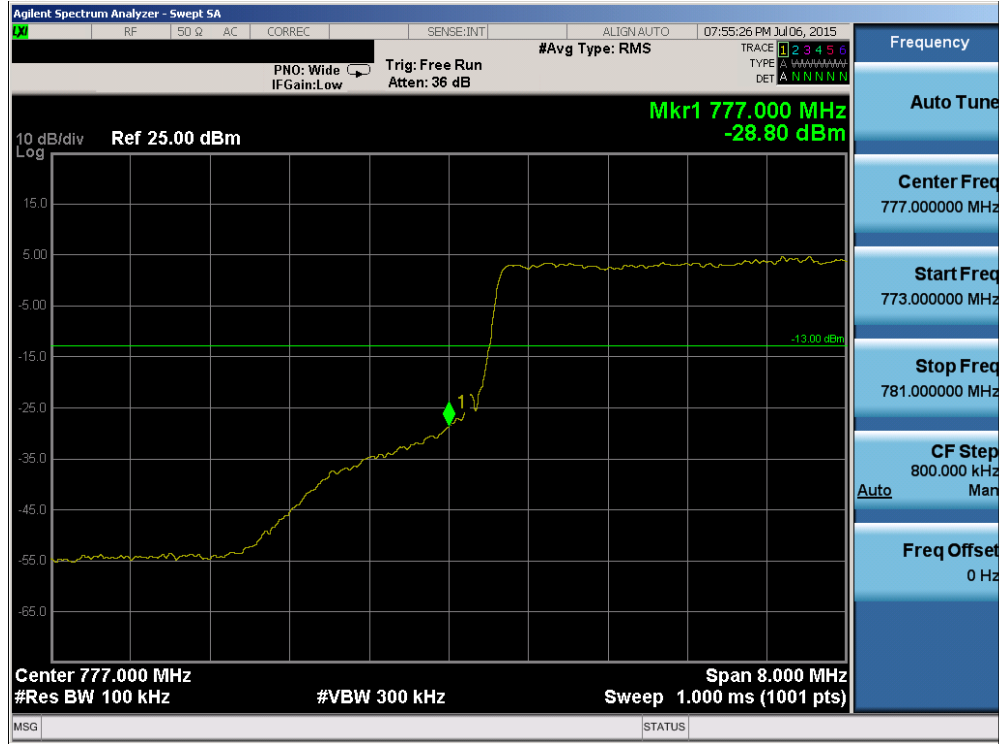
Plot 6-60. Lower Band Edge Plot (Band 13 – 10.0MHz QPSK – RB Size 50)
