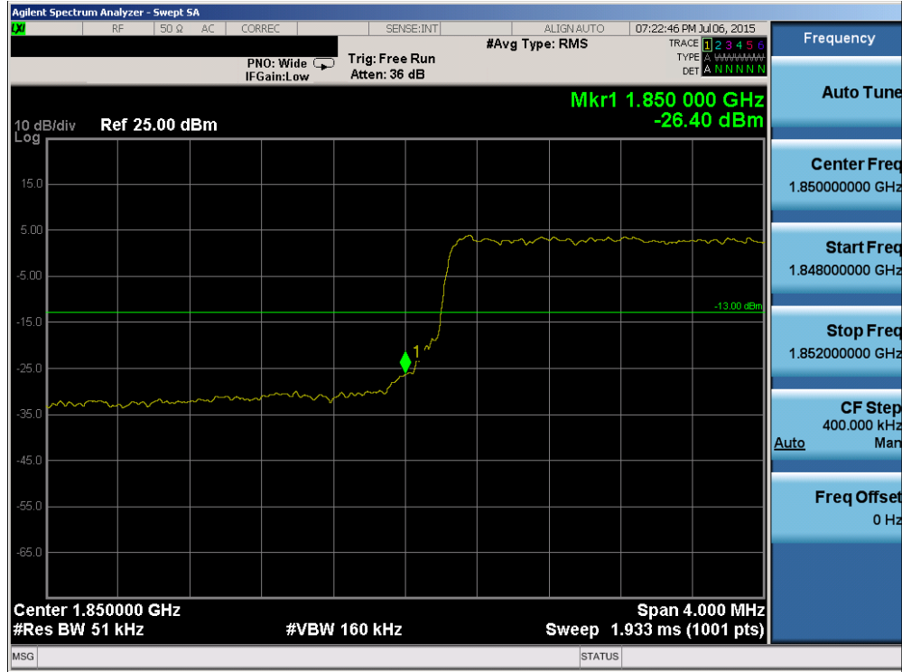
Plot 6-96. Lower Band Edge Plot (Band 2 – 5.0MHz QPSK – RB Size 25)
