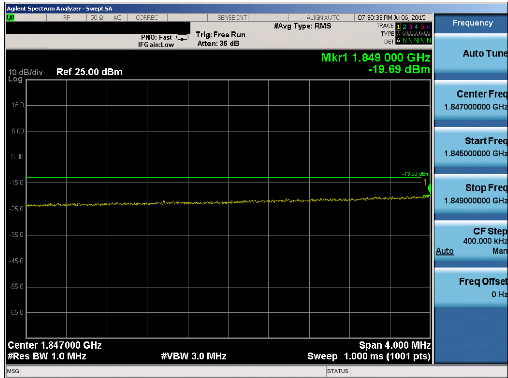
Plot 6-101. Lower Extended Band Edge Plot (Band 2 – 10.0MHz QPSK – RB Size 50)
