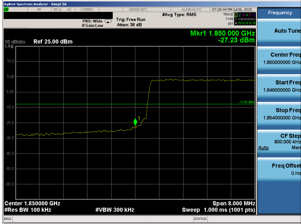
Plot 6-100. Lower Band Edge Plot (Band 2 – 10.0MHz QPSK – RB Size 50)
