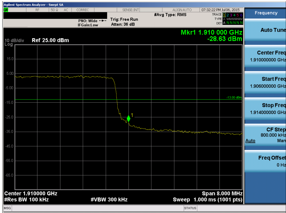
Plot 6-102. Upper Band Edge Plot (Band 2 – 10.0MHz QPSK – RB Size 50)
