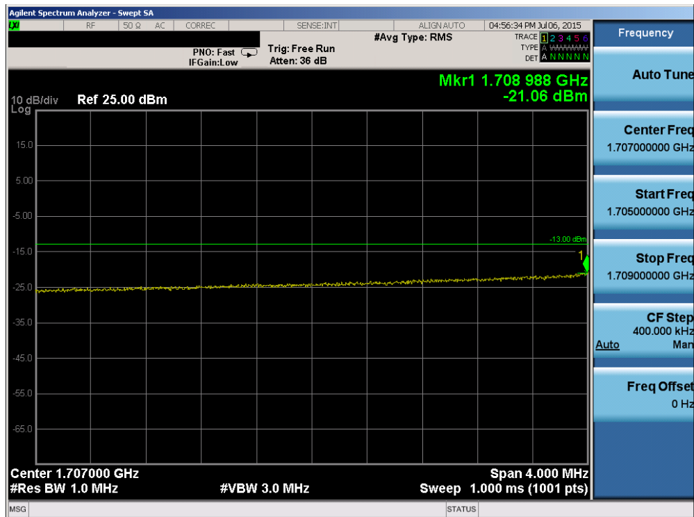
Plot 6-77. Lower Extended Band Edge Plot (Band 4 – 10.0MHz QPSK – RB Size 50)
