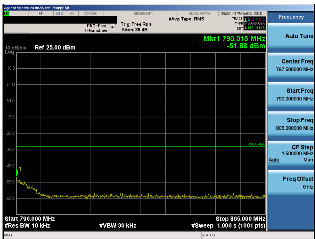
Plot 6-59. Upper Emission Mask Edge Plot (Band 13 - 5.0MHz QPSK - RB Size 25)
