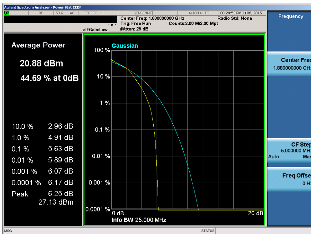
Plot 6-121. PAR Plot (Band 2 – 15.0MHz 16-QAM – RB Size 75)
