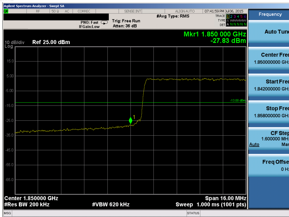
Plot 6-108. Lower Band Edge Plot (Band 2 – 20.0MHz QPSK – RB Size 100)
