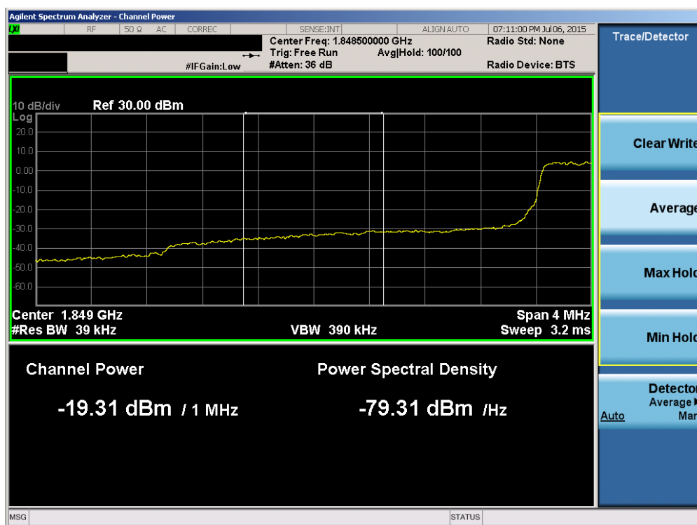
Plot 6-93. Lower Extended Band Edge Plot (Band 2 – 3.0MHz QPSK – RB Size 15)
