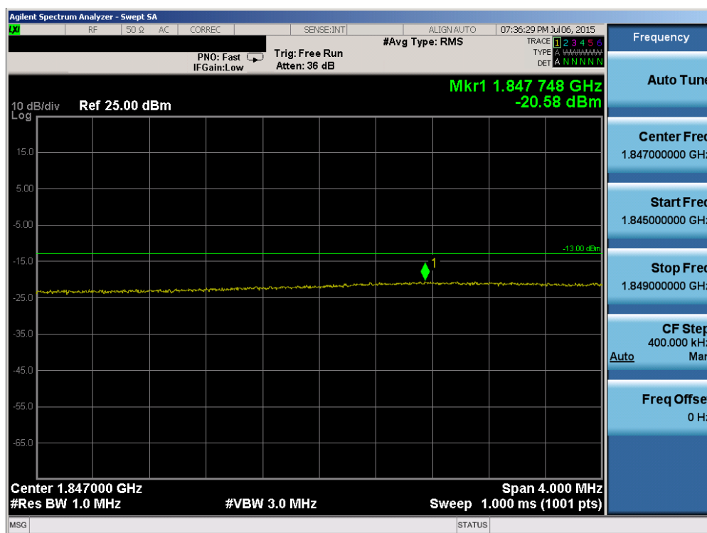
Plot 6-105. Lower Extended Band Edge Plot (Band 2 – 15.0MHz QPSK – RB Size 75)
