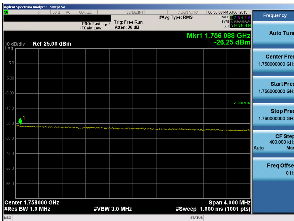
Plot 6-87. Upper Extended Band Edge Plot (Band 4 - 20.0MHz QPSK - RB Size 100)
