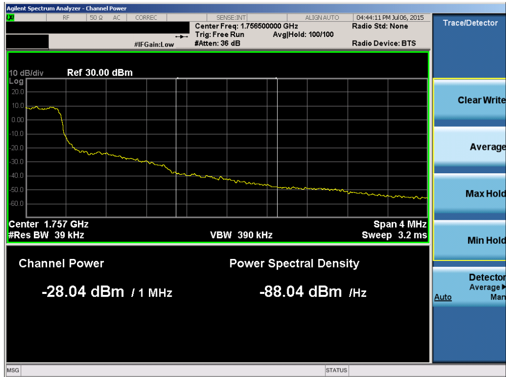
Plot 6-67. Upper Extended Band Edge Plot (Band 4 – 1.4MHz QPSK – RB Size 6)
