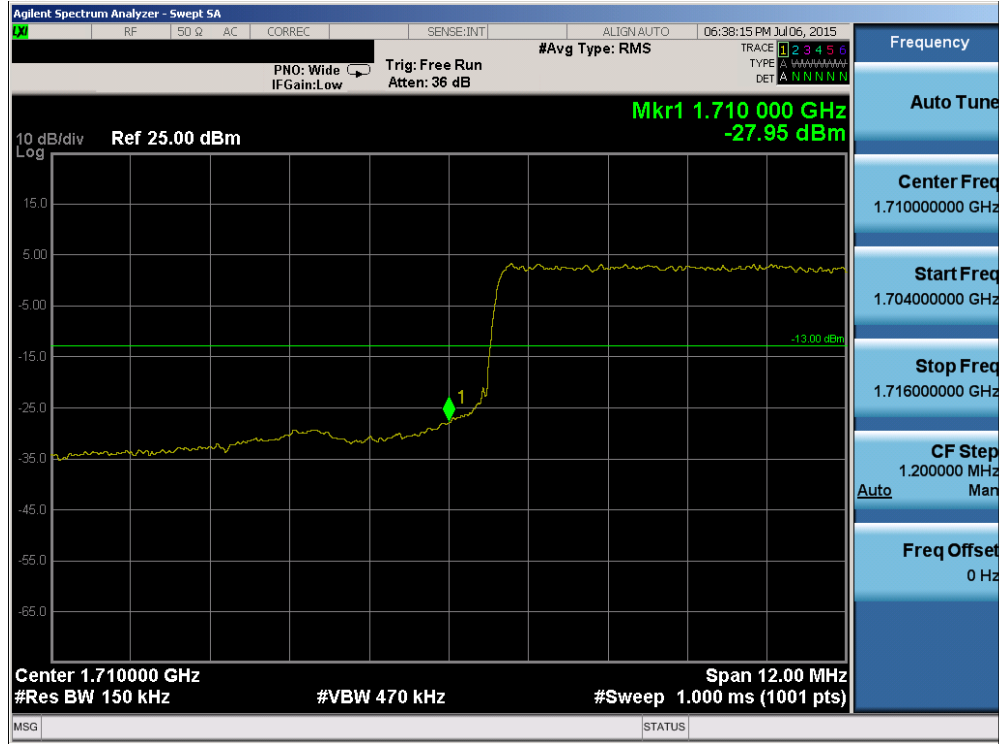
Plot 6-80. Lower Band Edge Plot (Band 4 – 15.0MHz QPSK – RB Size 75)
