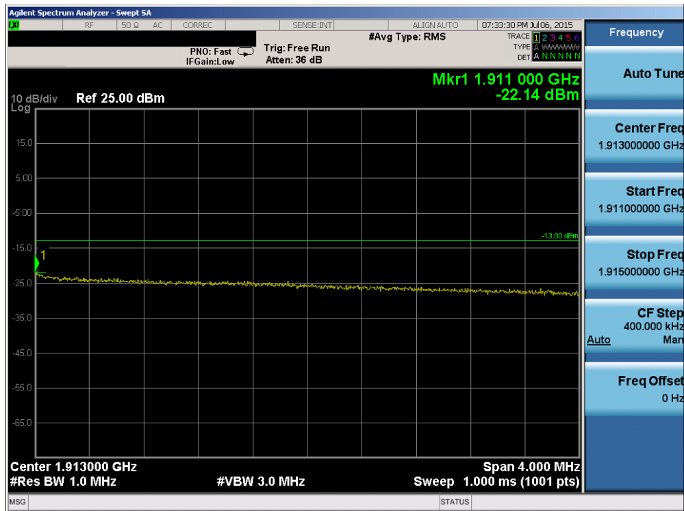
Plot 6-103. Upper Extended Band Edge Plot (Band 2 – 10.0MHz QPSK – RB Size 50)
