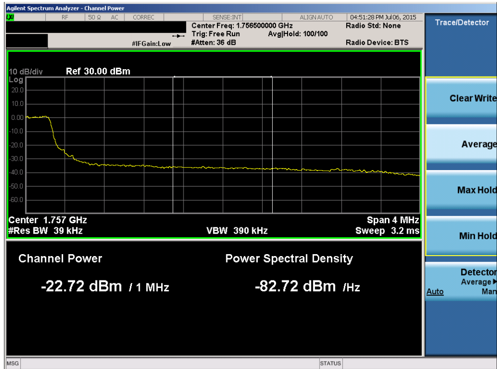
Plot 6-75. Upper Extended Band Edge Plot (Band 4 – 5.0MHz QPSK – RB Size 25)
