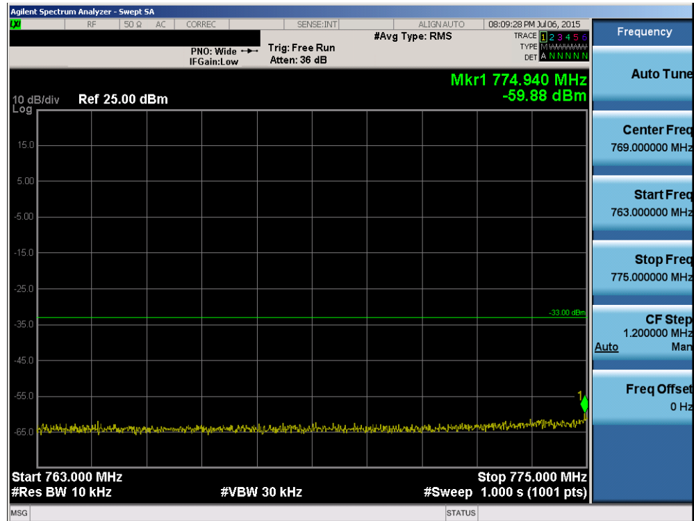
Plot 6-61. Lower Emission Mask Edge Plot (Band 13 – 10.0MHz QPSK – RB Size 50)
