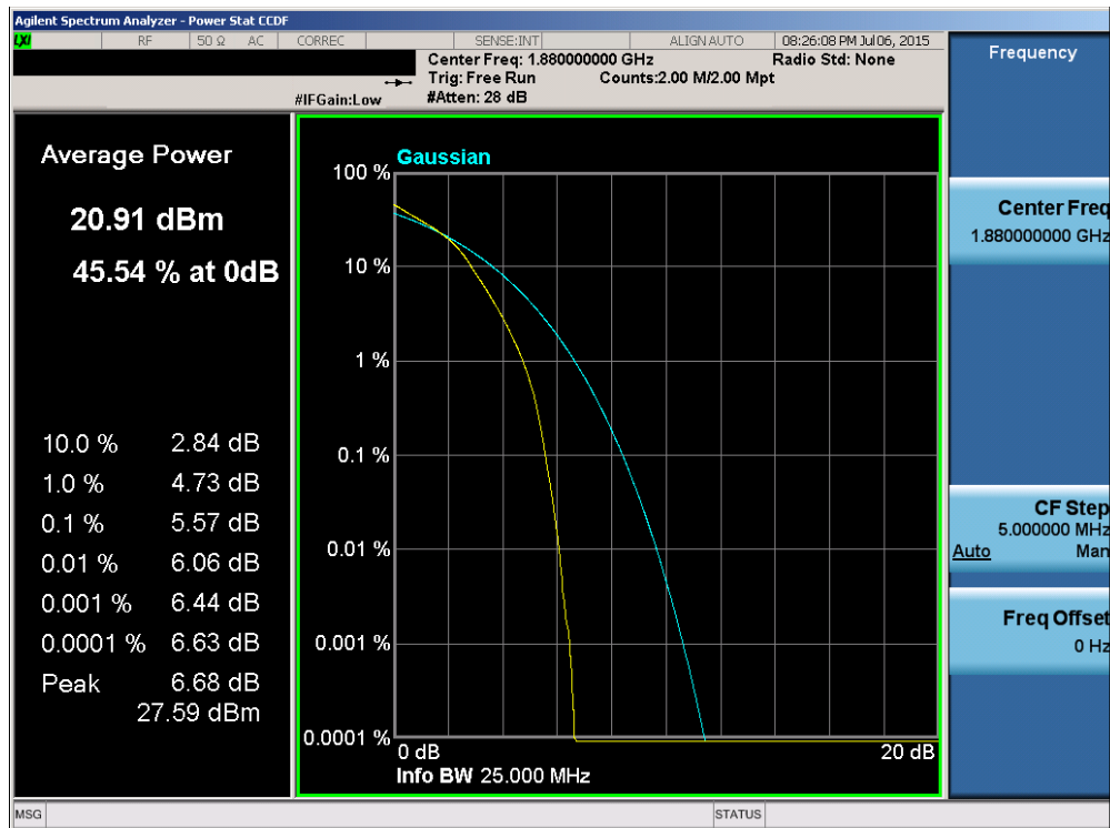
Plot 6-123. PAR Plot (Band 2 – 20.0MHz 16-QAM – RB Size 100)
