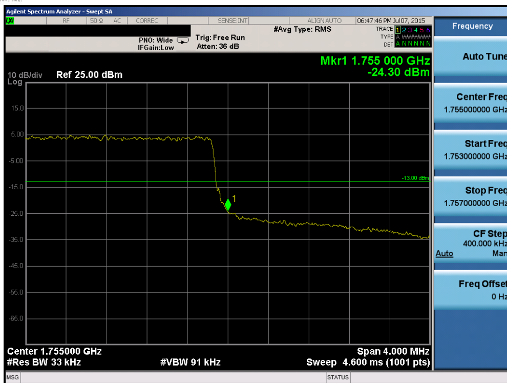
Plot 6-70. Upper Band Edge Plot (Band 4 – 3.0MHz QPSK – RB Size 15)
