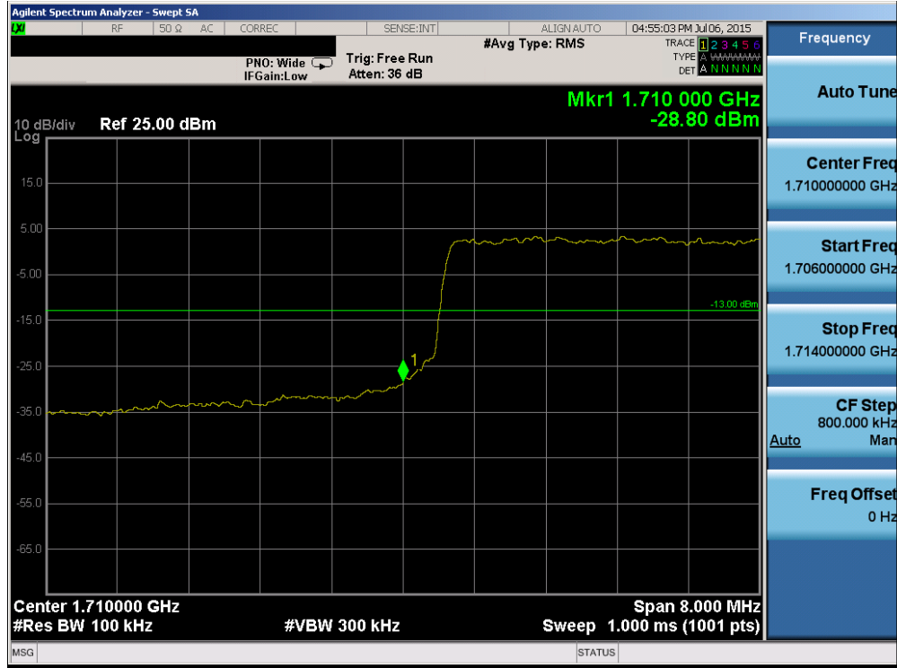
Plot 6-76. Lower Band Edge Plot (Band 4 – 10.0MHz QPSK – RB Size 50)
