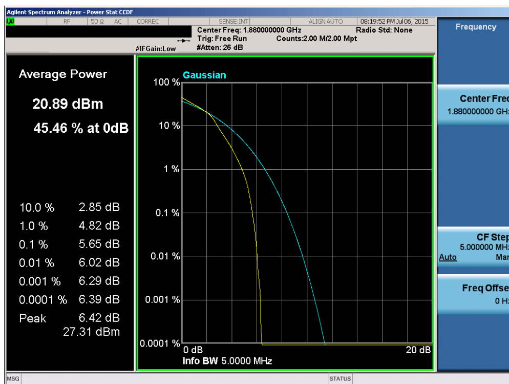
Plot 6-117. PAR Plot (Band 2 – 5.0MHz 16-QAM – RB Size 25)
