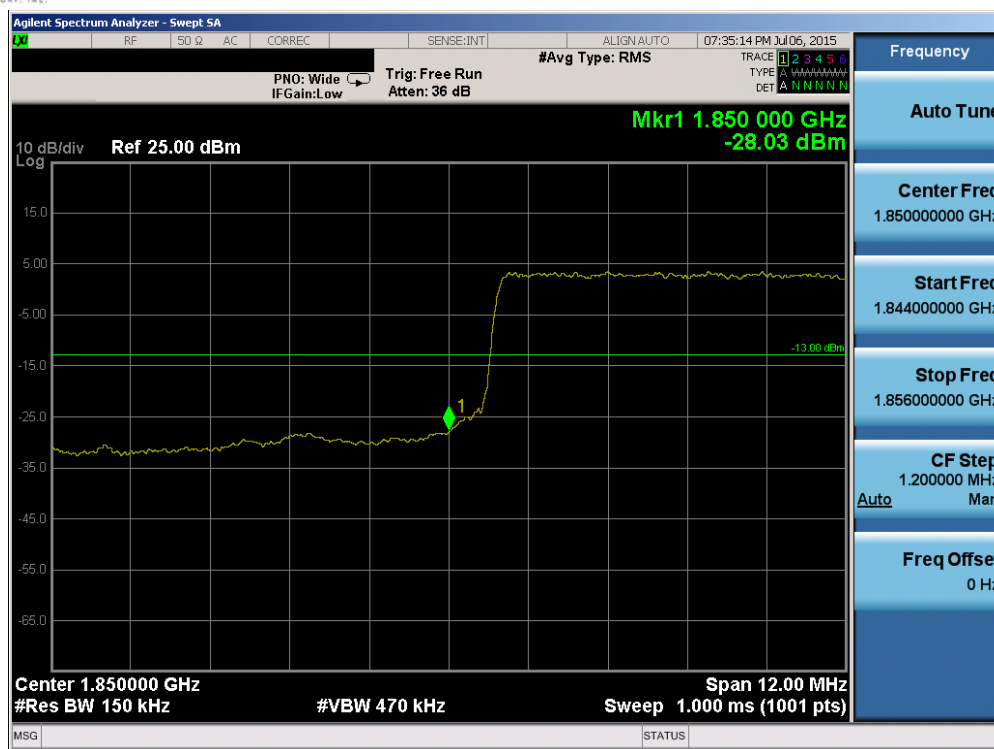
Plot 6-104. Lower Band Edge Plot (Band 2 – 15.0MHz QPSK – RB Size 75)
