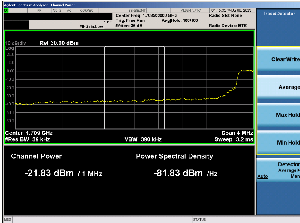
Plot 6-73. Lower Extended Band Edge Plot (Band 4 – 5.0MHz QPSK – RB Size 25)
