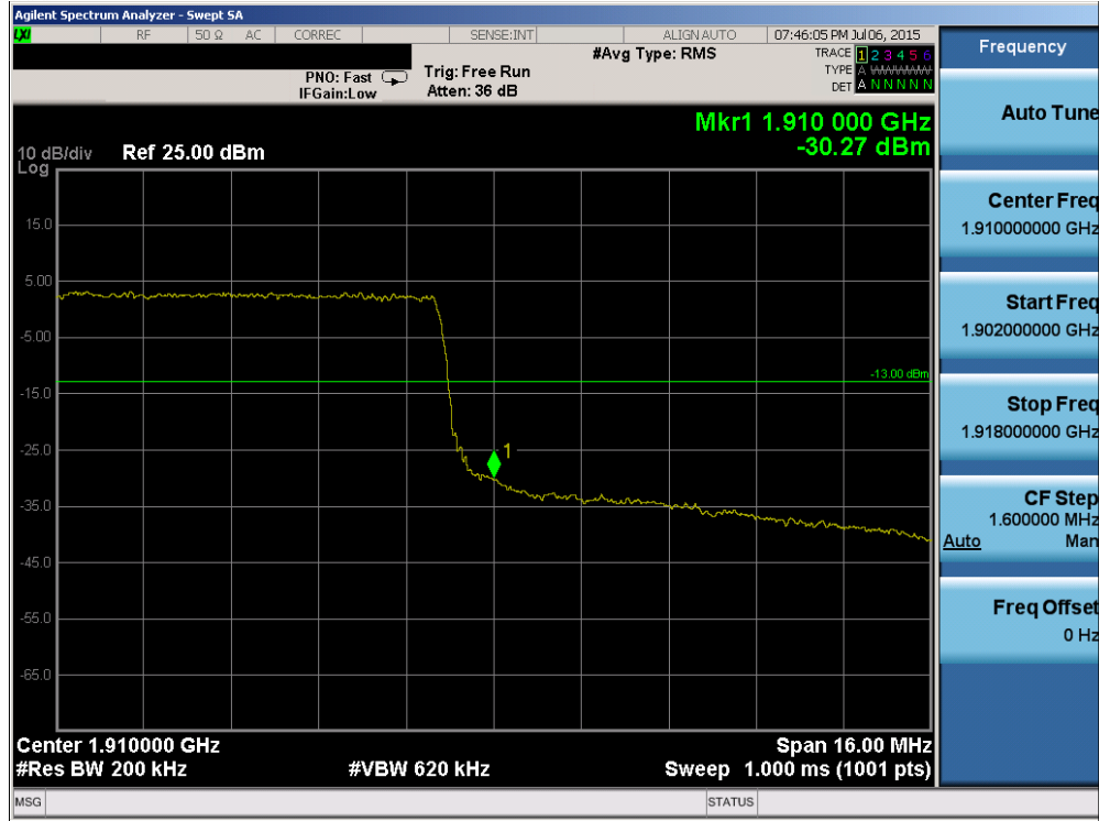
Plot 6-110. Upper Band Edge Plot (Band 2 - 20.0MHz QPSK - RB Size 100)
