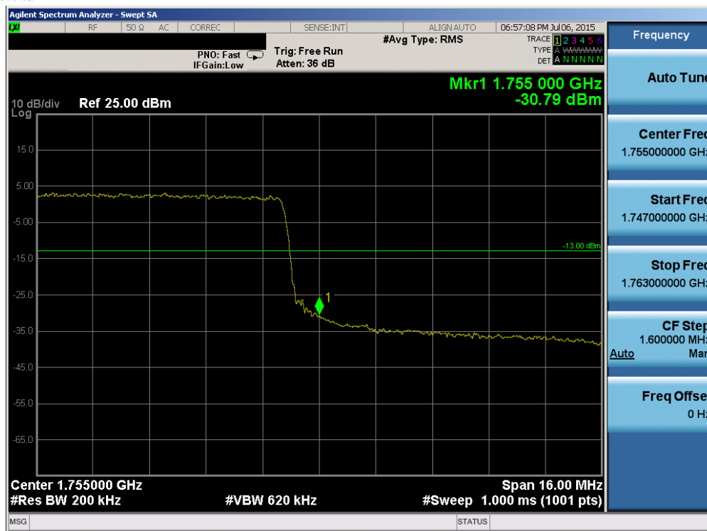
Plot 6-86. Upper Band Edge Plot (Band 4 - 20.0MHz QPSK - RB Size 100)
