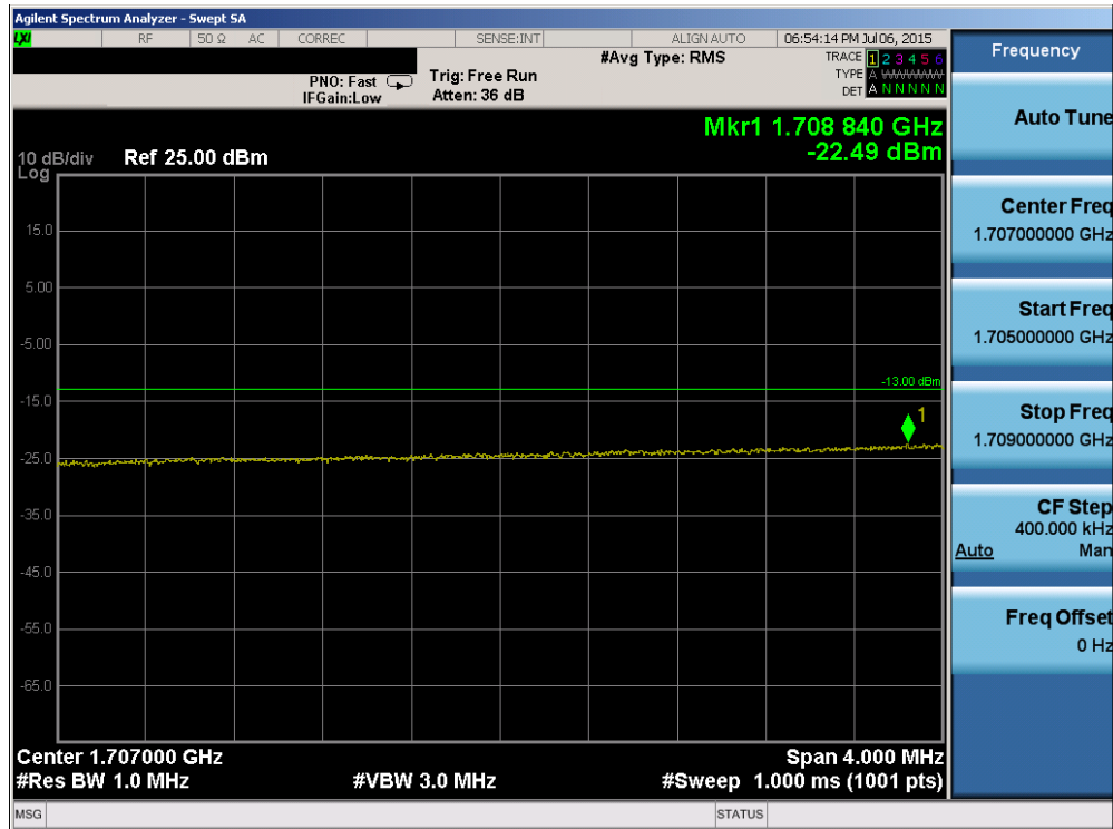
Plot 6-85. Lower Extended Band Edge Plot (Band 4 – 20.0MHz QPSK – RB Size 100)
