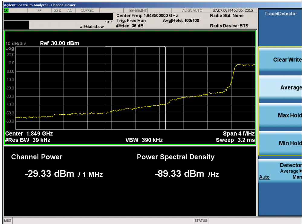
Plot 6-89. Lower Extended Band Edge Plot (Band 2 – 1.4MHz QPSK – RB Size 6)
