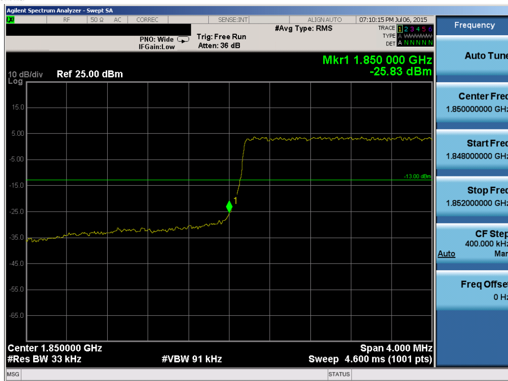
Plot 6-92. Lower Band Edge Plot (Band 2 – 3.0MHz QPSK – RB Size 15)
