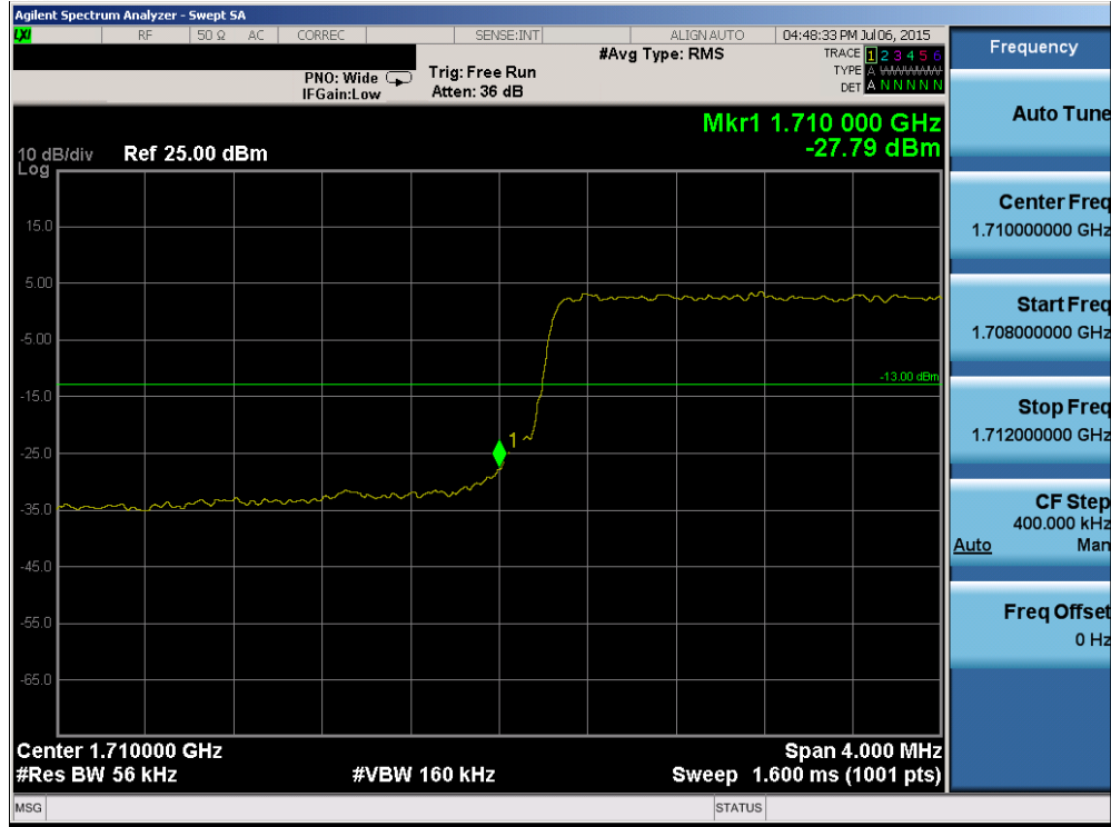
Plot 6-72. Lower Band Edge Plot (Band 4 – 5.0MHz QPSK – RB Size 25)
