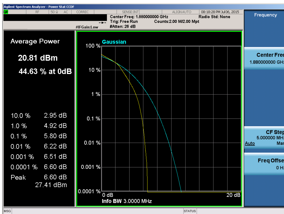
Plot 6-115. PAR Plot (Band 2 – 3.0MHz 16-QAM – RB Size 15)
