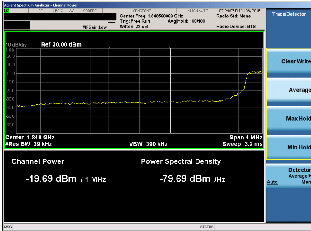
Plot 6-97. Lower Extended Band Edge Plot (Band 2 – 5.0MHz QPSK – RB Size 25)
