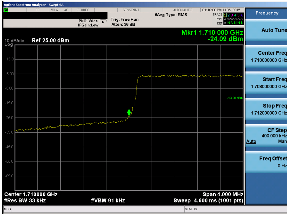
Plot 6-68. Lower Band Edge Plot (Band 4 – 3.0MHz QPSK – RB Size 15)
