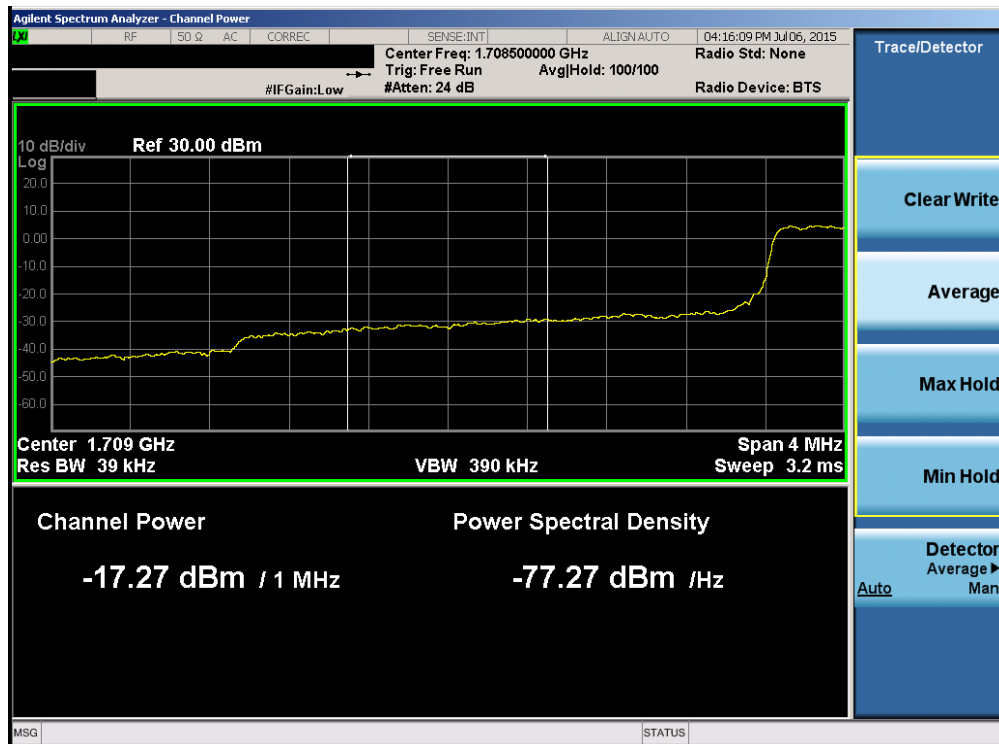
Plot 6-69. Lower Extended Band Edge Plot (Band 4 – 3.0MHz QPSK – RB Size 15)
