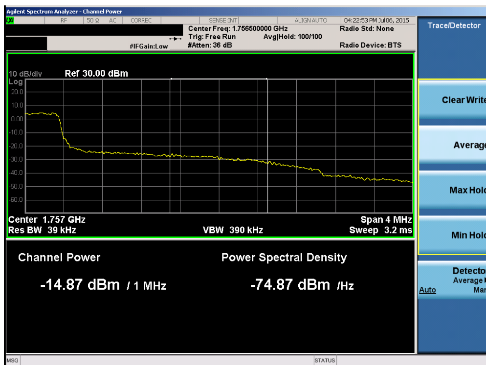
Plot 6-71. Upper Extended Band Edge Plot (Band 4 – 3.0MHz QPSK – RB Size 15)
