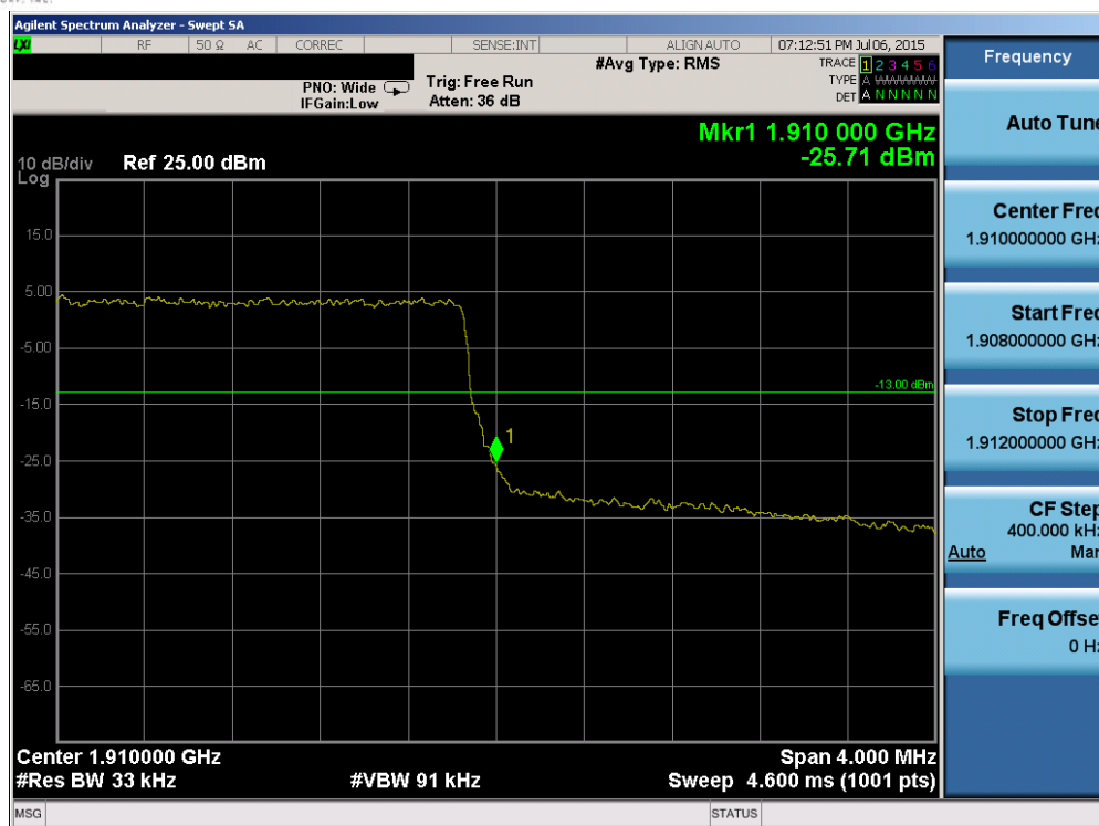
Plot 6-94. Upper Band Edge Plot (Band 2 – 3.0MHz QPSK – RB Size 15)
