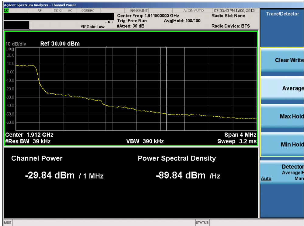
Plot 6-91. Upper Extended Band Edge Plot (Band 2 – 1.4MHz QPSK – RB Size 6)
