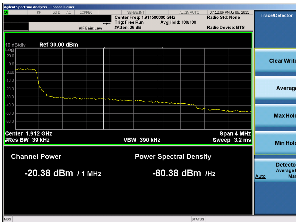
Plot 6-95. Upper Extended Band Edge Plot (Band 2 – 3.0MHz QPSK – RB Size 15)
