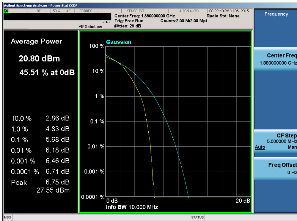
Plot 6-119. PAR Plot (Band 2 – 10.0MHz 16-QAM – RB Size 50)
