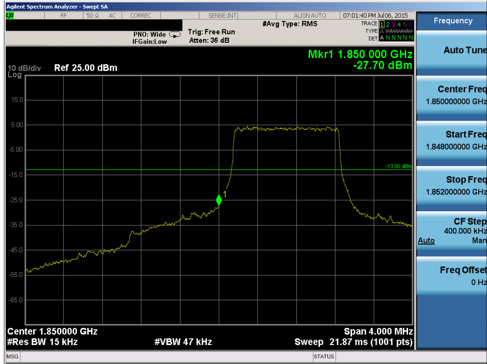
Plot 6-88. Lower Band Edge Plot (Band 2 – 1.4MHz QPSK – RB Size 6)
