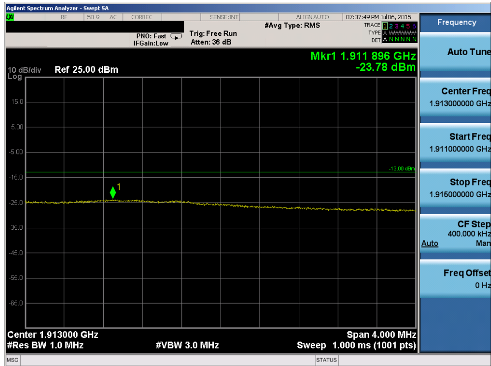
Plot 6-107. Upper Extended Band Edge Plot (Band 2 – 15.0MHz QPSK – RB Size 75)
