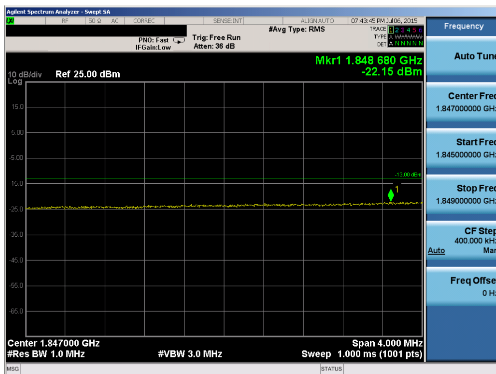
Plot 6-109. Lower Extended Band Edge Plot (Band 2 – 20.0MHz QPSK – RB Size 100)
