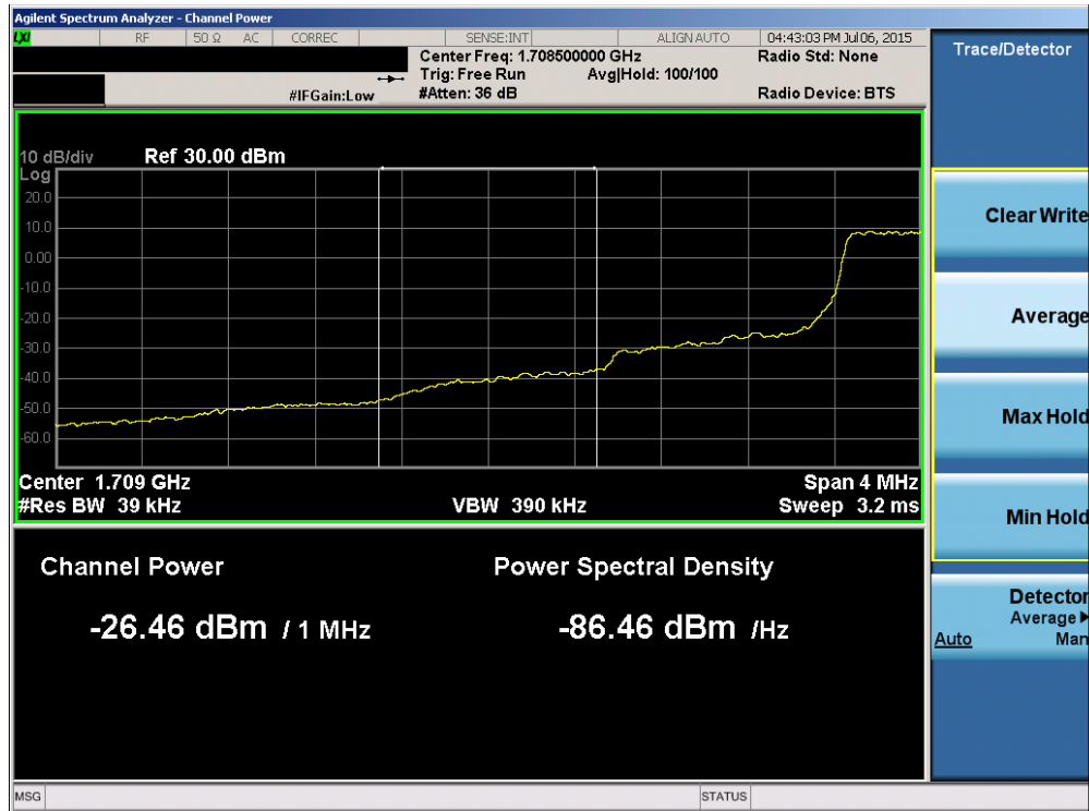
Plot 6-65. Lower Extended Band Edge Plot (Band 4 – 1.4MHz QPSK – RB Size 6)
