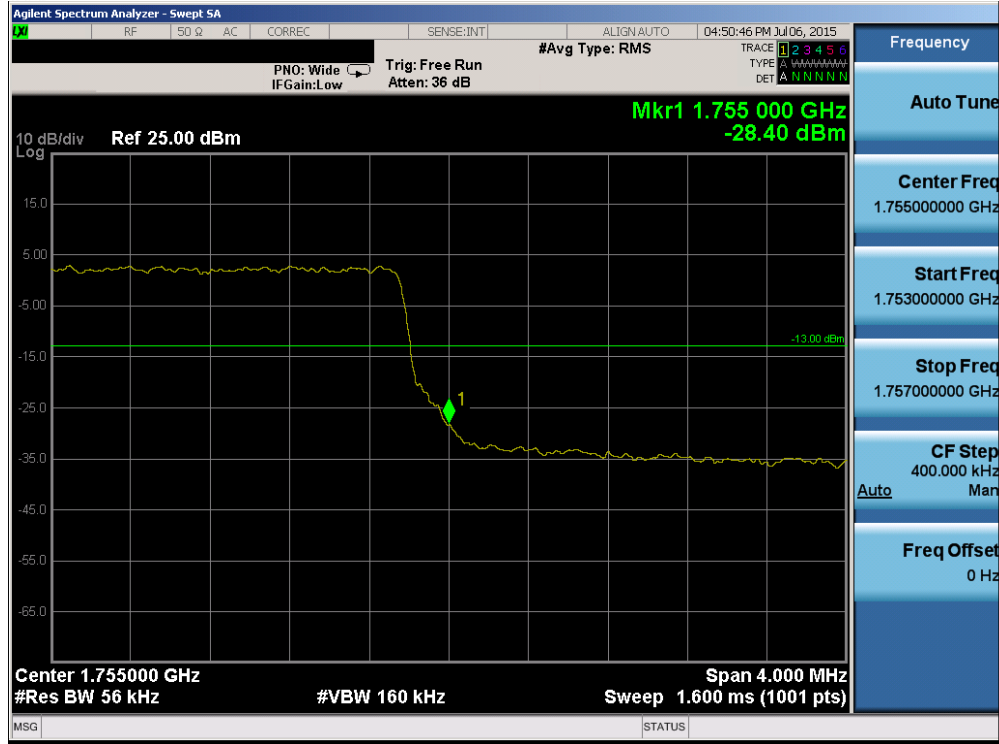
Plot 6-74. Upper Band Edge Plot (Band 4 – 5.0MHz QPSK – RB Size 25)
