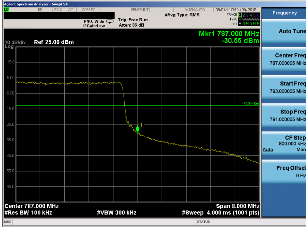
Plot 6-62. Upper Band Edge Plot (Band 13 – 10.0MHz QPSK – RB Size 50)
