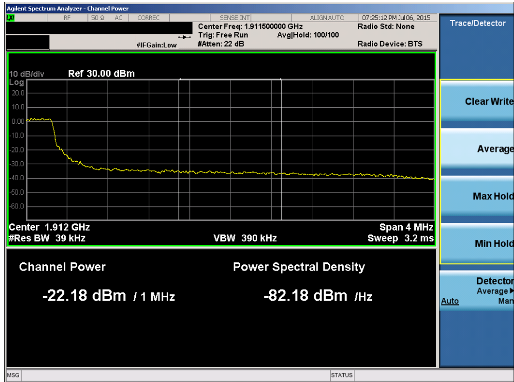
Plot 6-99. Upper Extended Band Edge Plot (Band 2 – 5.0MHz QPSK – RB Size 25)
