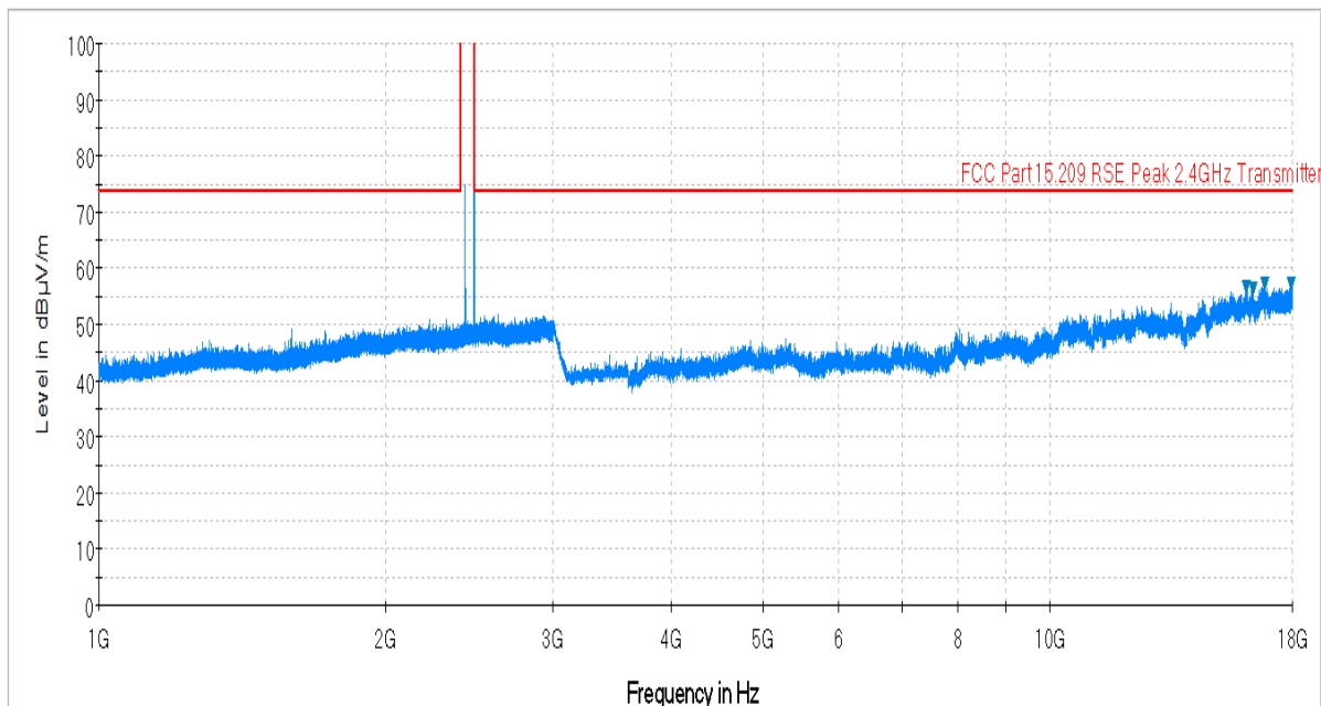
Plot 6-46. Radiated Spurious Plot above 1GHz (BT – Ch. 78, Ant. Pol. H)
