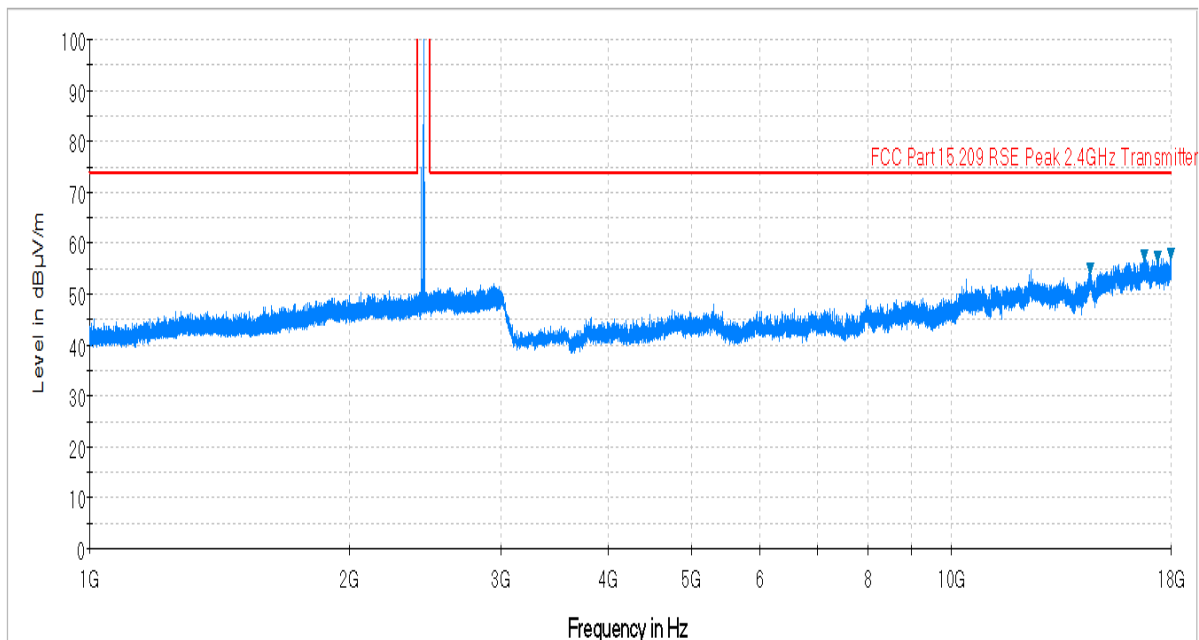
Plot 6-44. Radiated Spurious Plot above 1GHz (BT – Ch. 39, Ant. Pol. H)
