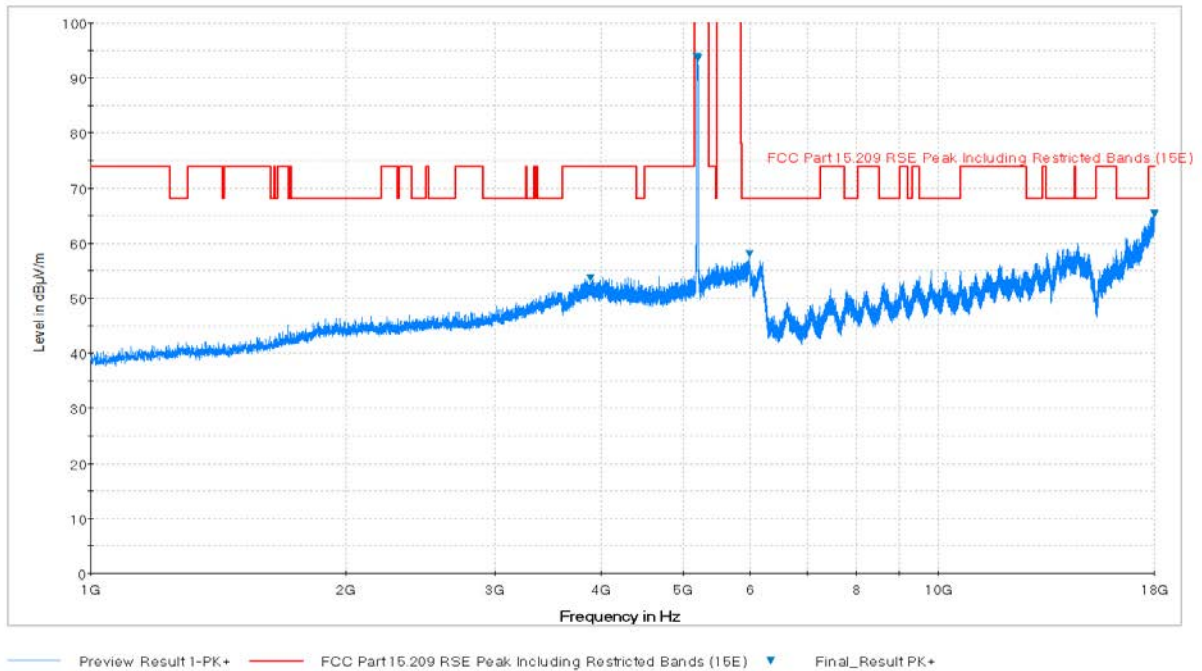
Plot 6-67. Radiated Spurious Plot above 1GHz (802.11a – U1 Ch. 40, Ant. Pol. H)
