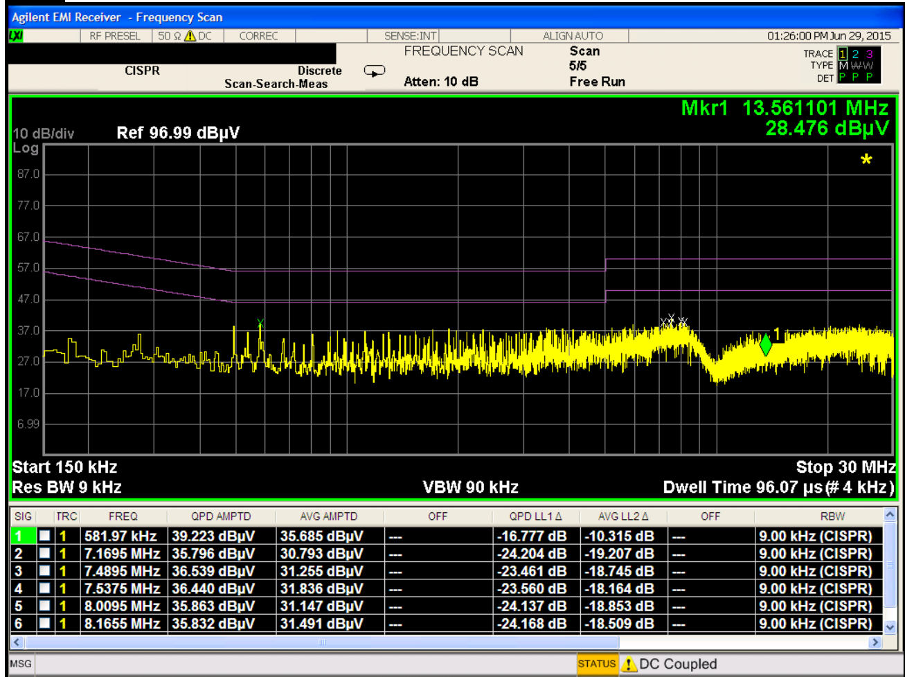
Plot 6-94. Line Conducted Plot with 802.11a UNII Band 2A (L1)
