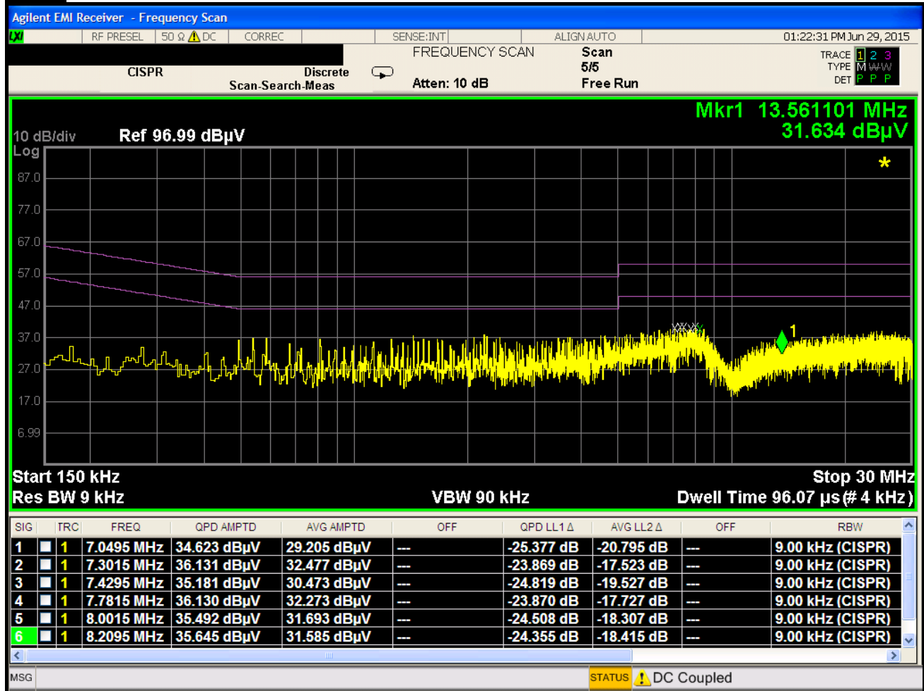
Plot 6-92. Line Conducted Plot with 802.11a UNII Band 1 (L1)
