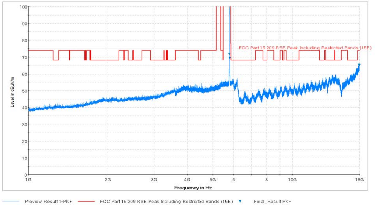
Plot 6-73. Radiated Spurious Plot above 1GHz (802.11a – U3 Ch. 157, Ant. Pol. H)
