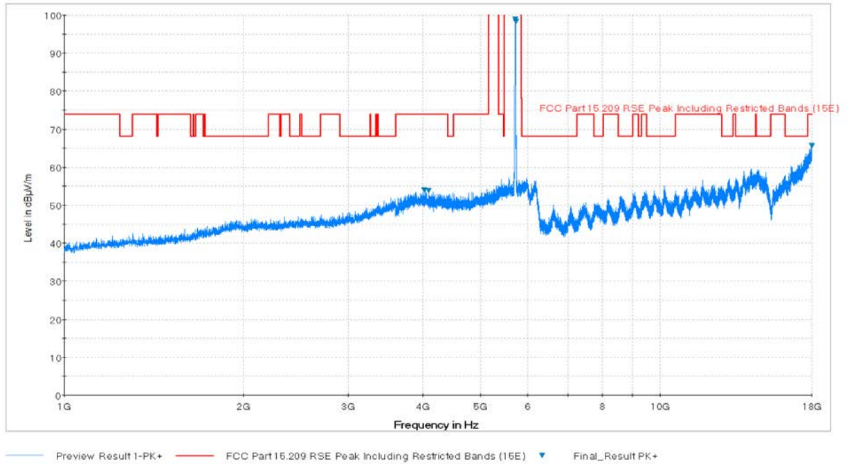
Plot 6-71. Radiated Spurious Plot above 1GHz (802.11a – U2C Ch. 120, Ant. Pol. H)
