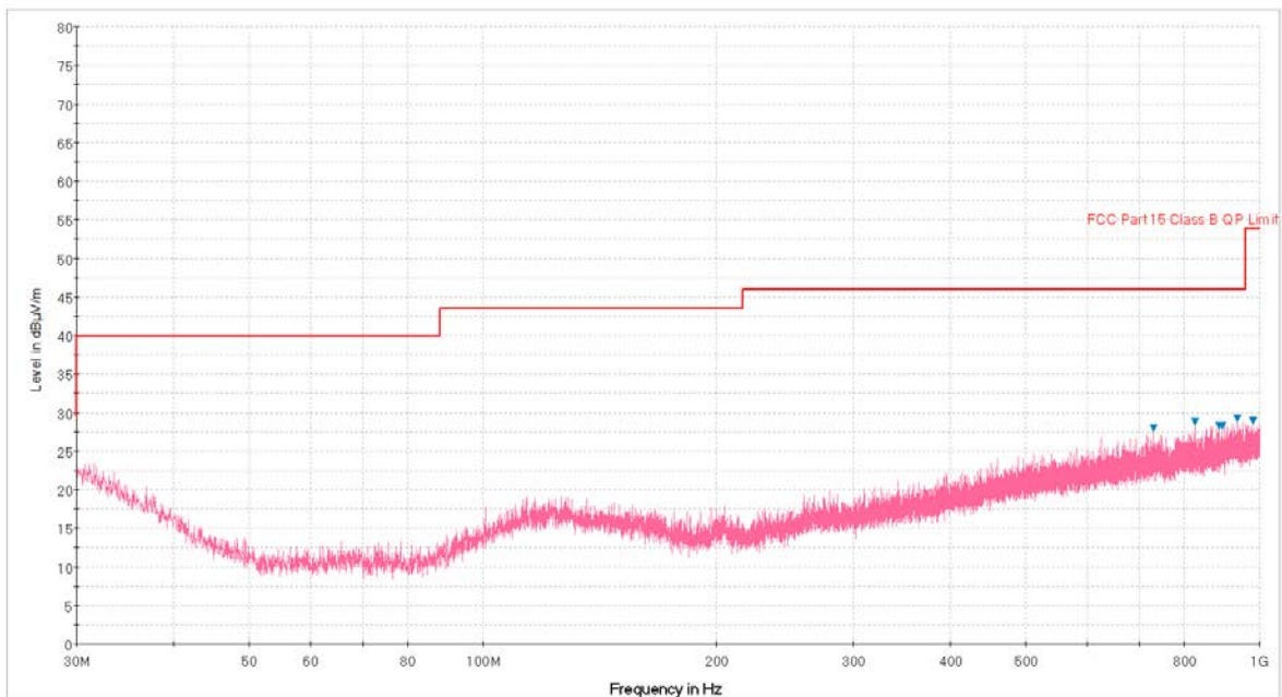
Plot 6-91. Radiated Spurious Plot below 1GHz (802.11a – U3 Ch. 157, Ant. Pol. V)
