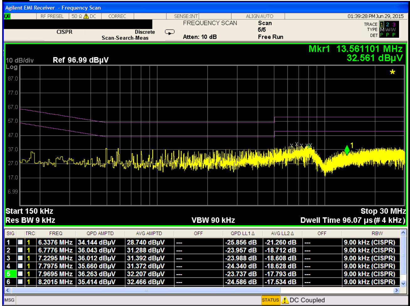
Plot 6-98. Line Conducted Plot with 802.11a UNII Band 3 (L1)
