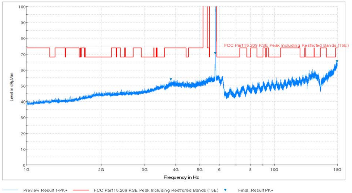
Plot 6-74. Radiated Spurious Plot above 1GHz (802.11a – U3 Ch. 157, Ant. Pol. V)
