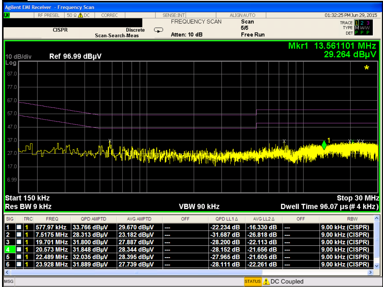
Plot 6-97. Line Conducted Plot with 802.11a UNII Band 2C (N)
