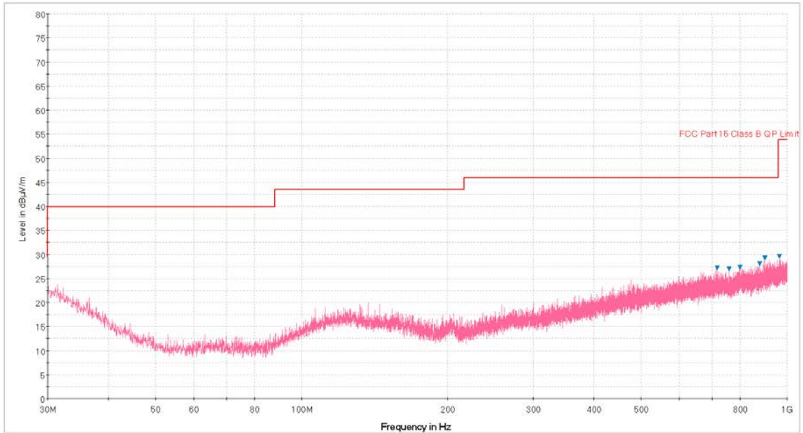
Plot 6-90. Radiated Spurious Plot below 1GHz (802.11a – U3 Ch. 157, Ant. Pol. H)
