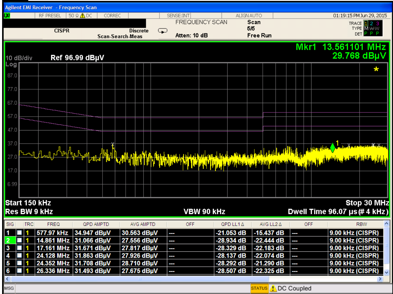
Plot 6-93. Line Conducted Plot with 802.11a UNII Band 1 (N)
