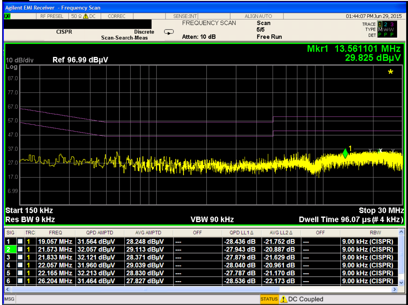
Plot 6-99. Line Conducted Plot with 802.11a UNII Band 3 (N)
