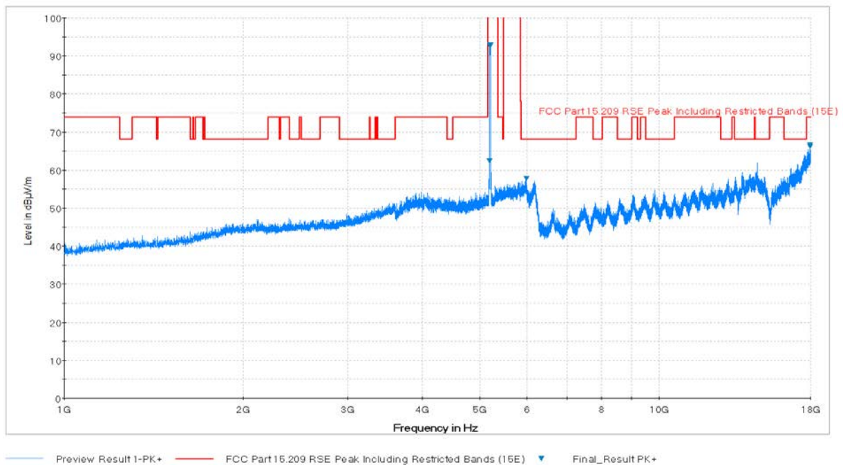
Plot 6-68. Radiated Spurious Plot above 1GHz (802.11a – U1 Ch. 40, Ant. Pol. V)
