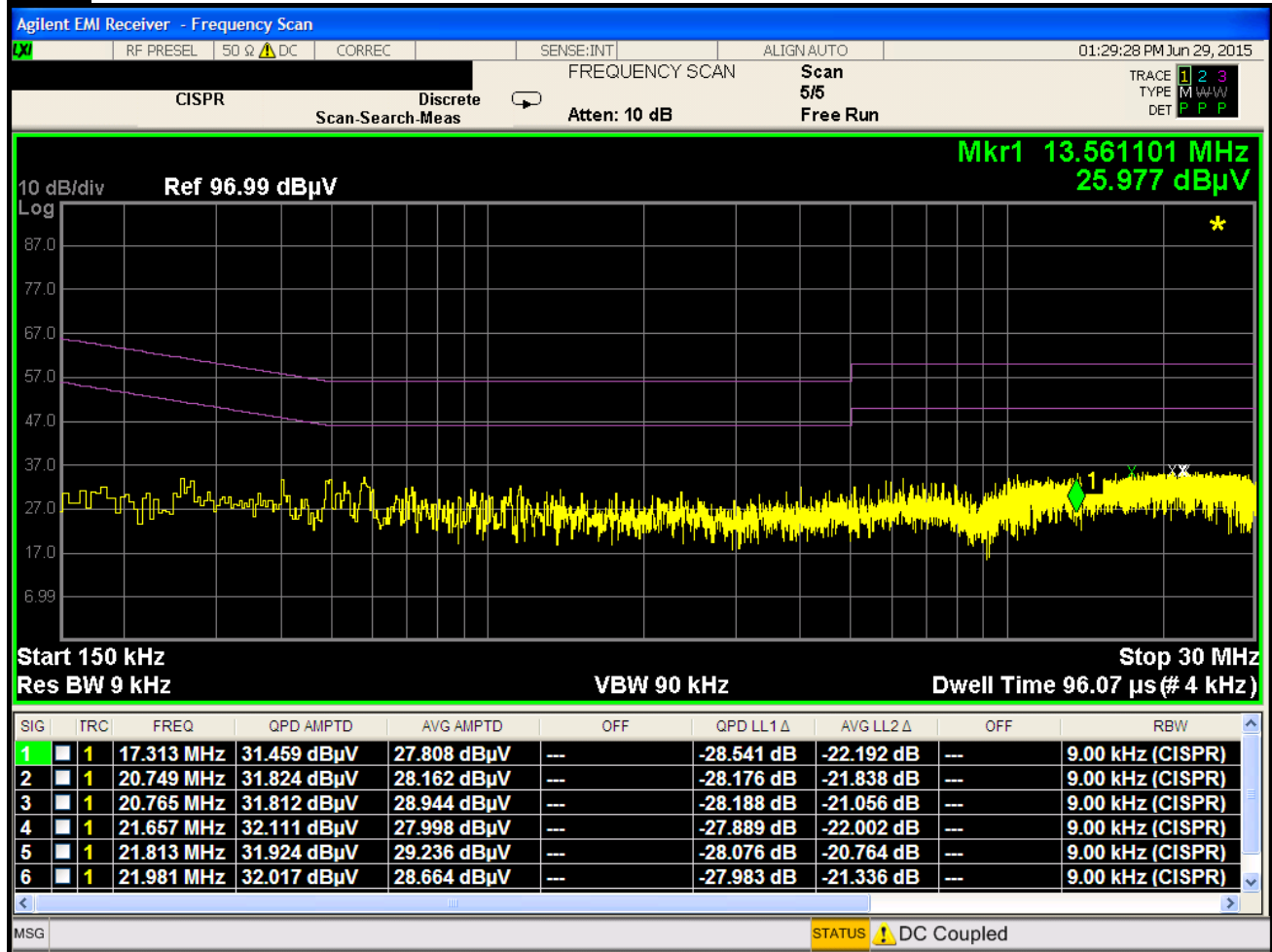
Plot 6-95. Line Conducted Plot with 802.11a UNII Band 2A (N)
