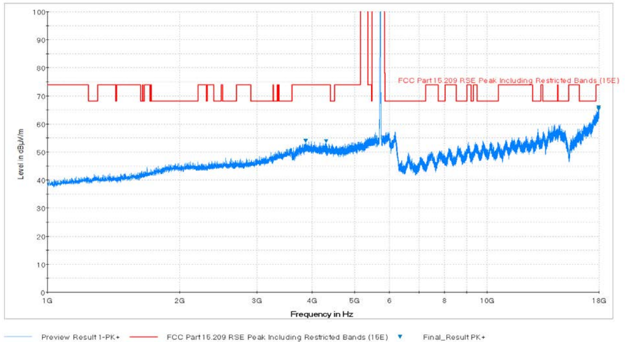
Plot 6-72. Radiated Spurious Plot above 1GHz (802.11a – U2C Ch. 120, Ant. Pol. V)
