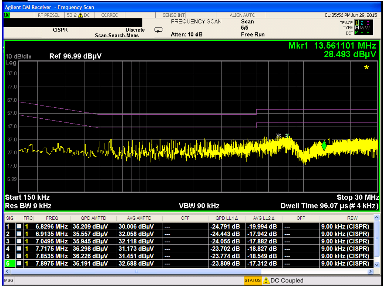
Plot 6-96. Line Conducted Plot with 802.11a UNII Band 2C (L1)
