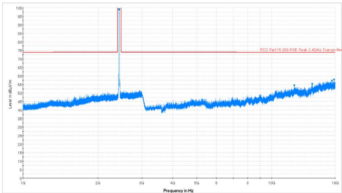
Plot 6-34. Radiated Spurious Plot above 1GHz (802.11b – Ch. 6, Ant. Pol. V)
