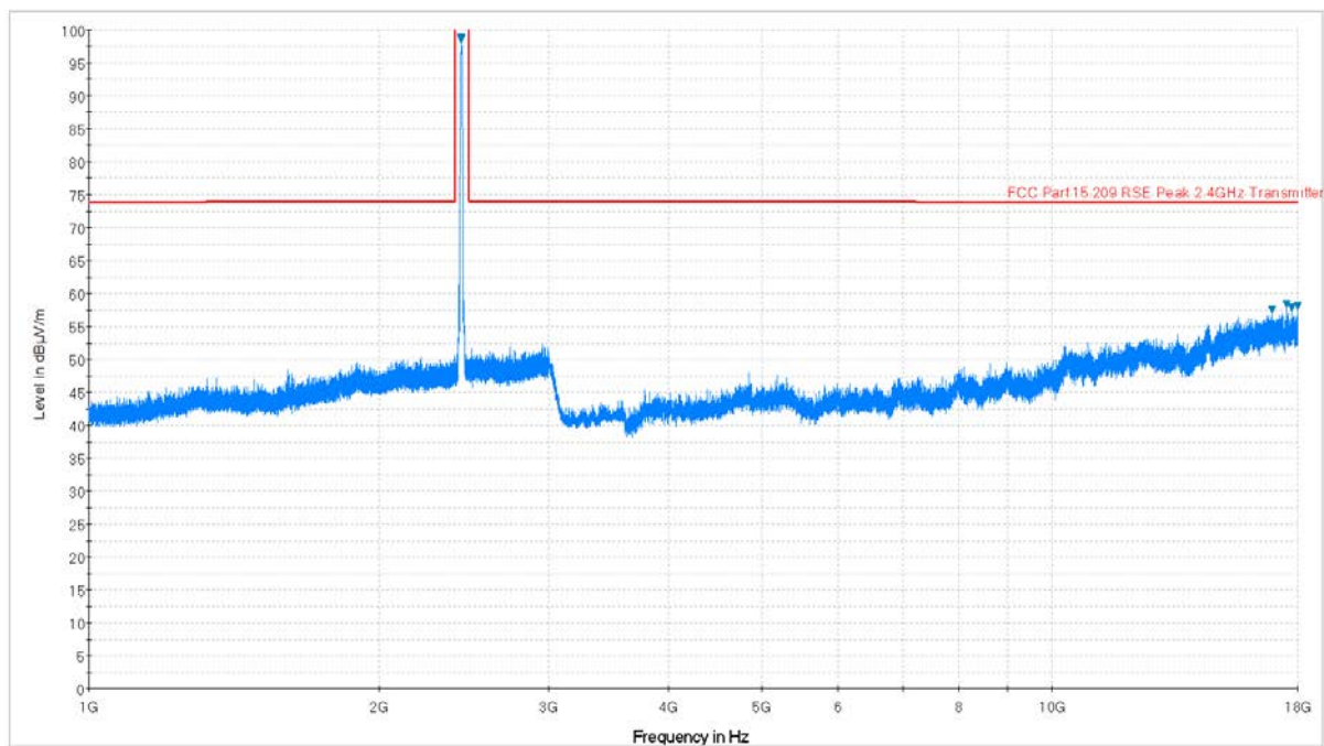
Plot 6-33. Radiated Spurious Plot above 1GHz (802.11b – Ch. 6, Ant. Pol. H)
