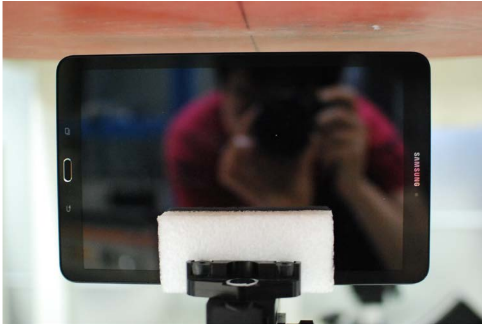
SAR Test Setup Photo 5: Left Edge at 1.1 cm
