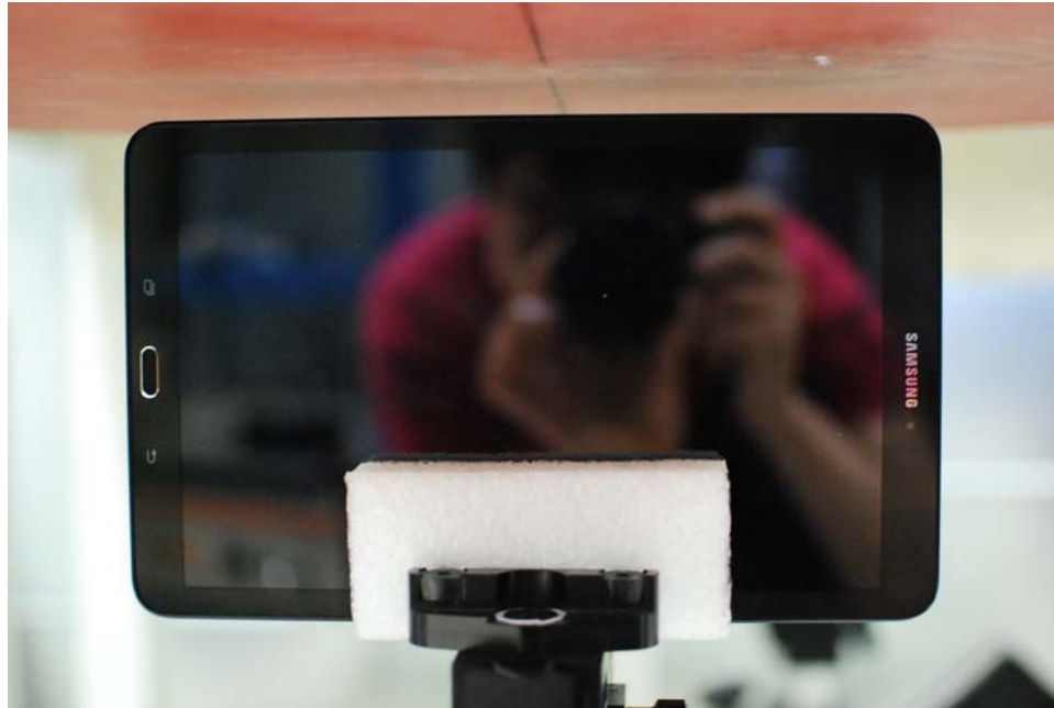
SAR Test Setup Photo 7: Left Edge at 1.1 cm
