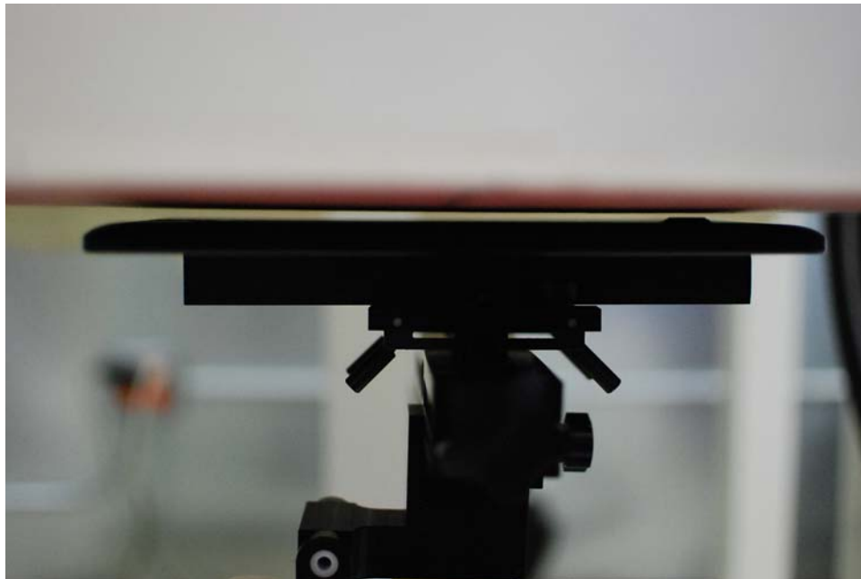
SAR Test Setup Photo 2: Back Side at 0.3 cm
