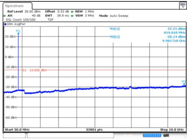
5M BW 16QAM High ch.
