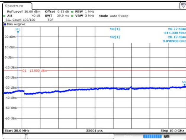
3M BW QPSK High ch.
