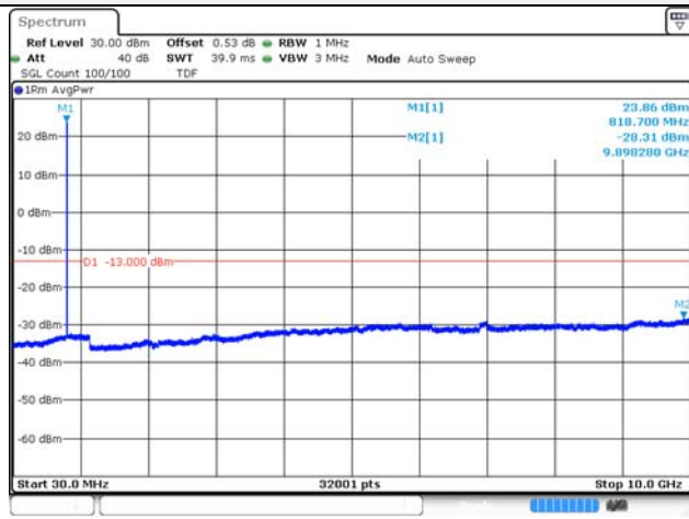
5M BW QPSK High ch.
