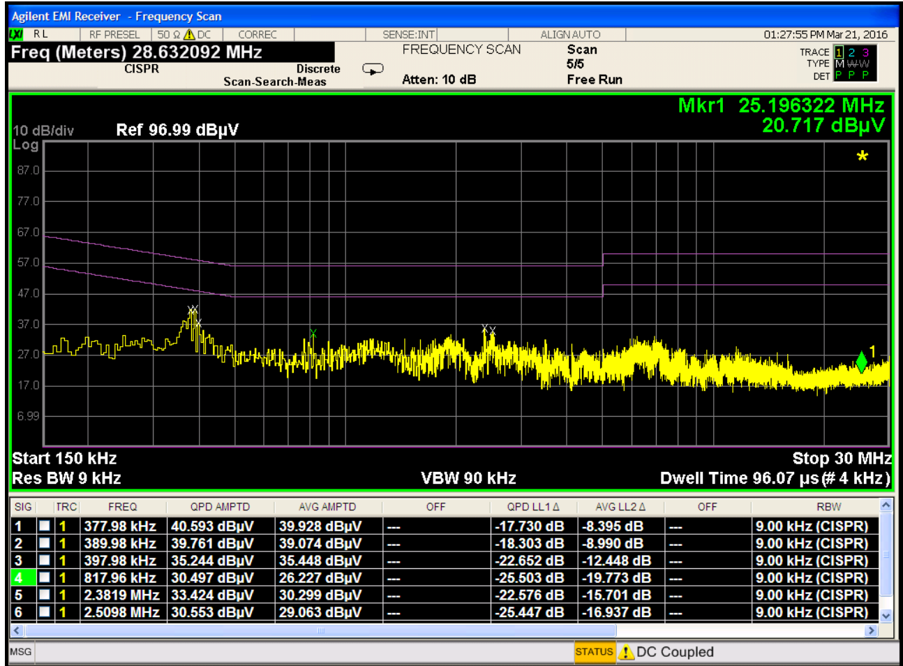
Plot 7-6. Line-Conducted Test Plot (L1)
