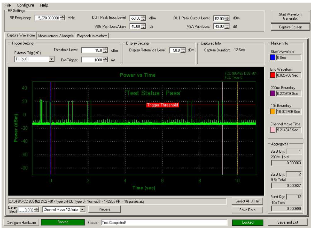
Figure 5-5. Band 2A Move Time and Aggregate Time
