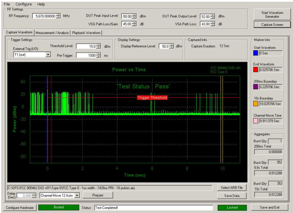
Figure 5-6. Band 2C Move Time and Aggregate Time
