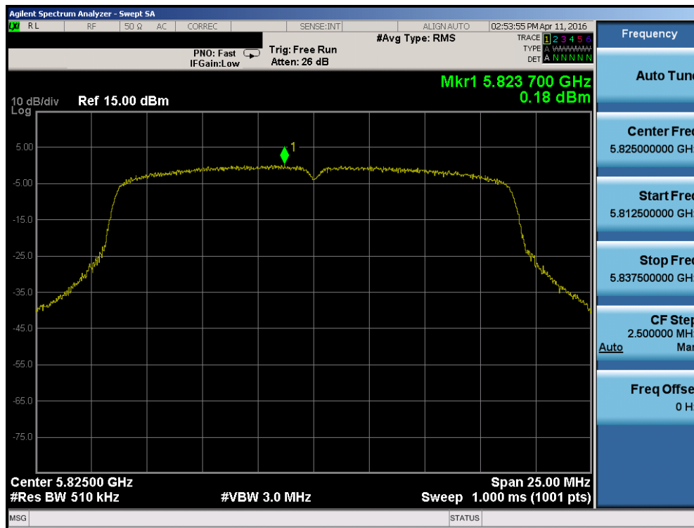
Plot 7-75. Power Spectral Density Plot (20MHz BW 802.11n (UNII Band 3) – Ch. 165)
