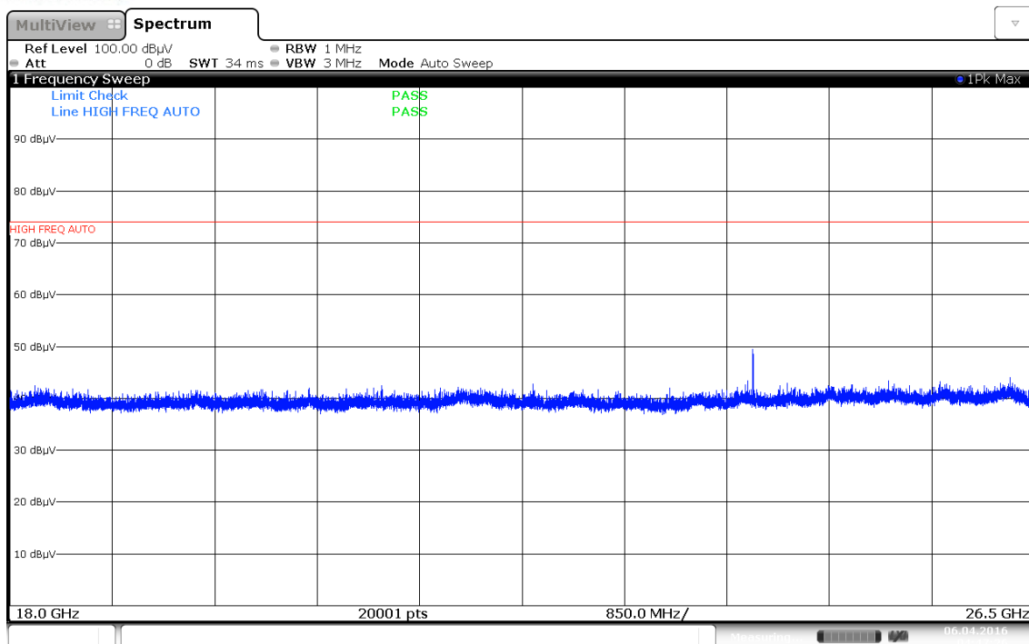
Plot 7-89. Radiated Spurious Plot above 18GHz (802.11a – Ant. Pol. V)
