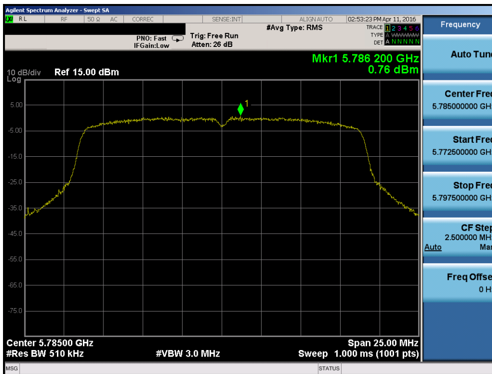
Plot 7-74. Power Spectral Density Plot (20MHz BW 802.11n (UNII Band 3) – Ch. 157)
