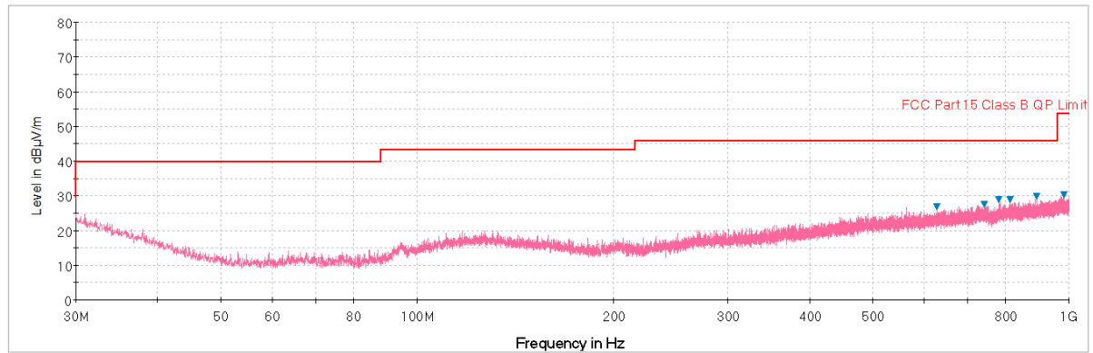
Plot 7-112. Radiated Spurious Plot below 1GHz (802.11a – U3 Ch. 157, Ant. Pol. H)
