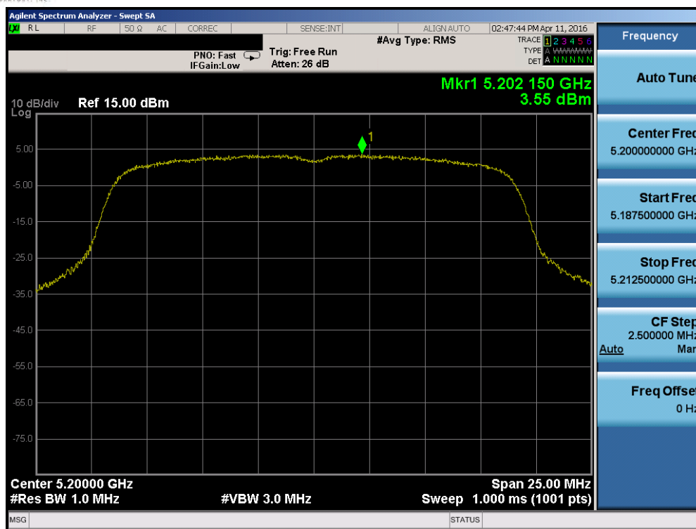
Plot 7-44. Power Spectral Density Plot (20MHz BW 802.11n (UNII Band 1) – Ch. 40)
