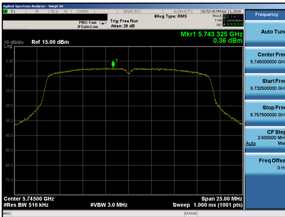
Plot 7-73. Power Spectral Density Plot (20MHz BW 802.11n (UNII Band 3) – Ch. 149)
