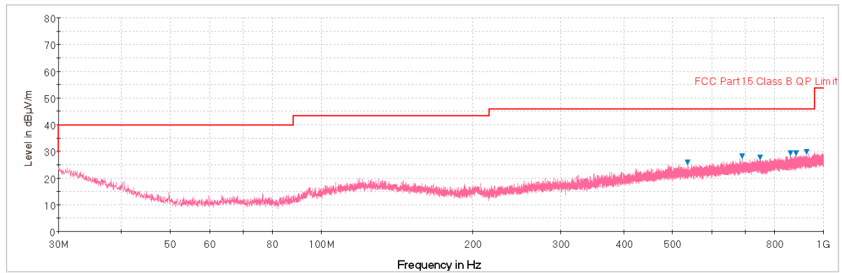
Plot 7-113. Radiated Spurious Plot below 1GHz (802.11a – U3 Ch. 157, Ant. Pol. V)
