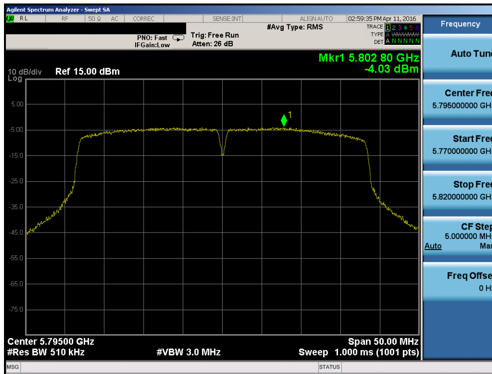
Plot 7-77. Power Spectral Density Plot (40MHz BW 802.11n (UNII Band 3) – Ch. 159)
