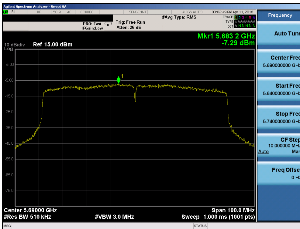
Plot 7-69. Power Spectral Density Plot (80MHz BW 802.11ac (UNII Band 2C) – Ch. 138)
