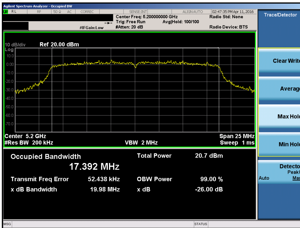
Plot 7-5. 26dB Bandwidth Plot (20MHz BW 802.11n (UNII Band 1) – Ch. 40)
