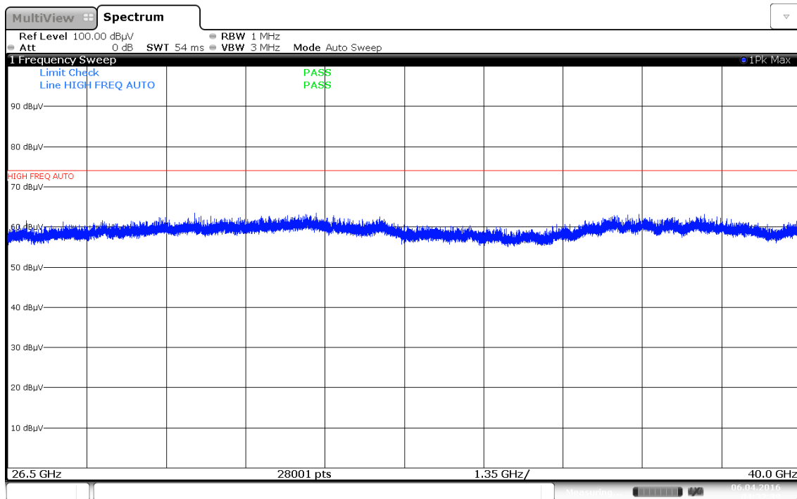
Plot 7-88. Radiated Spurious Plot above 18GHz (802.11a – Ant. Pol. H)
