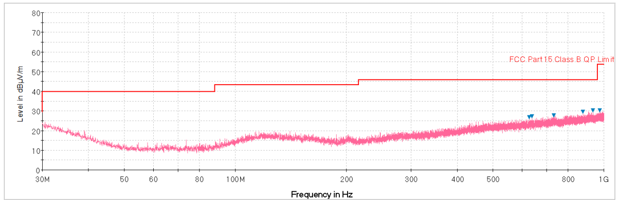
Plot 7-53. Radiated Spurious Plot below 1GHz (Pol. H)
