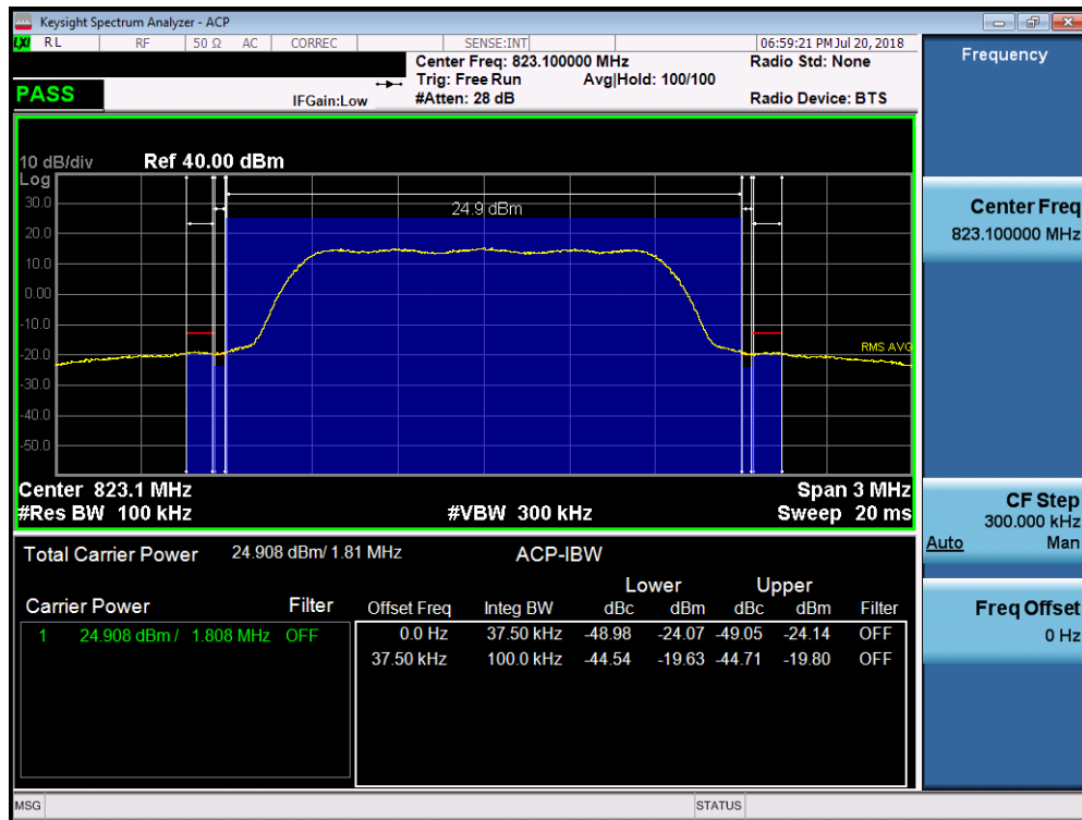
Plot 7-25. Channel Edge Plot (Ch. 684)
