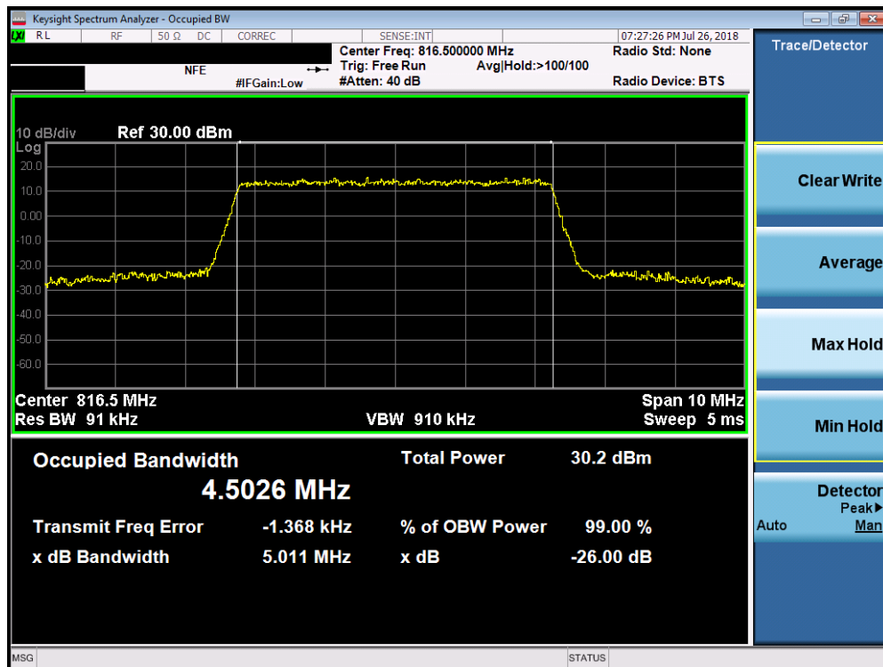
Plot 7-7. Occupied Bandwidth Plot (LTE Band 26, 5MHz 16-QAM – RB Size 25– Low Channel)
