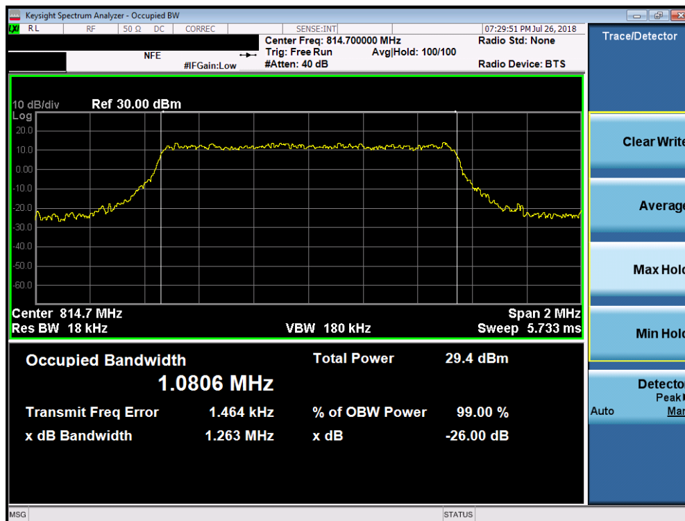
Plot 7-3. Occupied Bandwidth Plot (LTE Band 26, 1.4MHz 16-QAM – RB Size 6– Low Channel)
