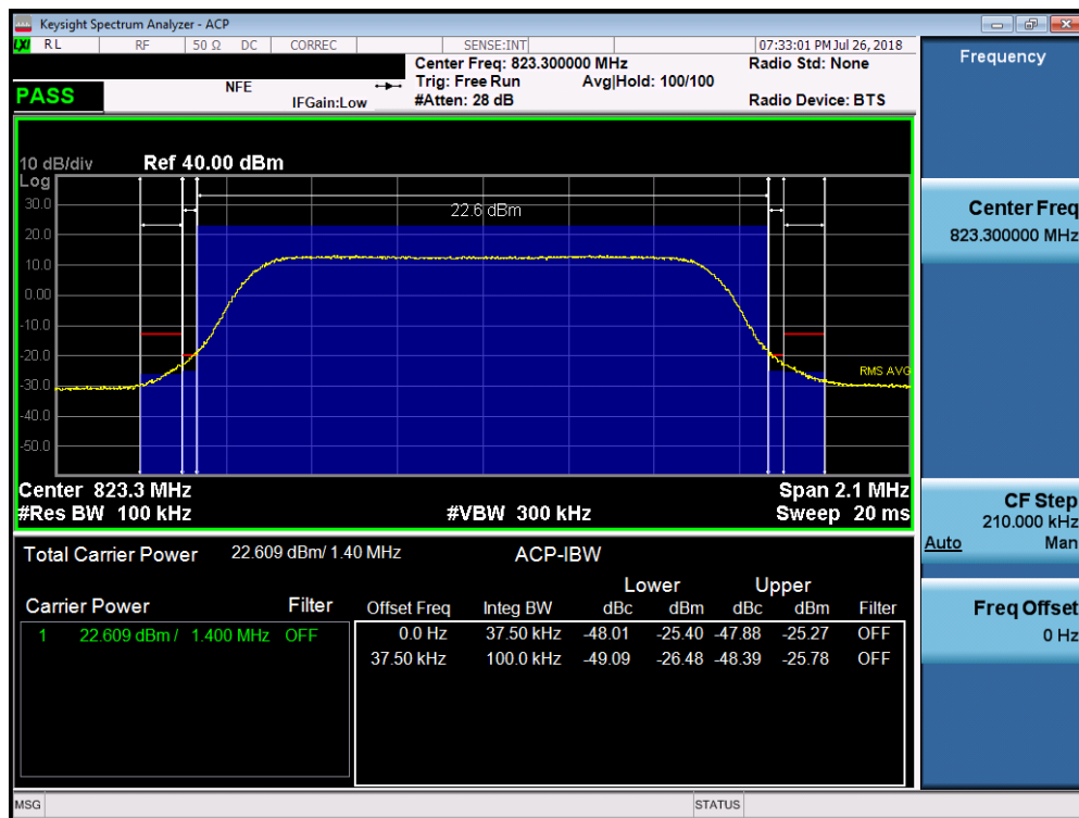
Plot 7-27. Channel Edge Plot (LTE Band 26, 1.4MHz QPSK – RB Size 6 – High Channel)
