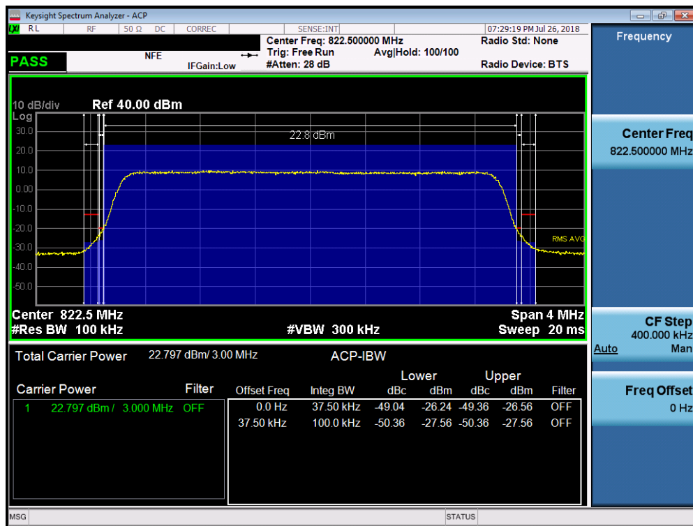
Plot 7-29. Channel Edge Plot (LTE Band 26, 3MHz QPSK – RB Size 15 – High Channel)
