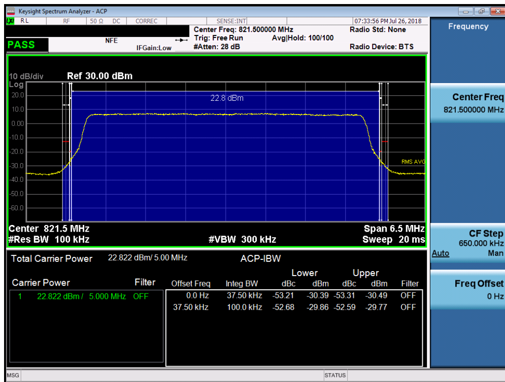
Plot 7-31. Channel Edge Plot (LTE Band 26, 5MHz QPSK – RB Size 25 – High Channel)
