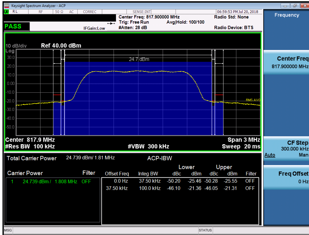
Plot 7-24. Channel Edge Plot (Ch. 476)
