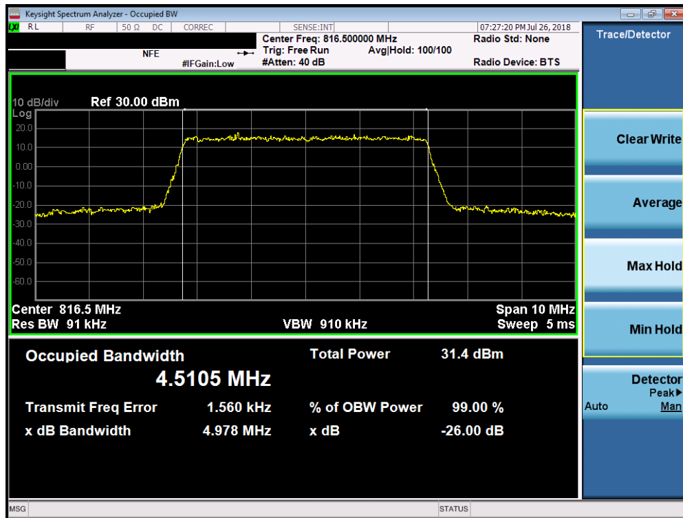
Plot 7-6. Occupied Bandwidth Plot (LTE Band 26, 5MHz QPSK – RB Size 25– Low Channel)
