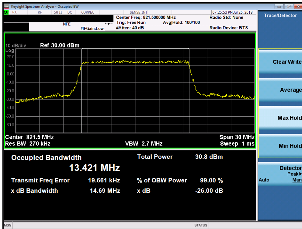
Plot 7-11. Occupied Bandwidth Plot (LTE Band 26, 15MHz 16-QAM – RB Size 75)
