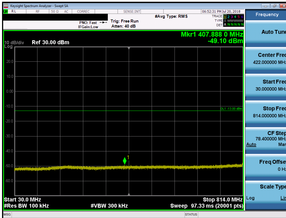
Plot 7-12. Conducted Spurious Plot (CDMA, Ch. 476)
