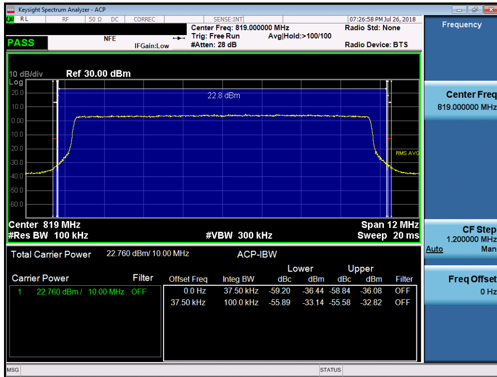
Plot 7-32. Channel Edge Plot (LTE Band 26, 10MHz QPSK – RB Size 50)
