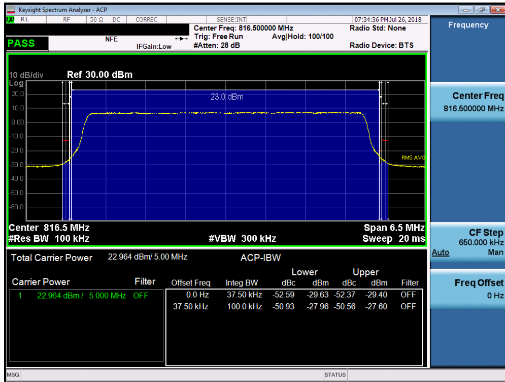
Plot 7-30. Channel Edge Plot (LTE Band 26, 5MHz QPSK – RB Size 25– Low Channel)
