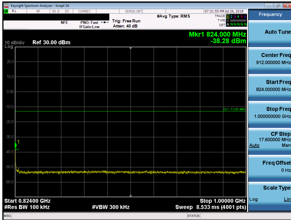
Plot 7-22. Conducted Spurious Plot (LTE Band 26, 1.4MHz QPSK – RB Size 1, RB Offset 0 – High Channel)
