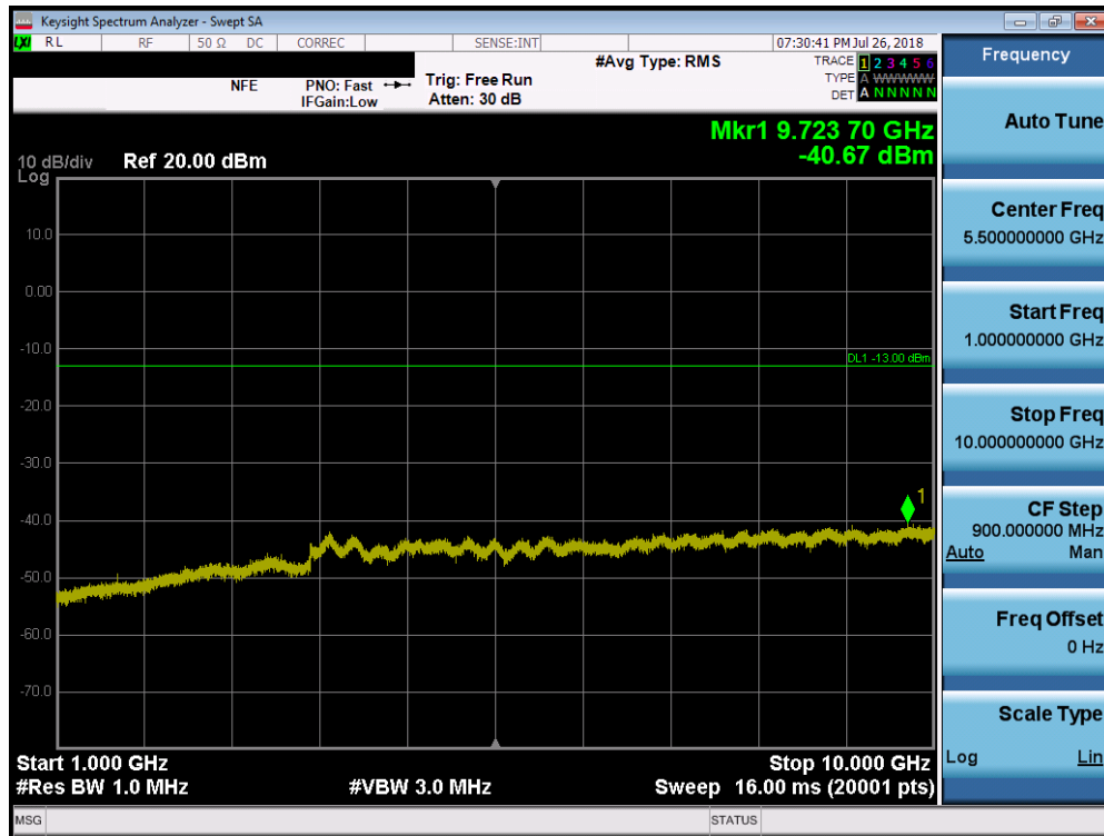
Plot 7-20. Conducted Spurious Plot (LTE Band 26, 1.4MHz QPSK – RB Size 1, RB Offset 0 – Low Channel)
