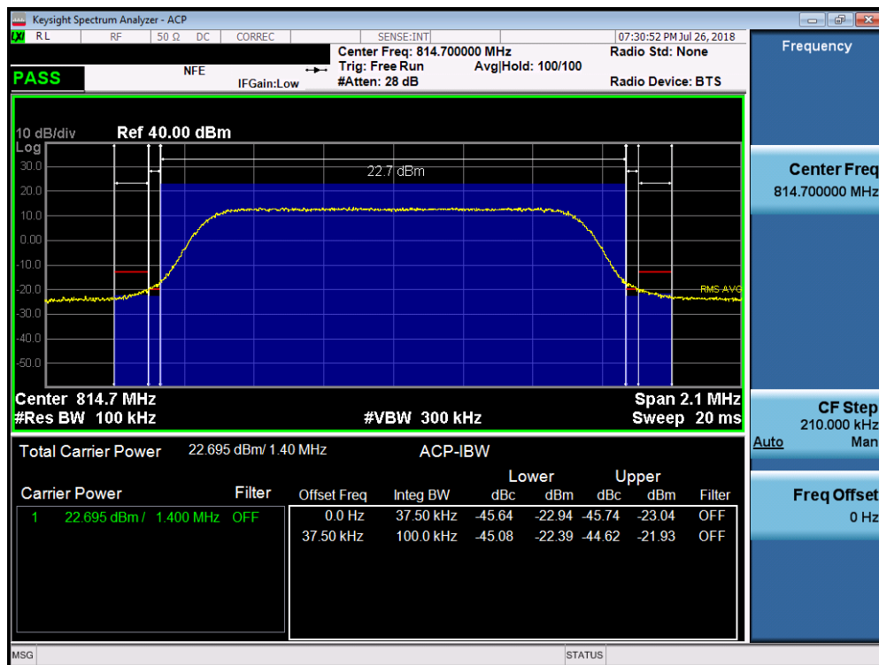
Plot 7-26. Channel Edge Plot (LTE Band 26, 1.4MHz QPSK – RB Size 6– Low Channel)
