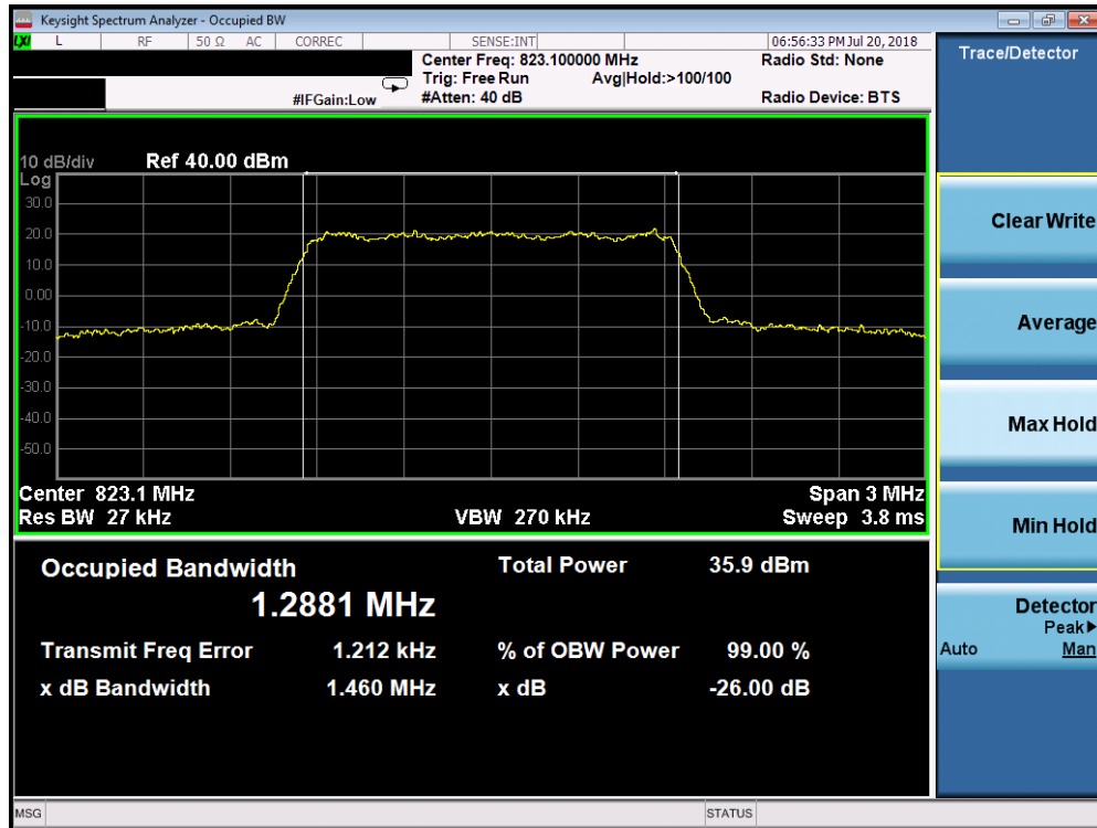
Plot 7-1. Occupied Bandwidth Plot (CDMA Ch. 684)
