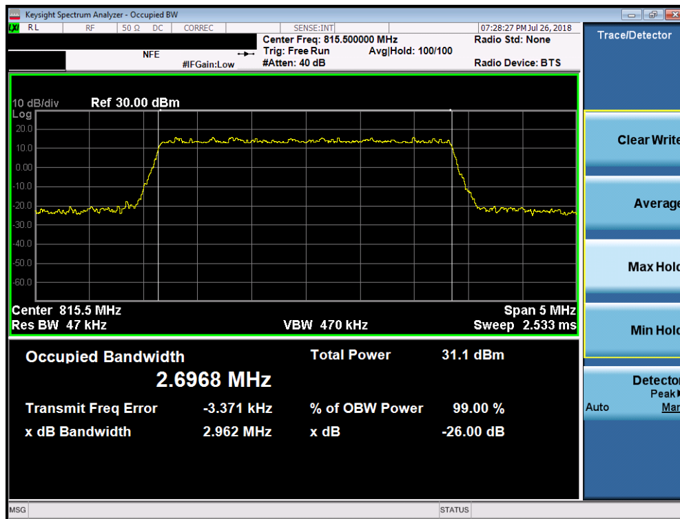
Plot 7-4. Occupied Bandwidth Plot (LTE Band 26, 3MHz QPSK – RB Size 15– Low Channel)
