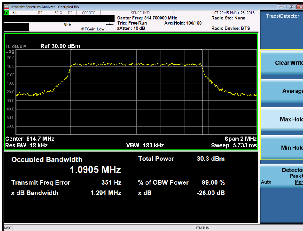
Plot 7-2. Occupied Bandwidth Plot (LTE Band 26, 1.4MHz QPSK – RB Size 6– Low Channel)
