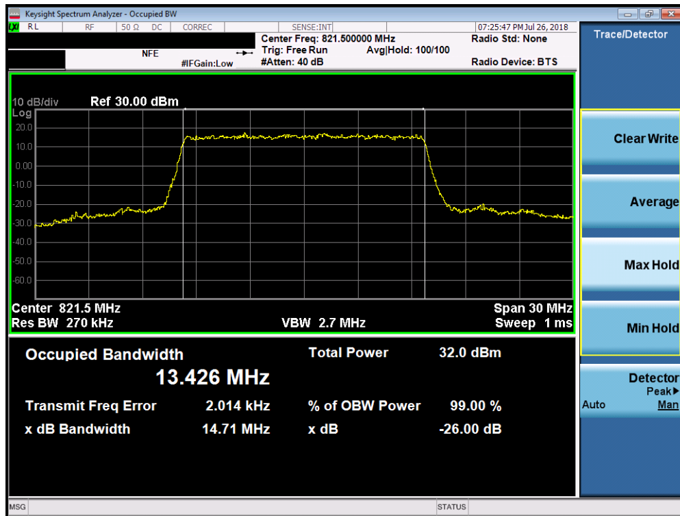
Plot 7-10. Occupied Bandwidth Plot (LTE Band 26, 15MHz QPSK – RB Size 75)
