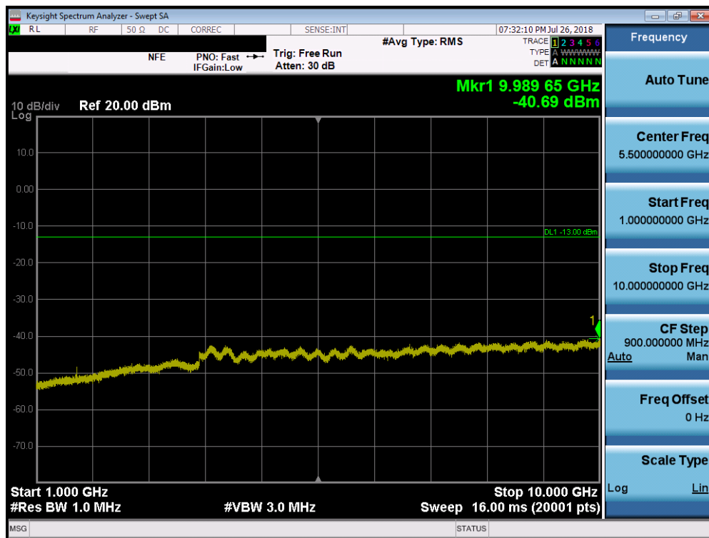
Plot 7-23. Conducted Spurious Plot (LTE Band 26, 1.4MHz QPSK – RB Size 1, RB Offset 0 – High Channel)
