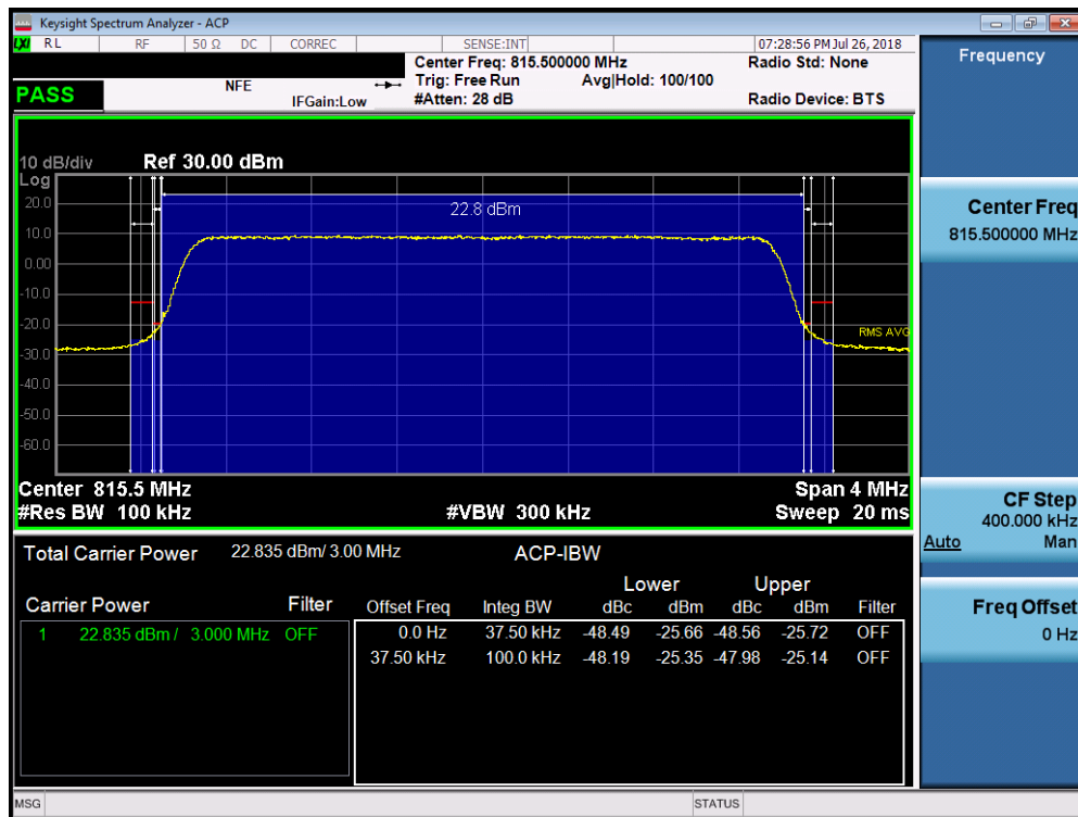
Plot 7-28. Channel Edge Plot (LTE Band 26, 3MHz QPSK – RB Size 15– Low Channel)
