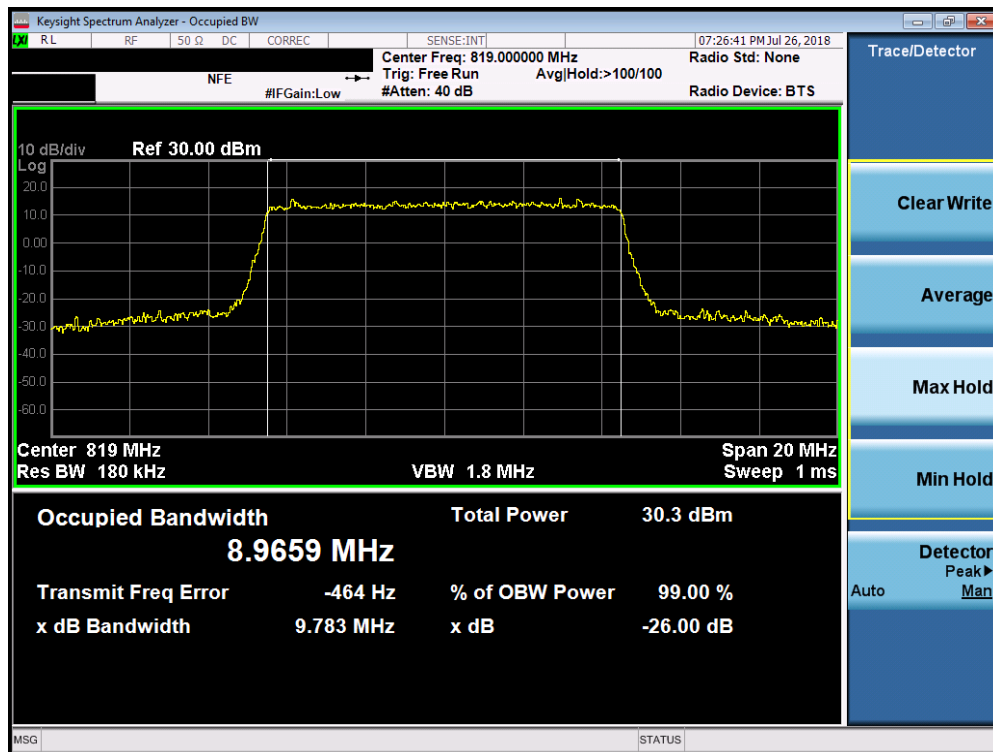
Plot 7-9. Occupied Bandwidth Plot (LTE Band 26, 10MHz 16-QAM – RB Size 50)
