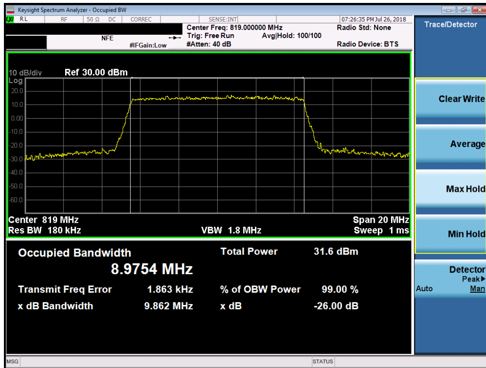
Plot 7-8. Occupied Bandwidth Plot (LTE Band 26, 10MHz QPSK – RB Size 50)
