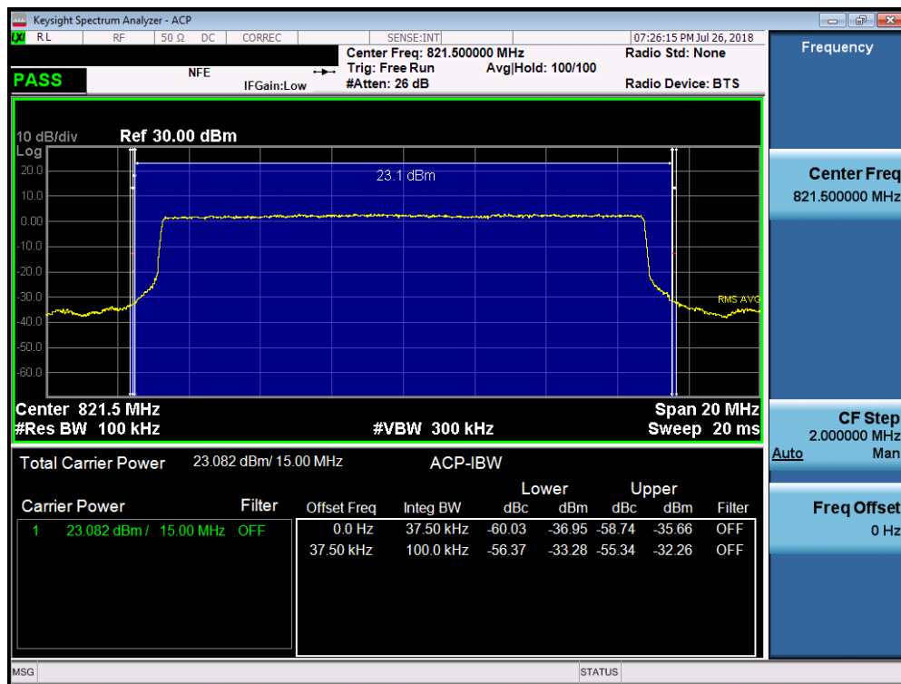
Plot 7-33. Channel Edge Plot (LTE Band 26, 15MHz QPSK – RB Size 75)
