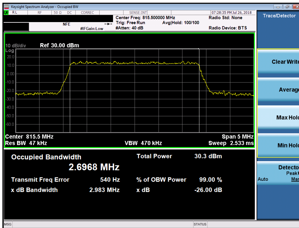
Plot 7-5. Occupied Bandwidth Plot (LTE Band 26, 3MHz 16-QAM – RB Size 15– Low Channel)
