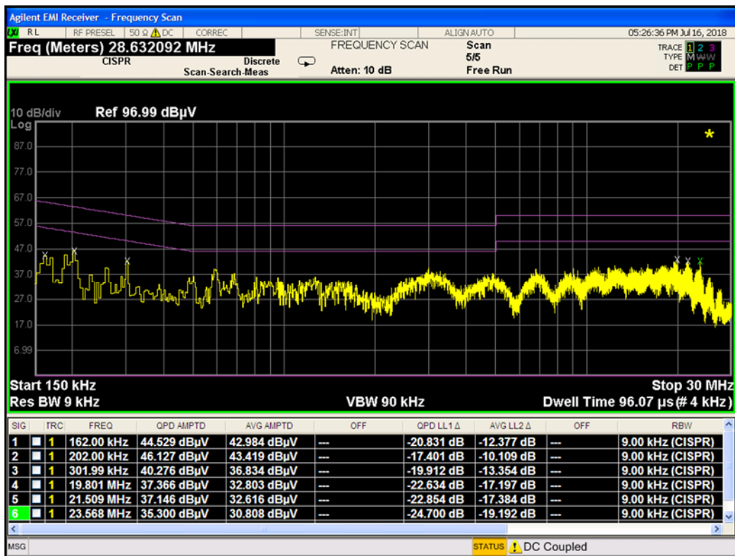
Plot 7-4. Line Conducted Plot (N)
