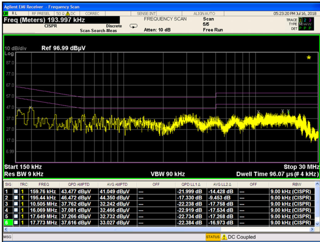
Plot 7-3. Line Conducted Plot (L1)
