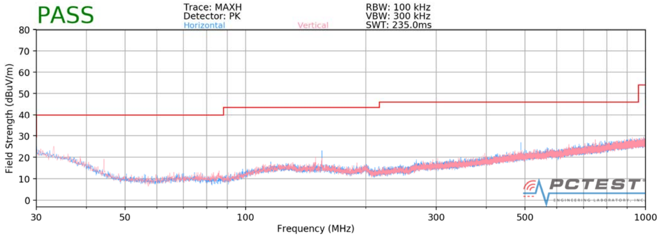
Plot 7-108. Radiated Spurious Plot below 1GHz (802.11a – U3 Ch. 157)
