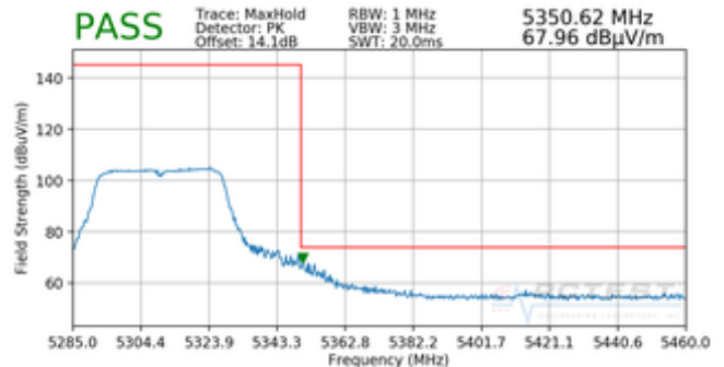
Plot 7-95. Radiated Upper Band Edge Plot (Peak – UNII Band 2A)
