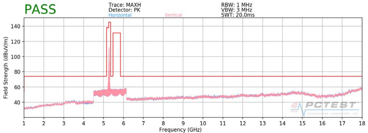
Plot 7-78. Radiated Spurious Plot above 1GHz (802.11a – U2A Ch. 56)
