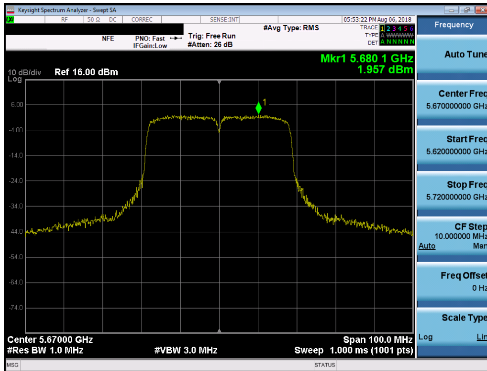
Plot 7-65. Power Spectral Density Plot (40MHz BW 802.11n (UNII Band 2C) – Ch. 134)
