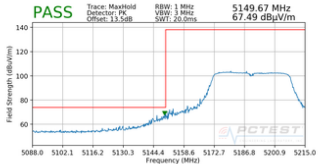
Plot 7-93. Radiated Lower Band Edge Plot (Peak – UNII Band 1)
