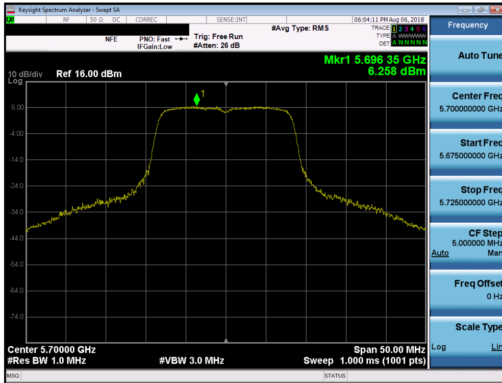
Plot 7-59. Power Spectral Density Plot (802.11a (UNII Band 2C) – Ch. 140)
