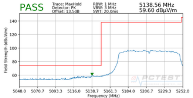
Plot 7-102. Radiated Lower Band Edge Plot (Peak – UNII Band 1)
