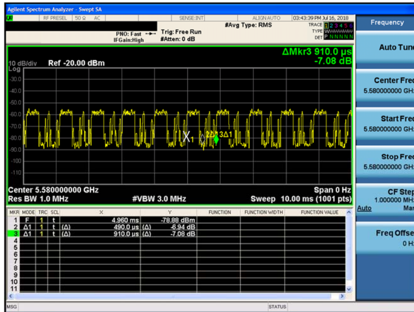
Figure 5-2. Band 2C Pulse Width & Period
