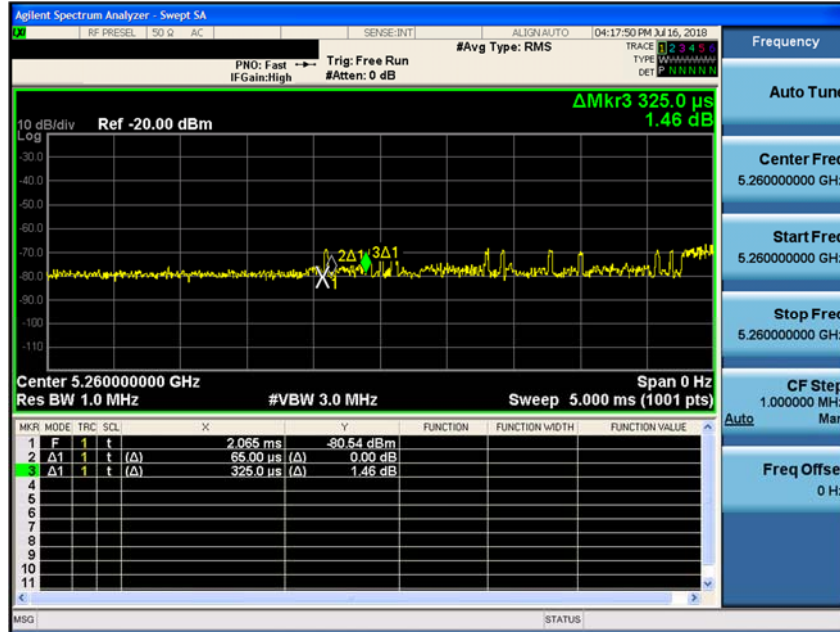
Figure 5-1. Band 2A Pulse Width & Period
