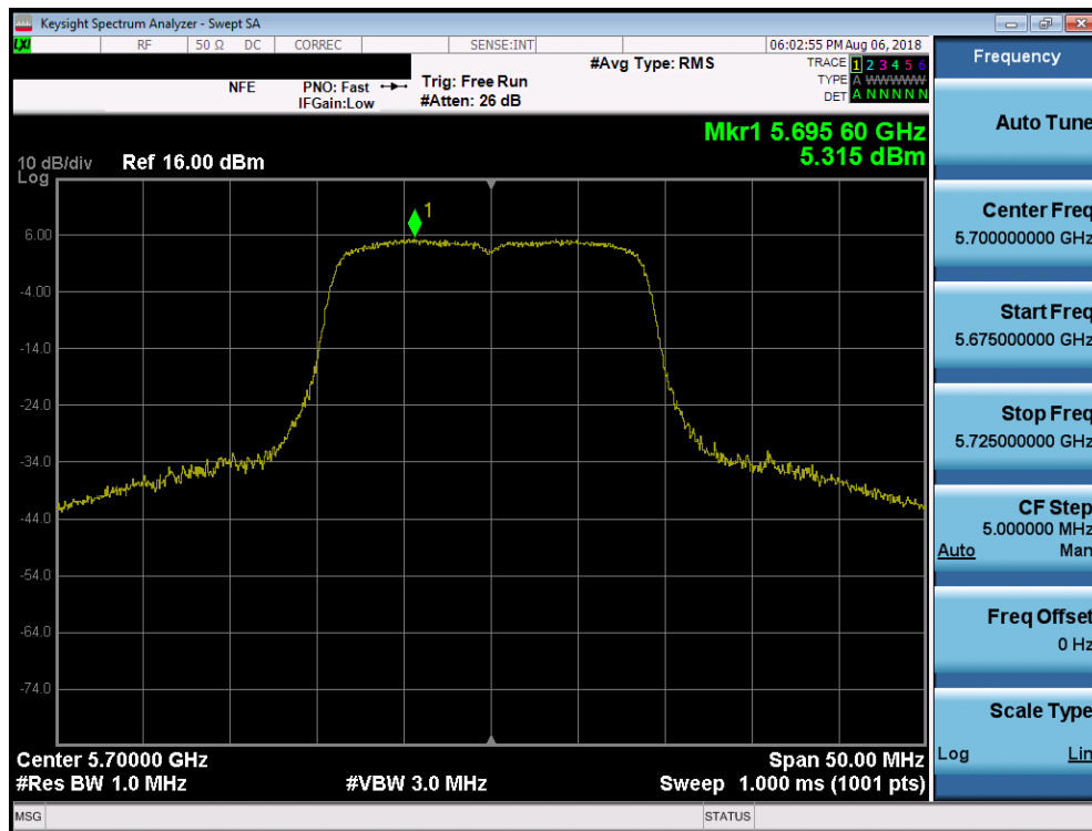
Plot 7-62. Power Spectral Density Plot (20MHz BW 802.11n (UNII Band 2C) – Ch. 140)
