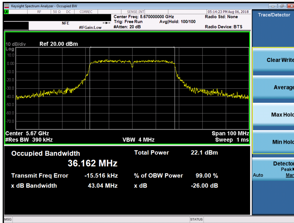
Plot 7-27. 26dB Bandwidth Plot (40MHz BW 802.11n (UNII Band 2C) – Ch. 134)
