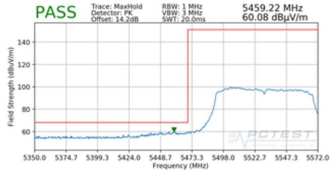
Plot 7-106. Radiated Lower Band Edge Plot (Peak – UNII Band 2C)
