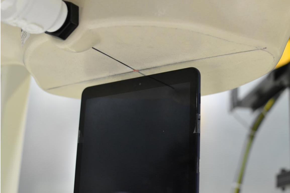
SAR Test Setup Photo 7 – Top Edge at 0.7 cm
