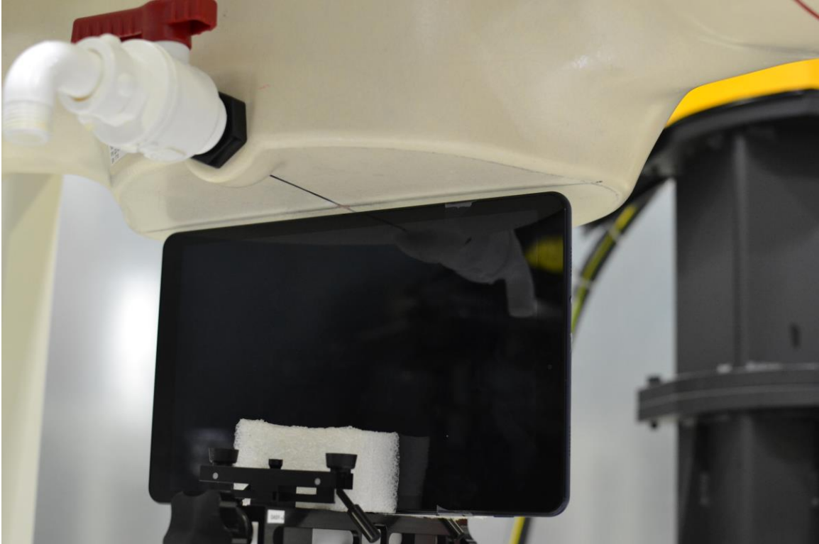
SAR Test Setup Photo 11 – Left Edge at 0.5 cm
