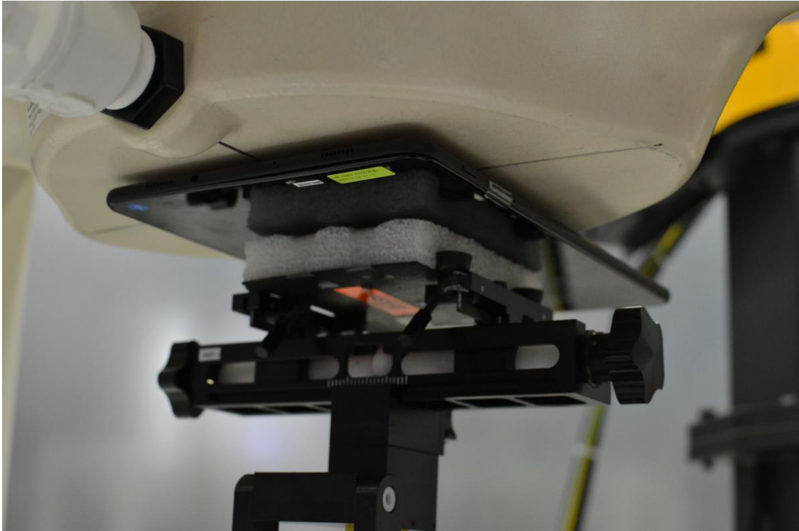
SAR Test Setup Photo 3 – Back Side at 0.7 cm
