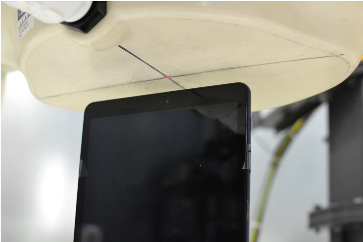
SAR Test Setup Photo 6 – Top Edge at 1.4 cm
