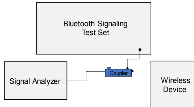
Figure 8-4 Power Measurement Setup
