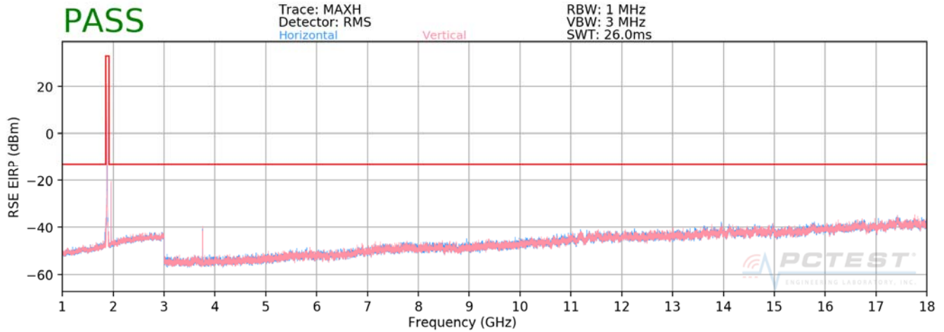
Plot 7-46. Radiated Spurious Plot (PCS WCDMA Mode)
