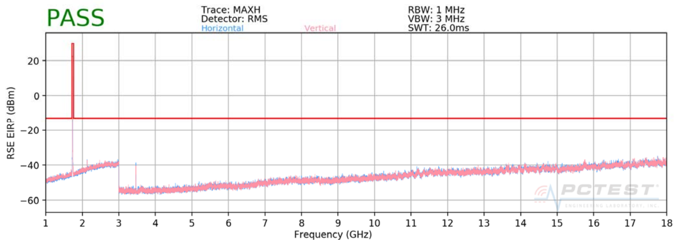
Plot 7-45. Radiated Spurious Plot (AWS WCDMA Mode)
