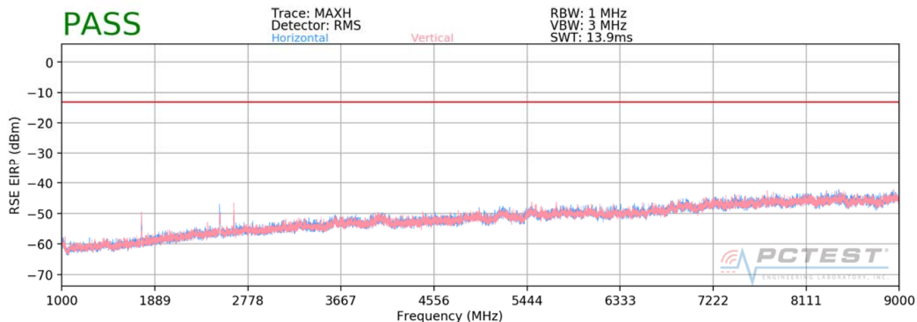
Plot 7-44. Radiated Spurious Plot (Cell WCDMA Mode)
