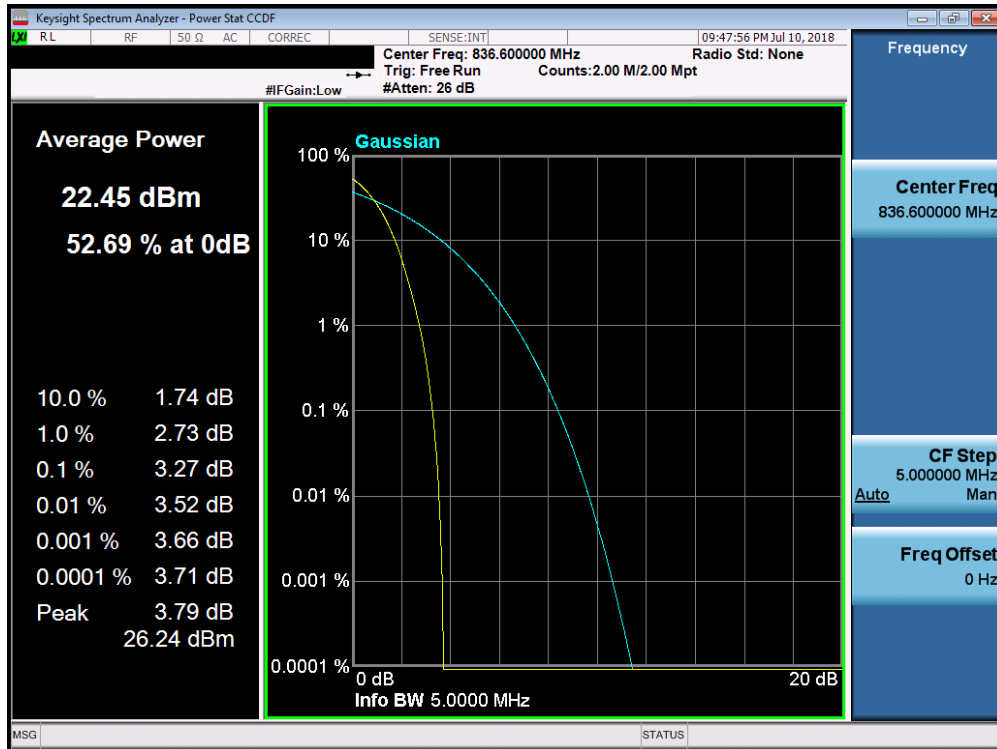
Plot 7-41. Peak-Average Ratio Plot (Cell WCDMA Mode)
