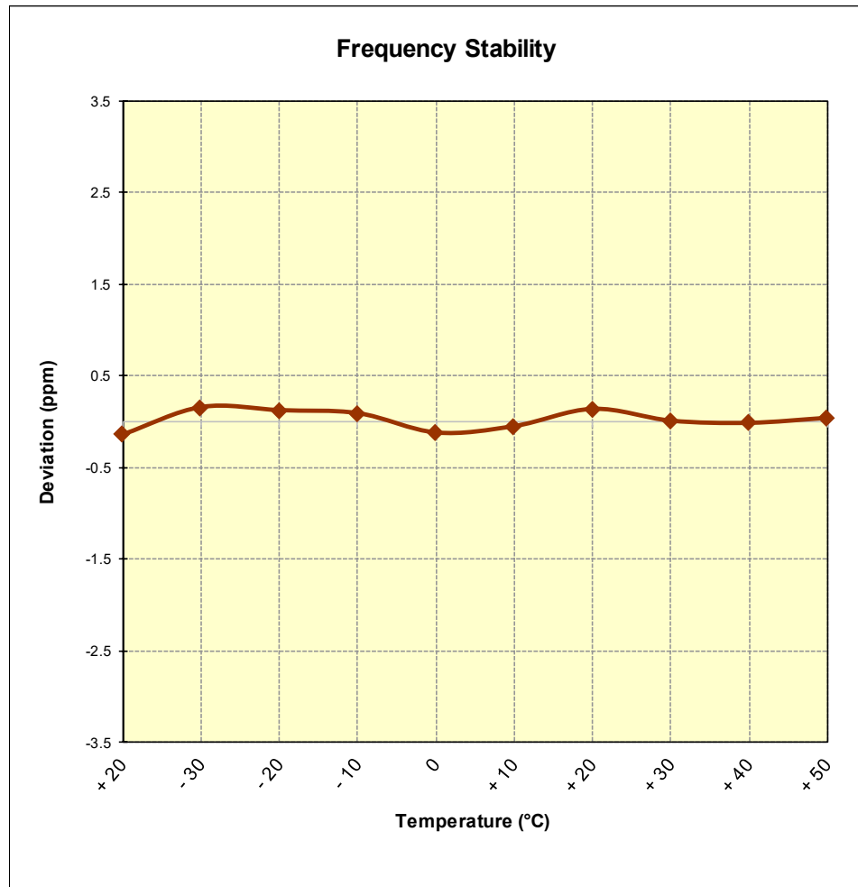
Figure 7-9. Frequency Stability Graph (PCS WCDMA Mode – Ch. 1413)
