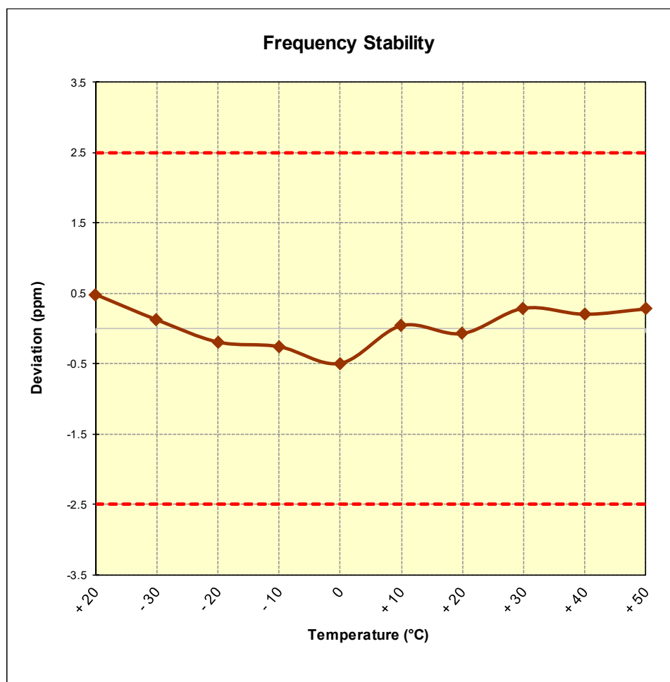
Figure 7-8. Frequency Stability Graph (Cellular WCDMA Mode – Ch. 4183)
