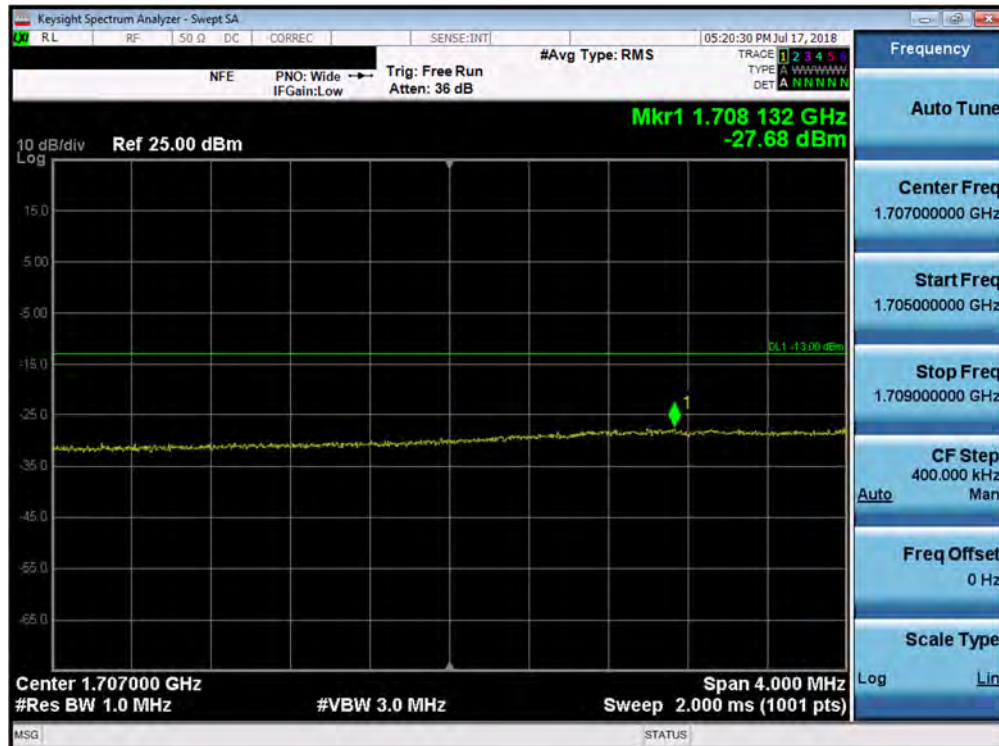
Plot 7-155. Lower Extended Band Edge Plot (Band 66/4 - 15.0MHz QPSK - Full RB Configuration)
