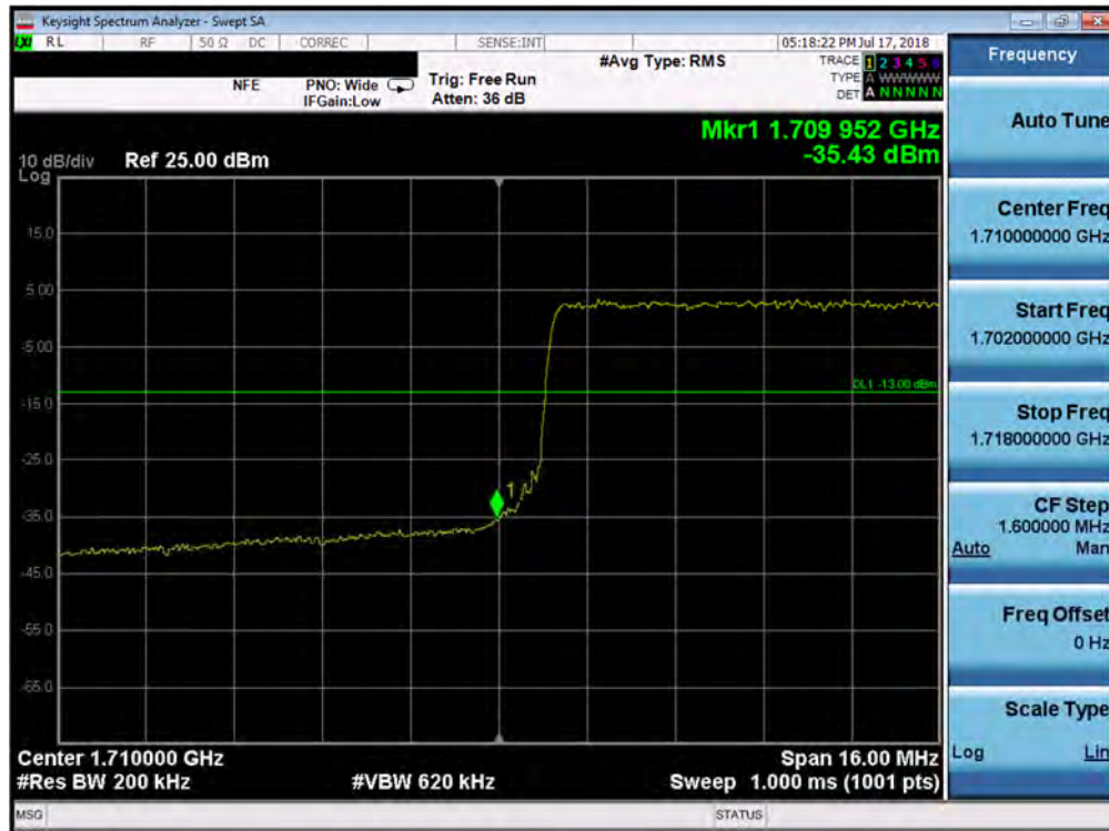
Plot 7-160. Lower Band Edge Plot (Band 66/4 - 20.0MHz QPSK - Full RB Configuration)
