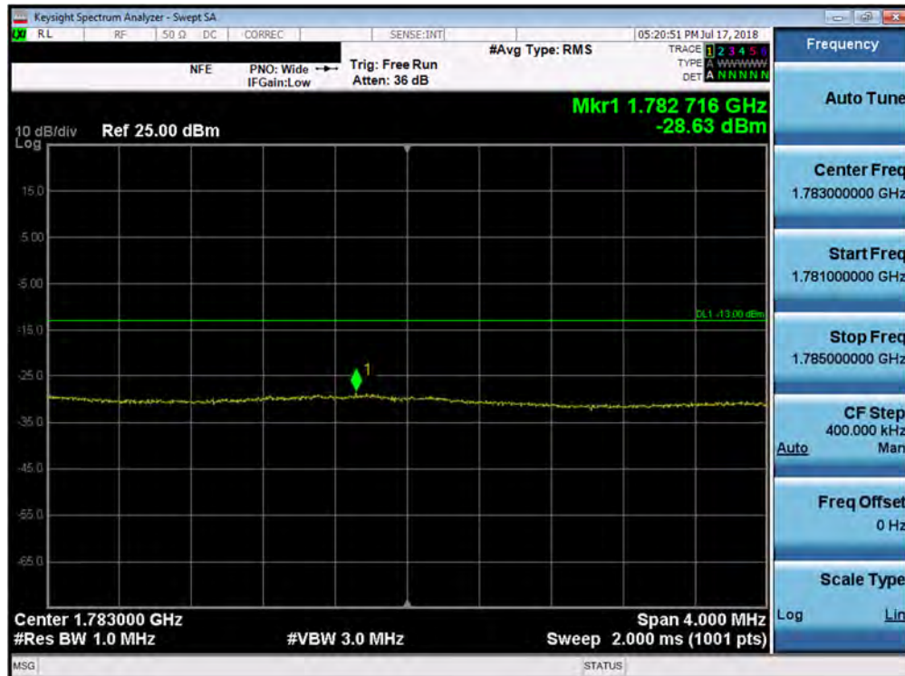
Plot 7-159. Upper Extended Band Edge Plot (Band 66 - 15.0MHz QPSK - Full RB Configuration)
