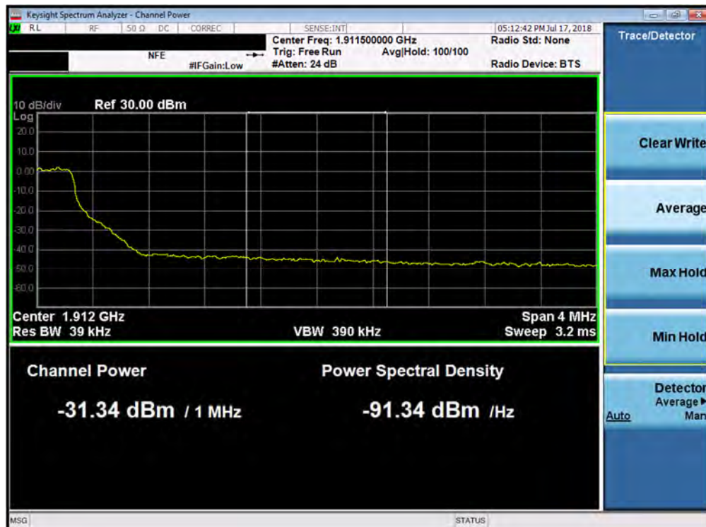
Plot 7-177. Upper Extended Band Edge Plot (Band 2 - 5.0MHz QPSK - Full RB Configuration)
