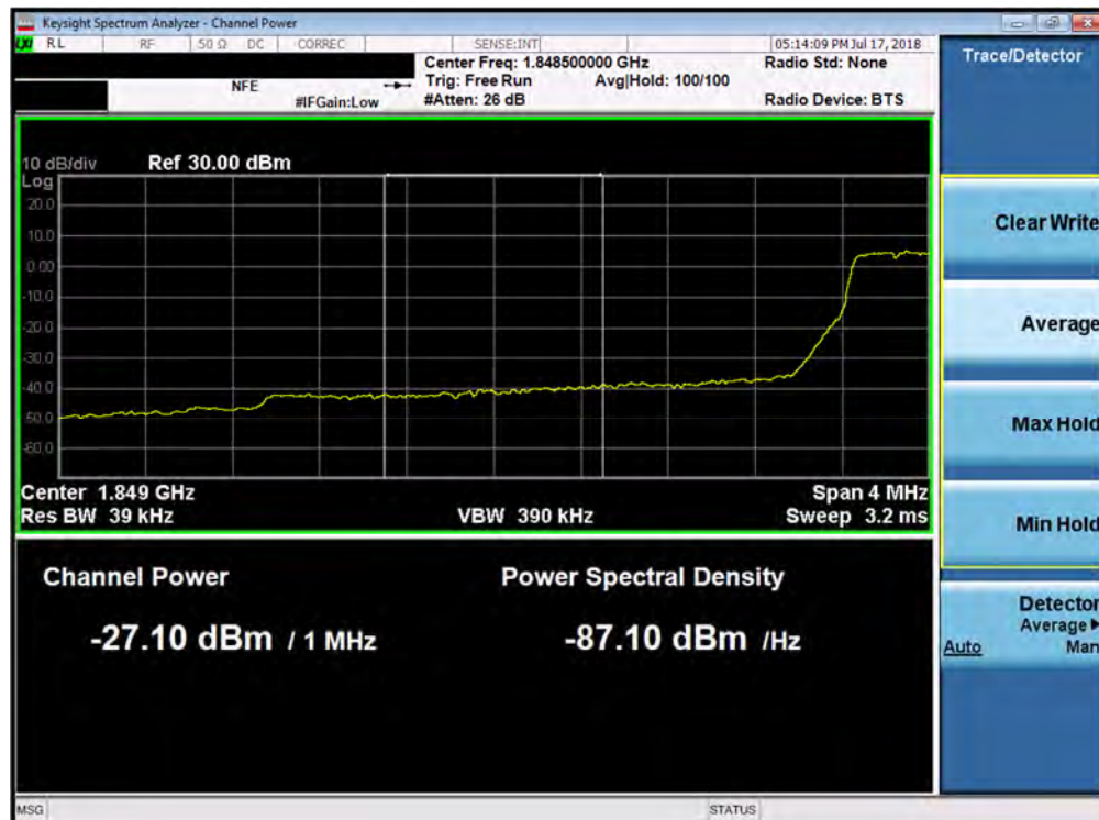
Plot 7-171. Lower Extended Band Edge Plot (Band 2 - 3.0MHz QPSK - Full RB Configuration)
