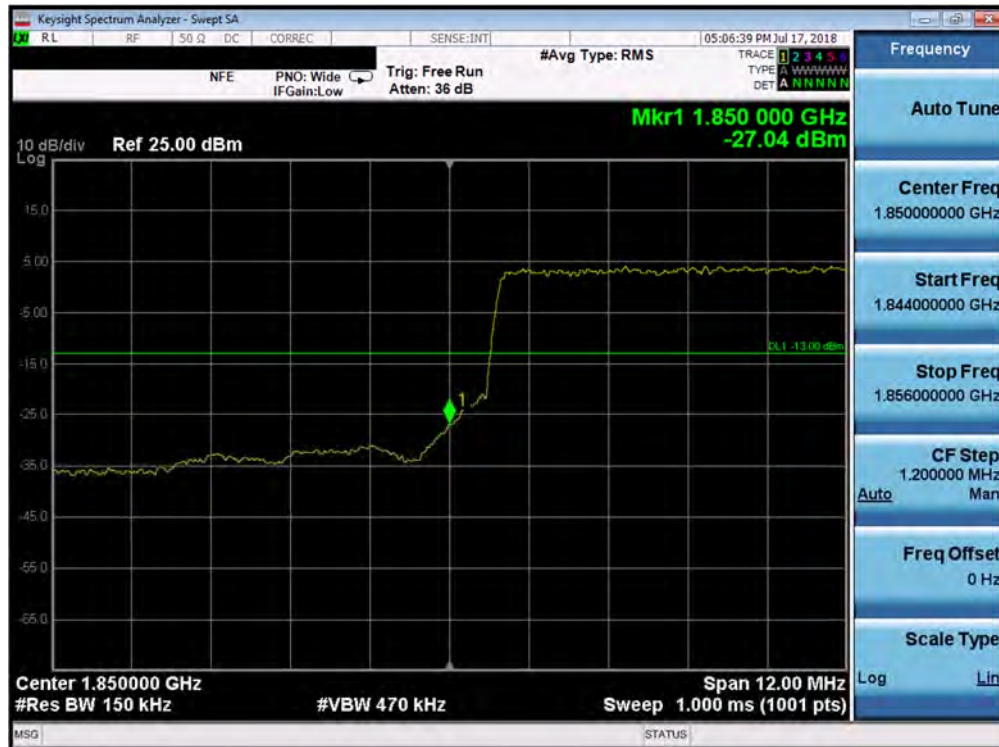
Plot 7-182. Lower Band Edge Plot (Band 2 - 15.0MHz QPSK - Full RB Configuration)
