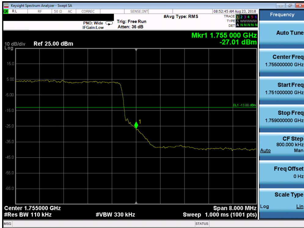
Plot 7-150. Upper Band Edge Plot (Band 4 - 10.0MHz QPSK - Full RB Configuration)
