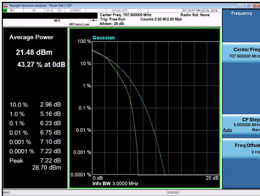
Plot 7-201. PAR Plot (Band 12 – 3.0MHz 16-QAM - Full RB Configuration)
