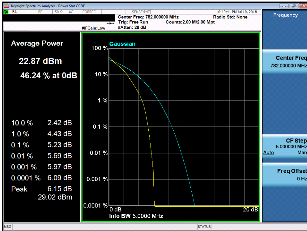
Plot 7-206. PAR Plot (Band 13 – 5.0MHz QPSK - Full RB Configuration)
