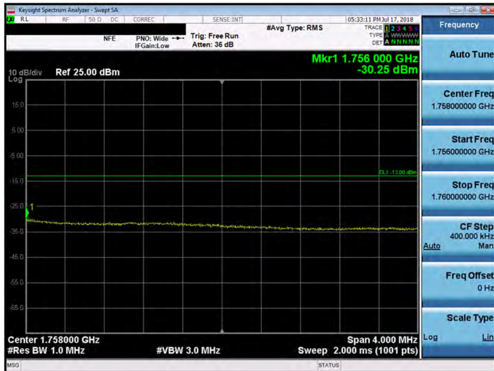
Plot 7-163. Upper Extended Band Edge Plot (Band 4 - 20.0MHz QPSK - Full RB Configuration)
