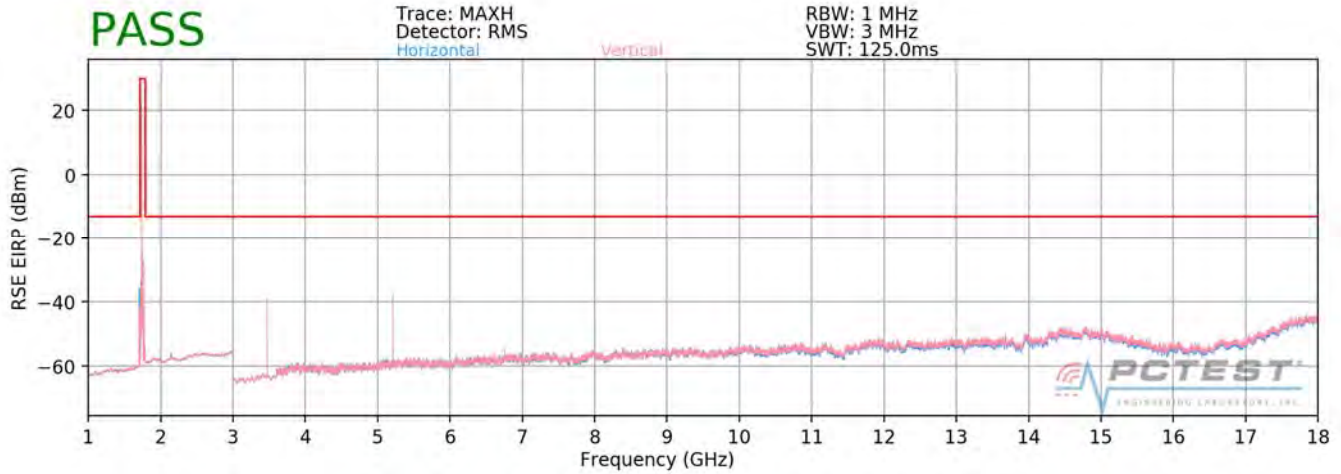
Plot 7-253. Radiated Spurious Plot above 1GHz (Band 66/4)
