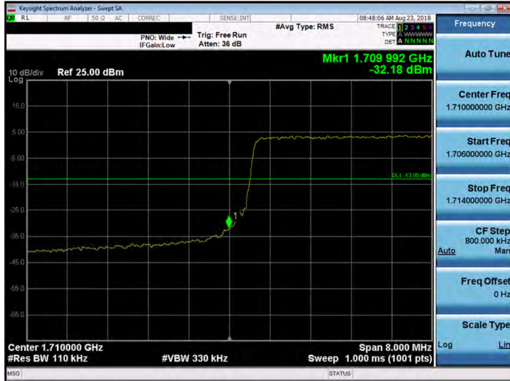
Plot 7-148. Lower Band Edge Plot (Band 66/4 - 10.0MHz QPSK - Full RB Configuration)
