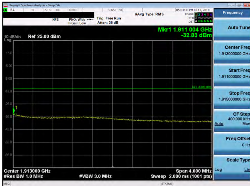
Plot 7-189. Upper Extended Band Edge Plot (Band 2 - 20.0MHz QPSK - Full RB Configuration)
