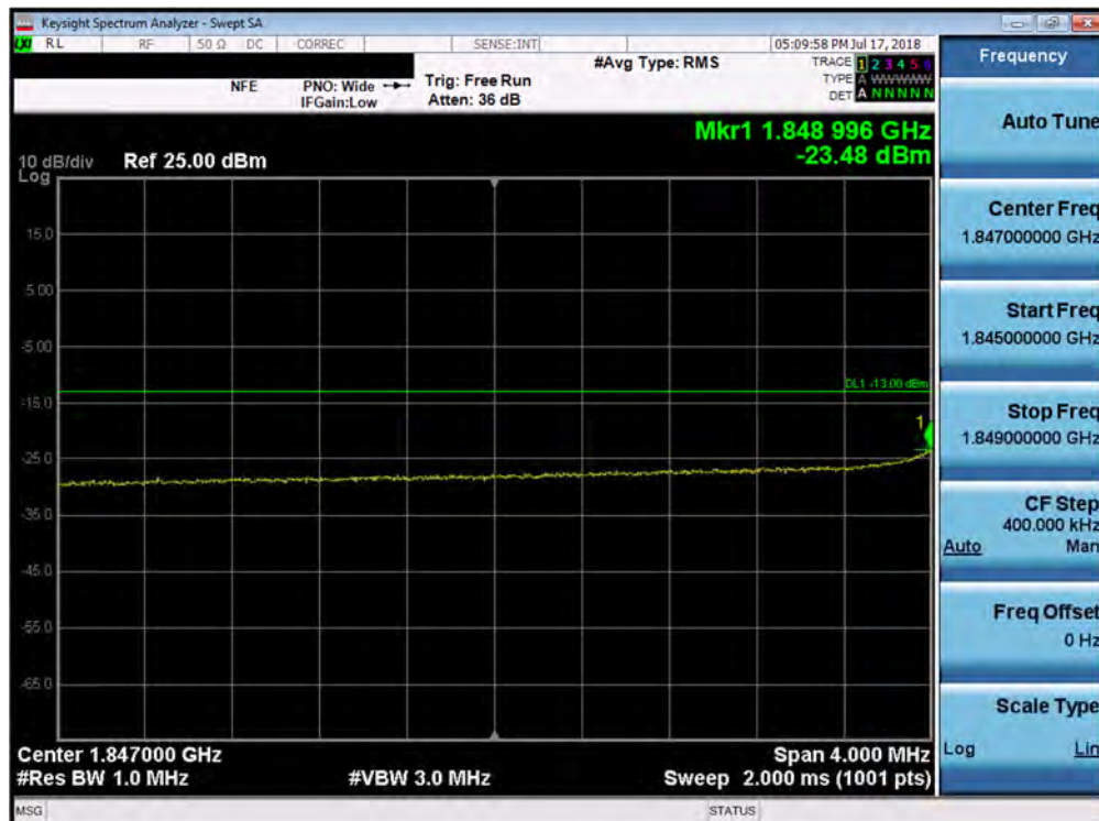
Plot 7-179. Lower Extended Band Edge Plot (Band 2 - 10.0MHz QPSK - Full RB Configuration)
