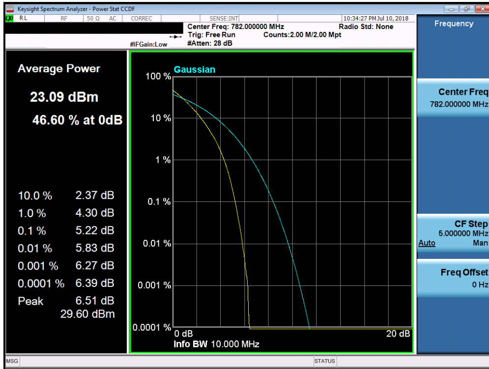
Plot 7-208. PAR Plot (Band 13 – 10.0MHz QPSK - Full RB Configuration)
