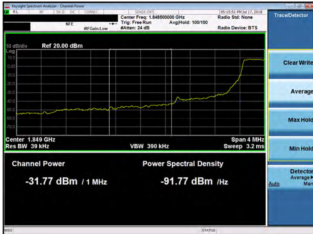
Plot 7-167. Lower Extended Band Edge Plot (Band 2 - 1.4MHz QPSK - Full RB Configuration)
