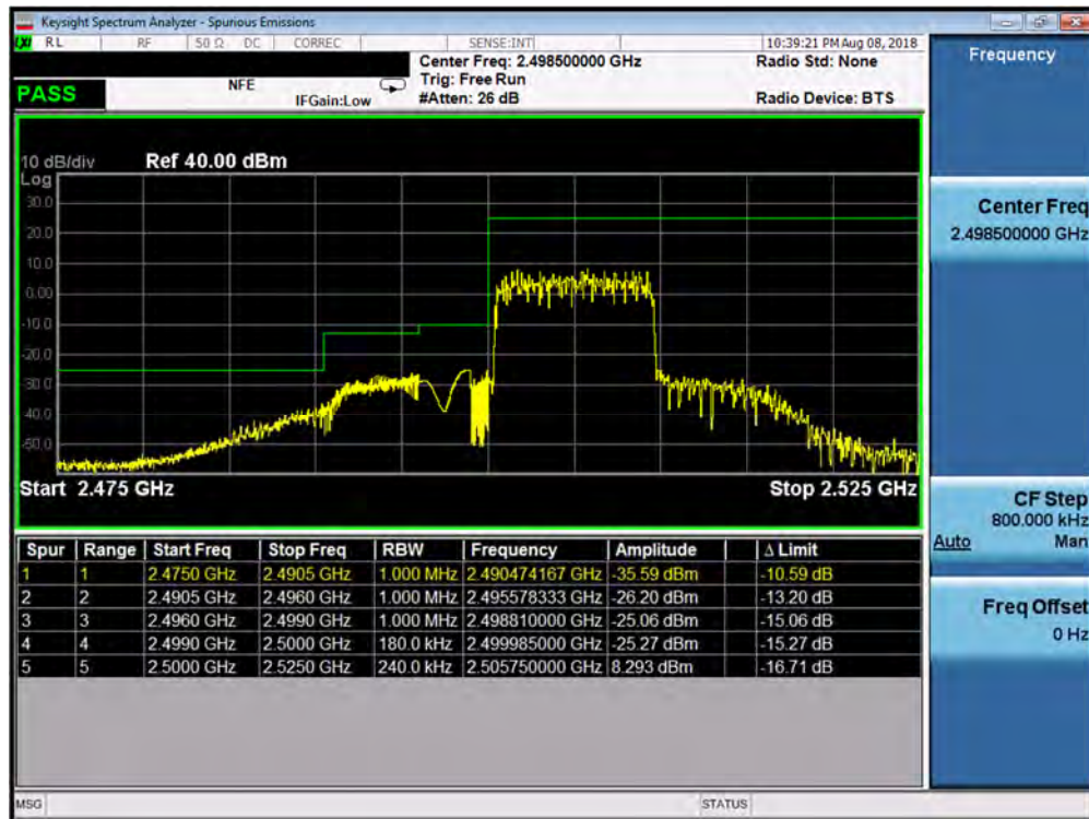
Plot 7-192. Lower ACP Plot (Band 7 - 10.0MHz QPSK - RB Size 50)
