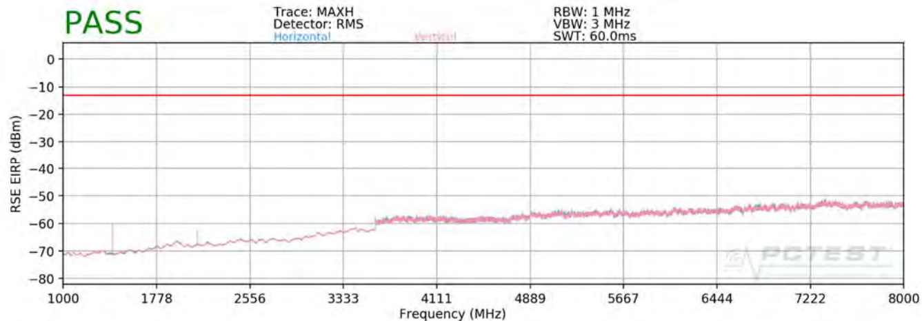
Plot 7-250. Radiated Spurious Plot above 1GHz (Band 12)
