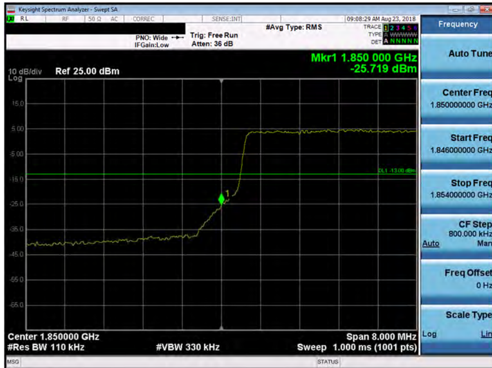
Plot 7-178. Lower Band Edge Plot (Band 2 - 10.0MHz QPSK - Full RB Configuration)
