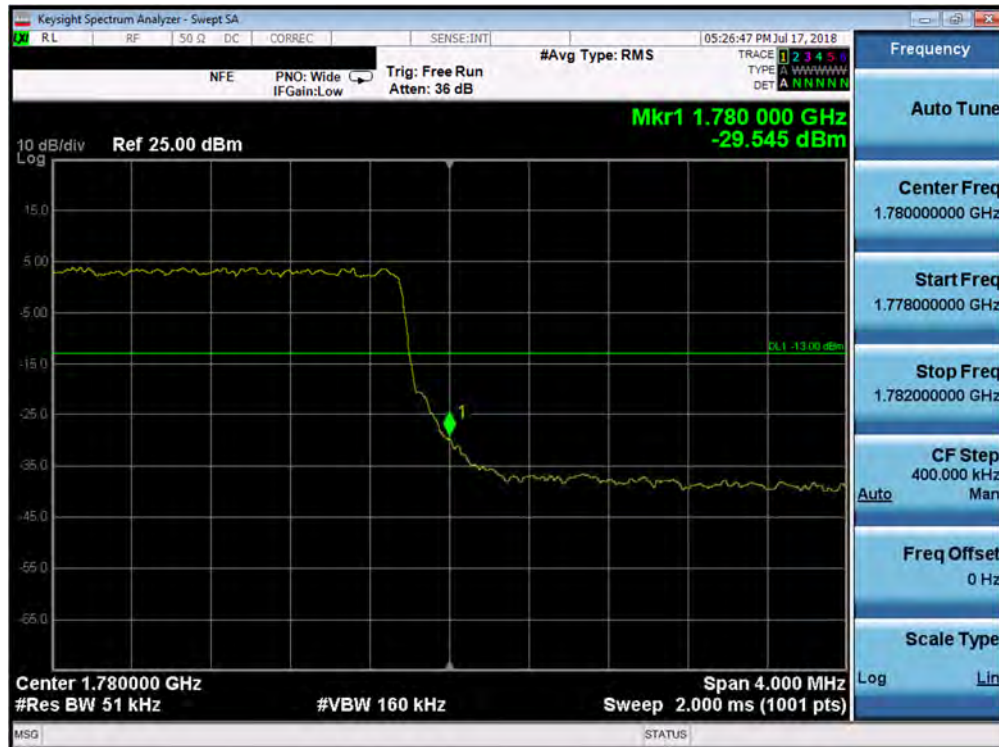
Plot 7-146. Upper Band Edge Plot (Band 66 - 5.0MHz QPSK - Full RB Configuration)
