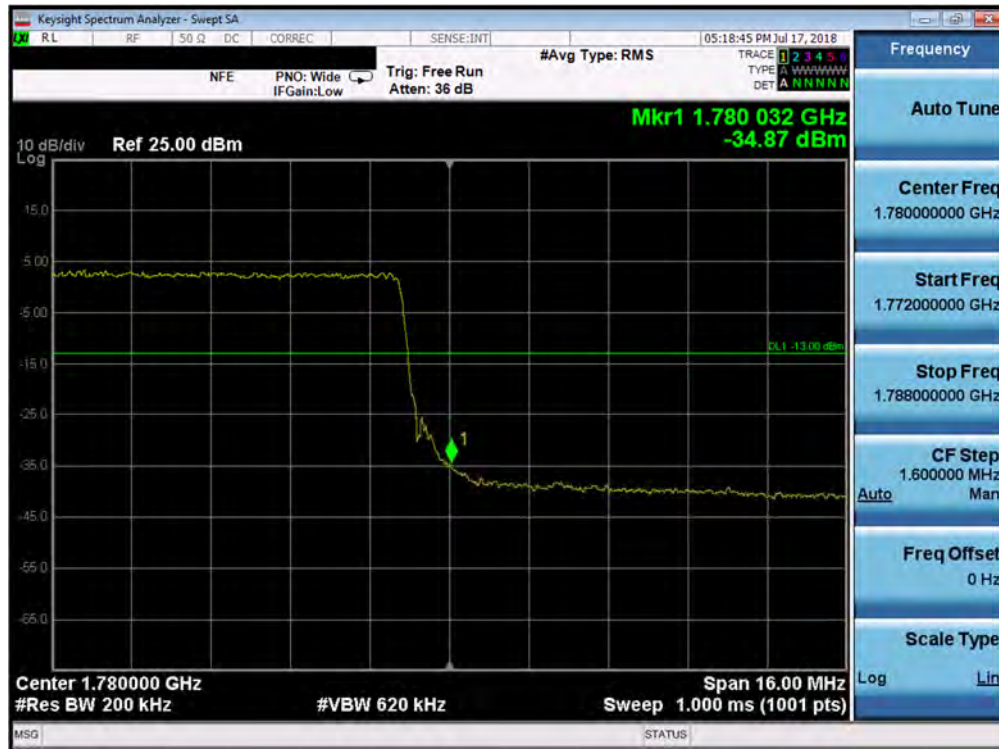
Plot 7-164. Upper Band Edge Plot (Band 66 - 20.0MHz QPSK - Full RB Configuration)
