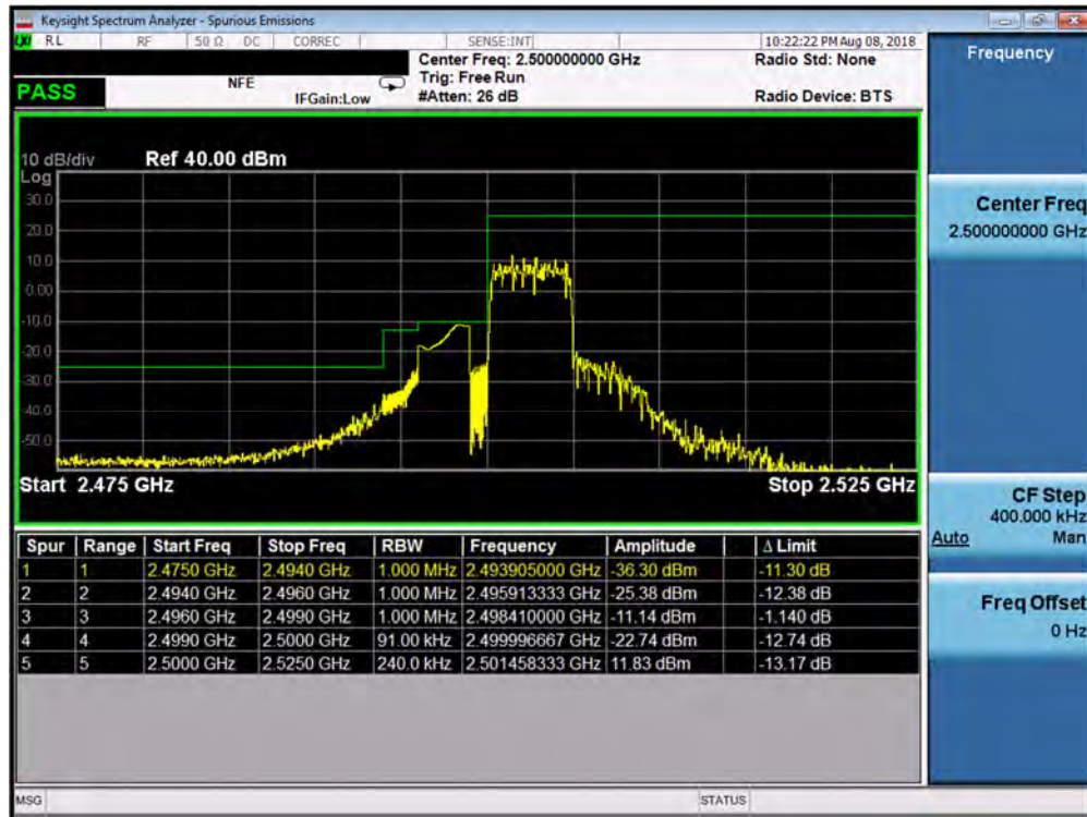
Plot 7-190. Lower ACP Plot (Band 7 - 5.0MHz QPSK - RB Size 25)
