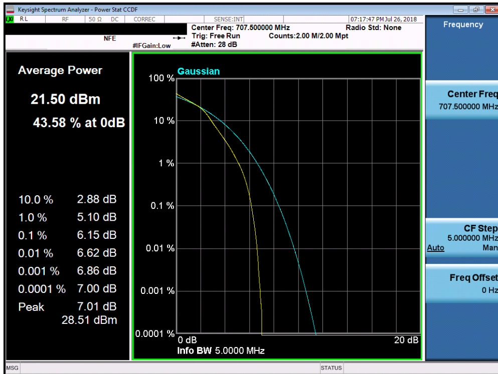
Plot 7-203. PAR Plot (Band 12 – 5.0MHz 16-QAM - Full RB Configuration)
