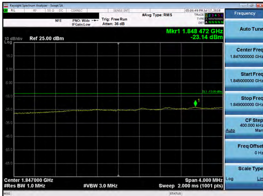
Plot 7-183. Lower Extended Band Edge Plot (Band 2 - 15.0MHz QPSK - Full RB Configuration)
