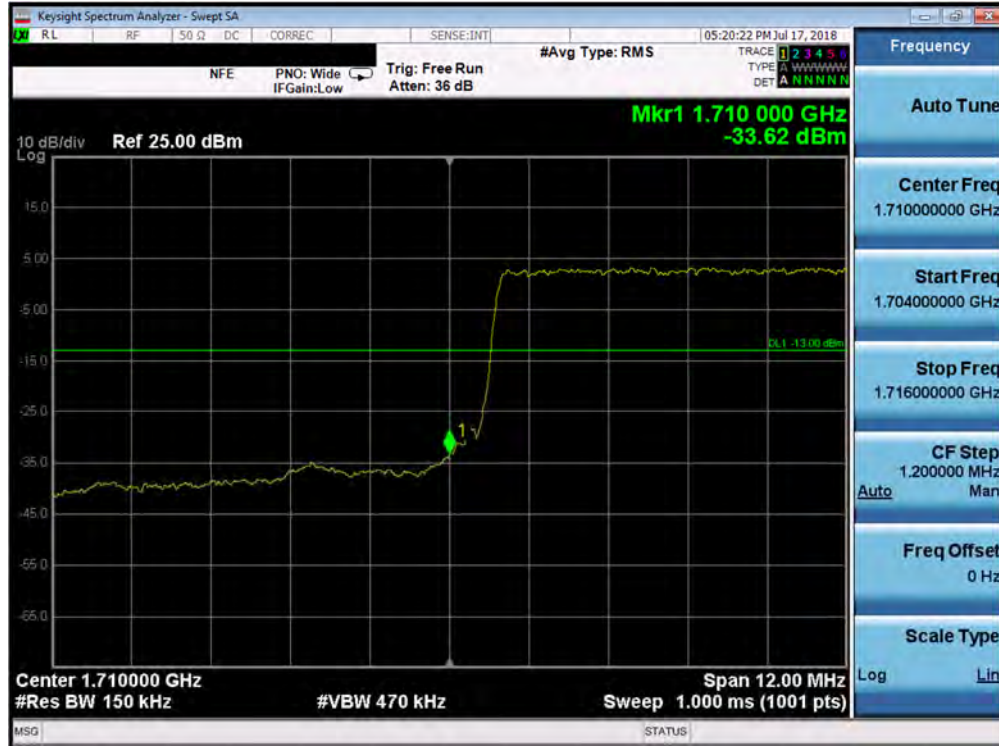
Plot 7-154. Lower Band Edge Plot (Band 66/4 - 15.0MHz QPSK - Full RB Configuration)
