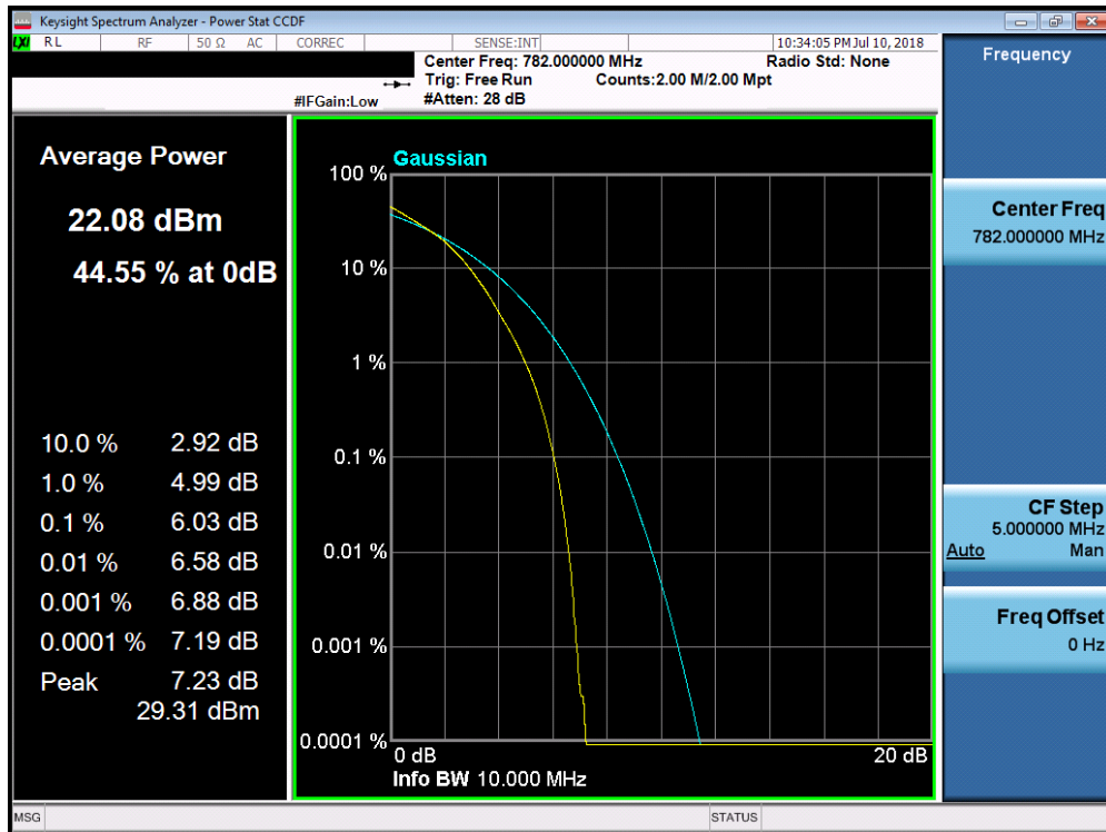
Plot 7-209. PAR Plot (Band 13 – 10.0MHz 16-QAM - Full RB Configuration)
