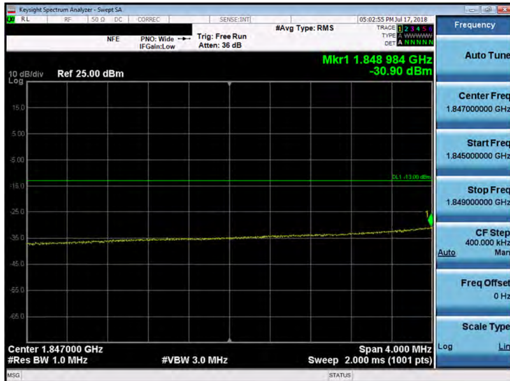
Plot 7-187. Lower Extended Band Edge Plot (Band 2 - 20.0MHz QPSK - Full RB Configuration)
