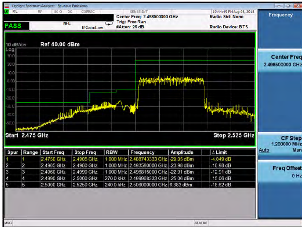
Plot 7-194. Lower ACP Plot (Band 7 - 15.0MHz QPSK - RB Size 75)
