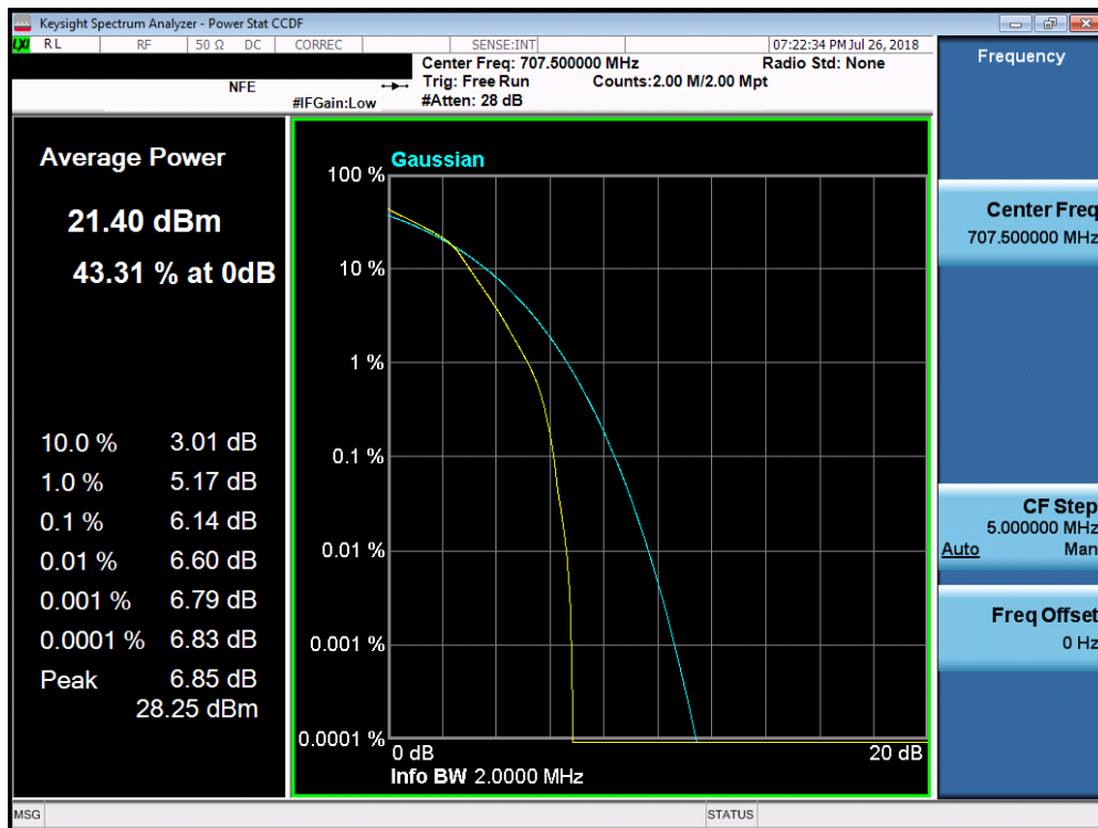
Plot 7-199. PAR Plot (Band 12 - 1.4MHz 16-QAM - Full RB Configuration)
