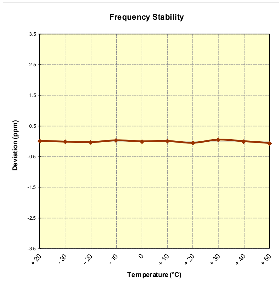
Figure 7-11. Frequency Stability Graph (Band 66/4)
