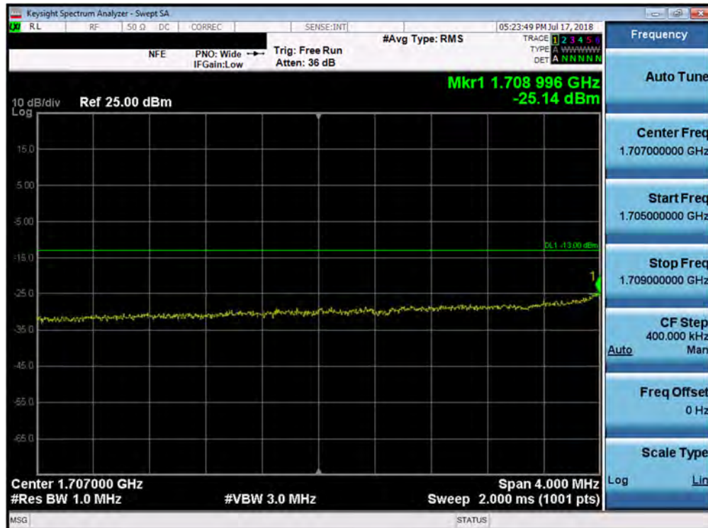
Plot 7-149. Lower Extended Band Edge Plot (Band 66/4 - 10.0MHz QPSK - Full RB Configuration)
