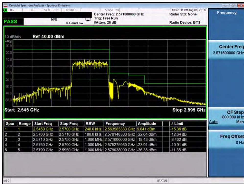
Plot 7-193. Upper ACP Plot (Band 7 - 10.0MHz QPSK - RB Size 50)
