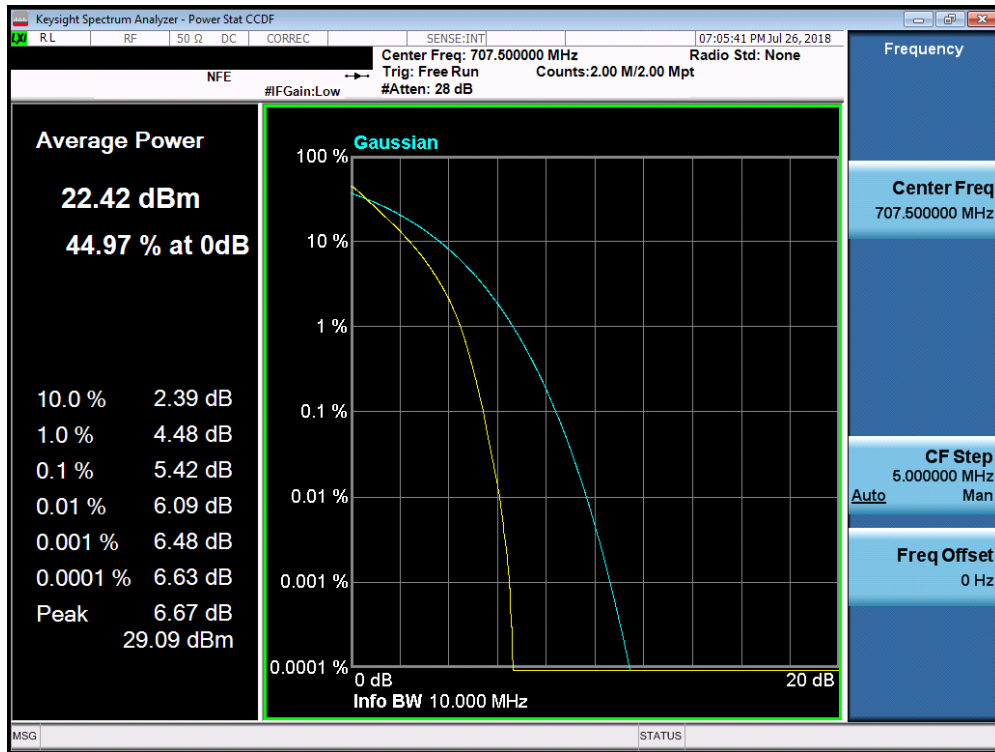
Plot 7-204. PAR Plot (Band 12 – 10.0MHz QPSK - Full RB Configuration)
