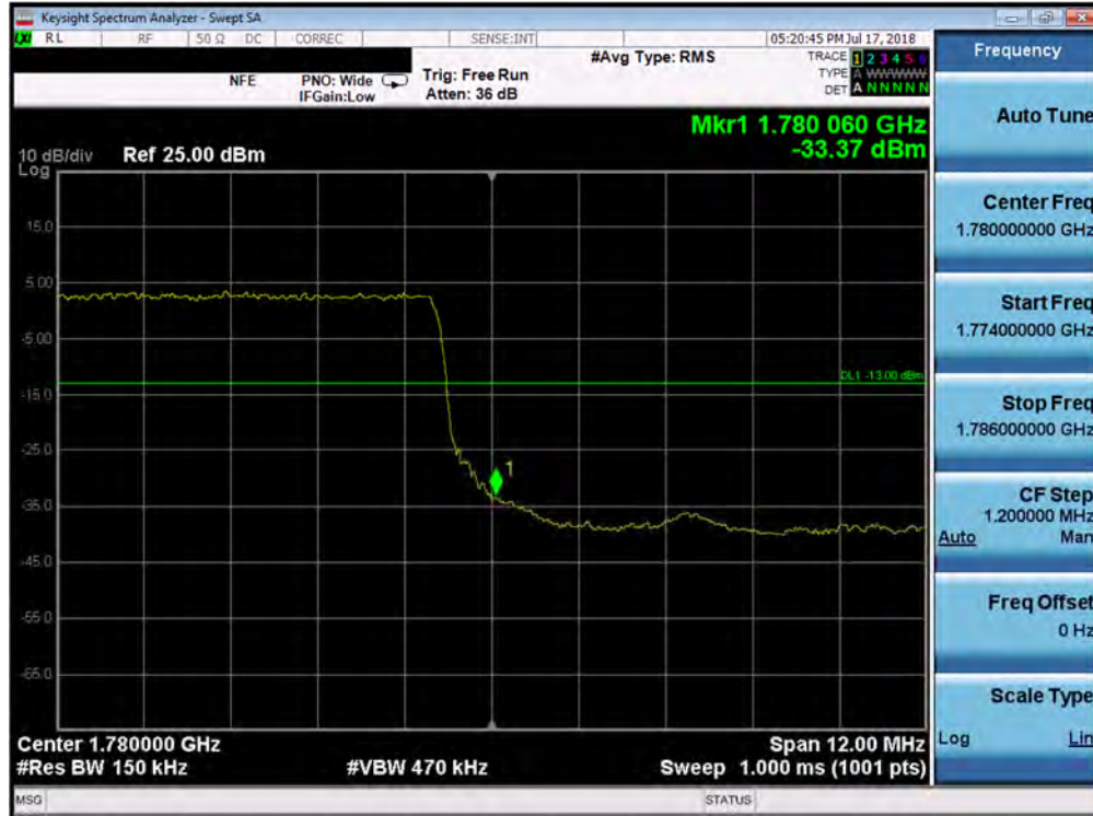
Plot 7-158. Upper Band Edge Plot (Band 66 - 15.0MHz QPSK - Full RB Configuration)
