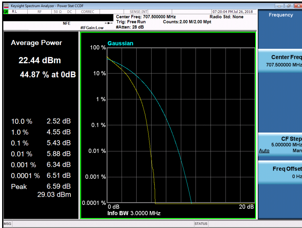
Plot 7-200. PAR Plot (Band 12 – 3.0MHz QPSK - Full RB Configuration)
