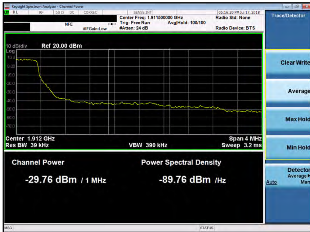
Plot 7-169. Upper Extended Band Edge Plot (Band 2 - 1.4MHz QPSK - Full RB Configuration)
