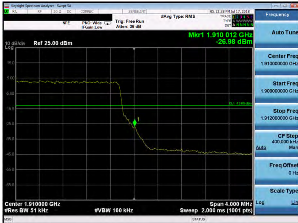
Plot 7-176. Upper Band Edge Plot (Band 2 - 5.0MHz QPSK - Full RB Configuration)
