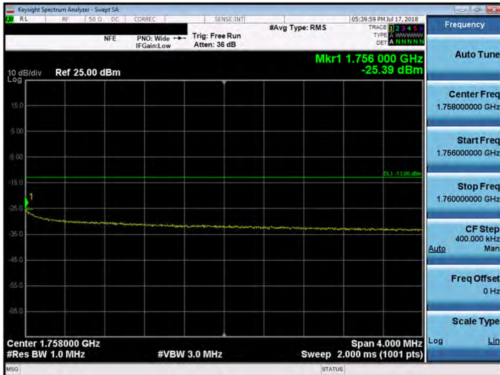
Plot 7-151. Upper Extended Band Edge Plot (Band 4 - 10.0MHz QPSK - Full RB Configuration)
