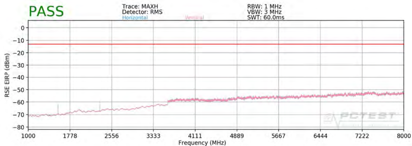
Plot 7-251. Radiated Spurious Plot above 1GHz (Band 13)
