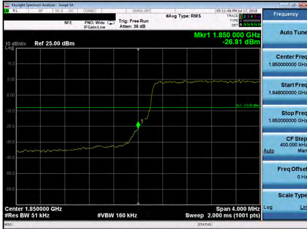
Plot 7-174. Lower Band Edge Plot (Band 2 - 5.0MHz QPSK - Full RB Configuration)
