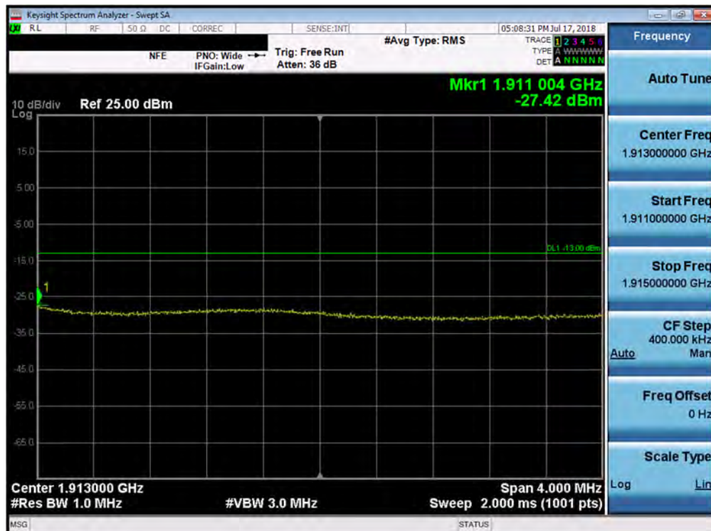
Plot 7-185. Upper Extended Band Edge Plot (Band 2 - 15.0MHz QPSK - Full RB Configuration)
