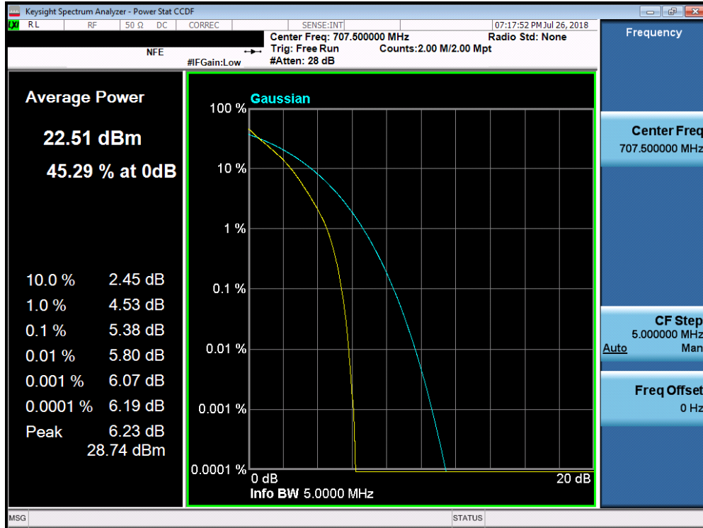
Plot 7-202. PAR Plot (Band 12 – 5.0MHz QPSK - Full RB Configuration)
