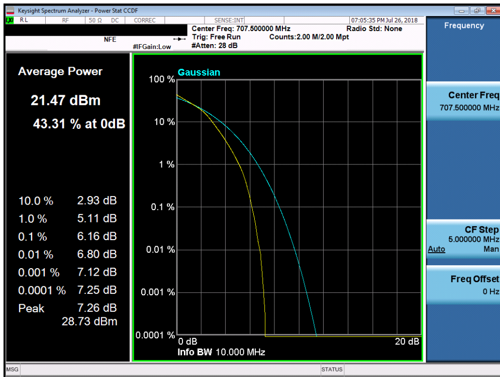
Plot 7-205. PAR Plot (Band 12 – 10.0MHz 16-QAM - Full RB Configuration)
