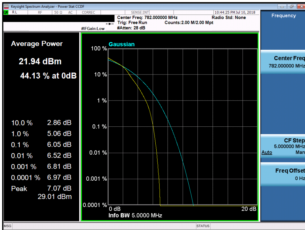
Plot 7-207. PAR Plot (Band 13 – 5.0MHz 16-QAM - Full RB Configuration)
