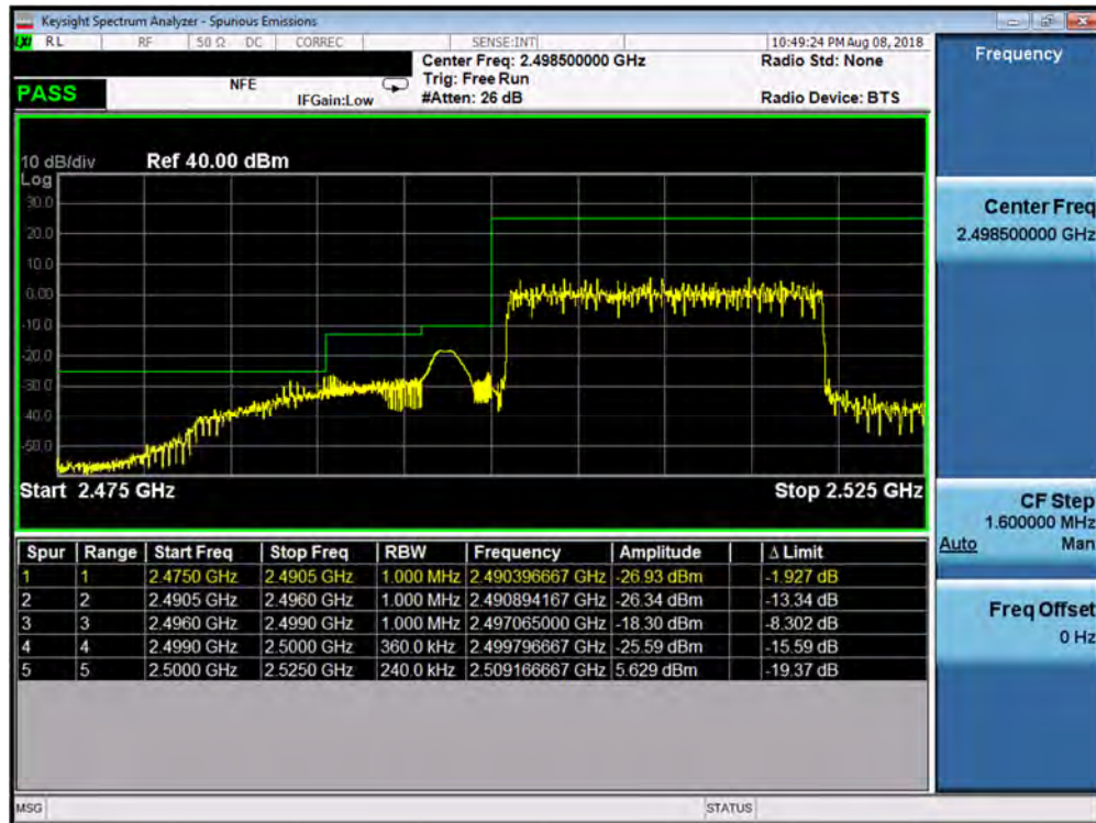
Plot 7-196. Lower ACP Plot (Band 7 - 20.0MHz QPSK - RB Size 100)
