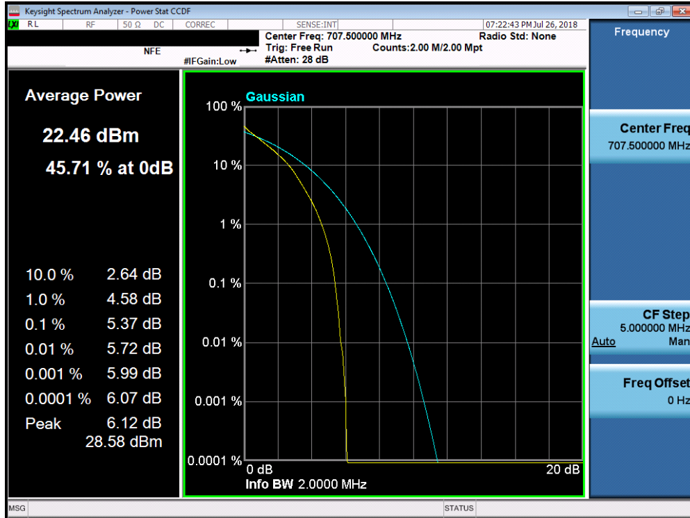
Plot 7-198. PAR Plot (Band 12 - 1.4MHz QPSK - Full RB Configuration)
