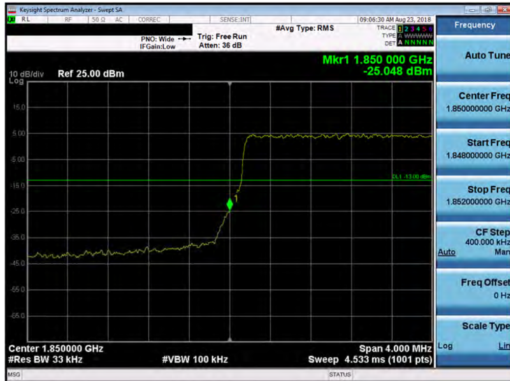
Plot 7-170. Lower Band Edge Plot (Band 2 - 3.0MHz QPSK - Full RB Configuration)
