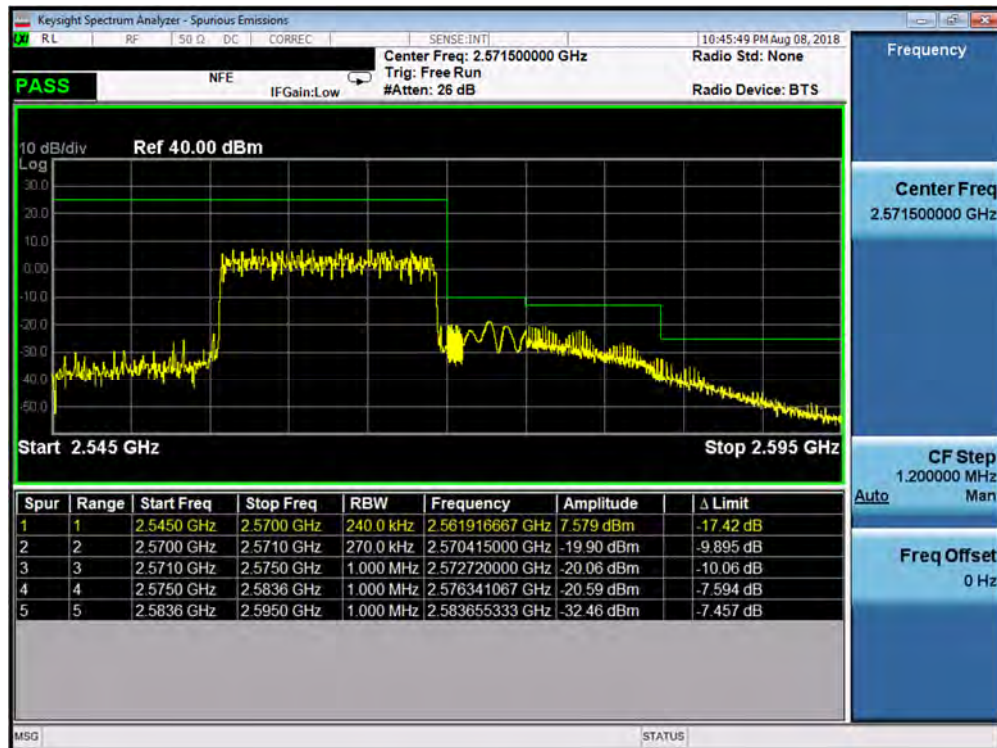
Plot 7-195. Upper ACP Plot (Band 7 - 15.0MHz QPSK - RB Size 75)
