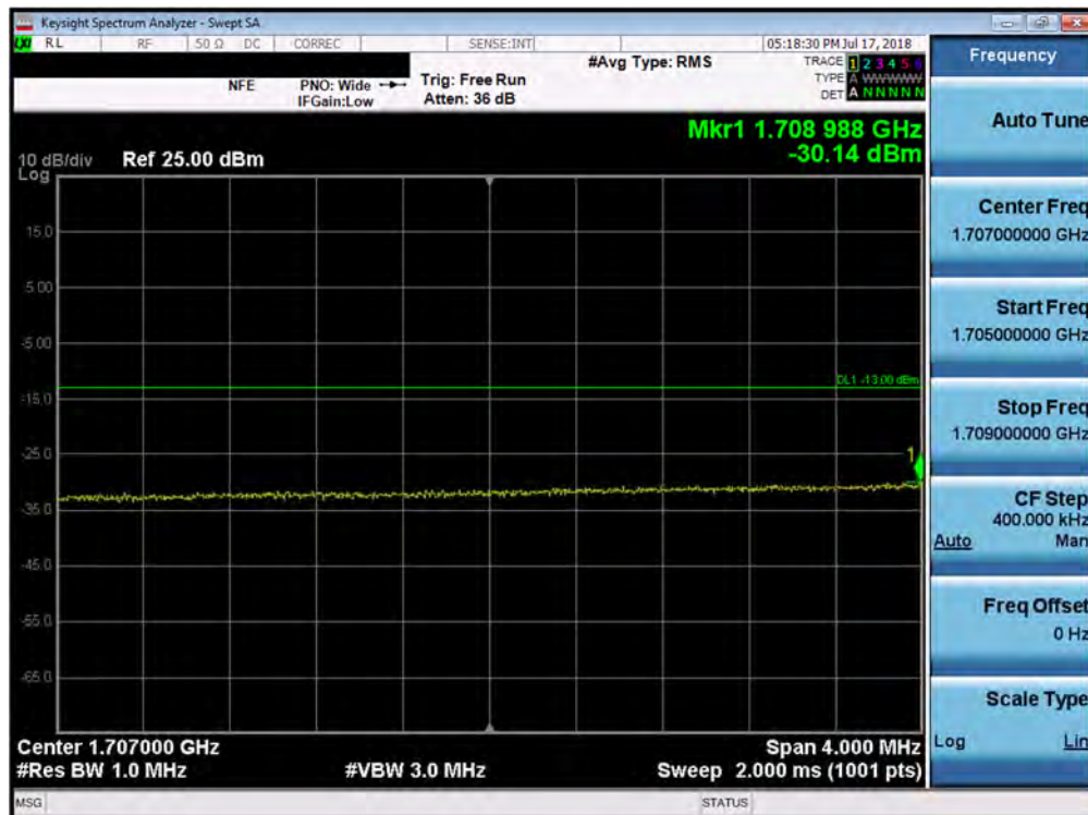
Plot 7-161. Lower Extended Band Edge Plot (Band 66/4 - 20.0MHz QPSK - Full RB Configuration)
