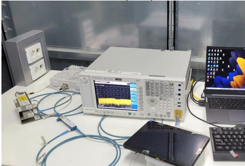
LICENSED BAND TEST PHOTO(CBRS)
