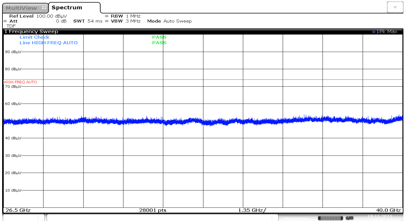
Plot 7-88. Radiated Spurious Plot above 26.5GHz (802.11a – Ant. Pol. H)
