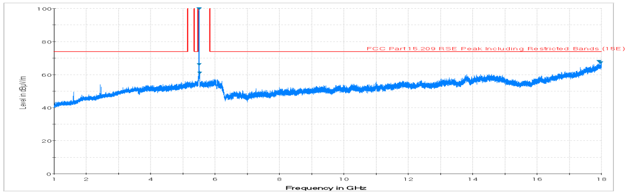
Plot 7-84. Radiated Spurious Plot above 1GHz (802.11a – U2C Ch. 116, Ant. Pol. V)
