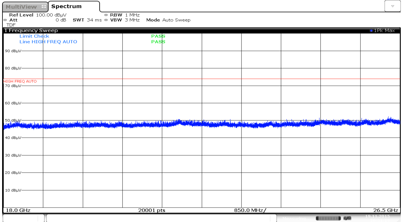
Plot 7-89. Radiated Spurious Plot above 18GHz (802.11a – Ant. Pol. V)
