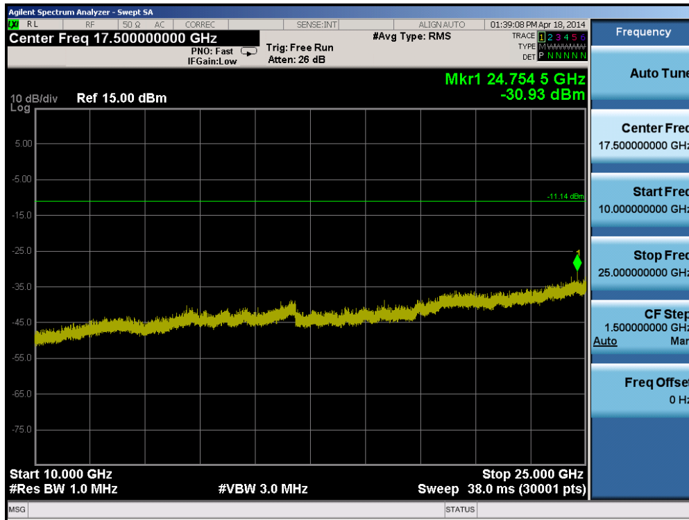
Plot 6-41. Conducted Spurious Plot (Bluetooth, 1Mbps – Ch. 78)
