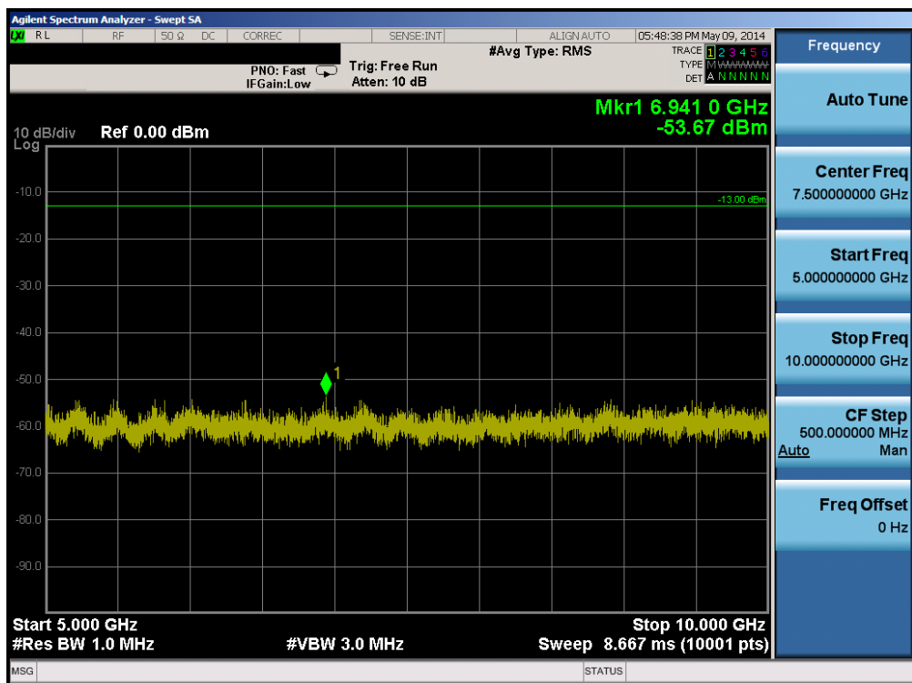
Plot 6-48. Conducted Spurious Plot (Band 17 – 10.0MHz QPSK – RB Size 1, RB Offset 0 – High Channel)
