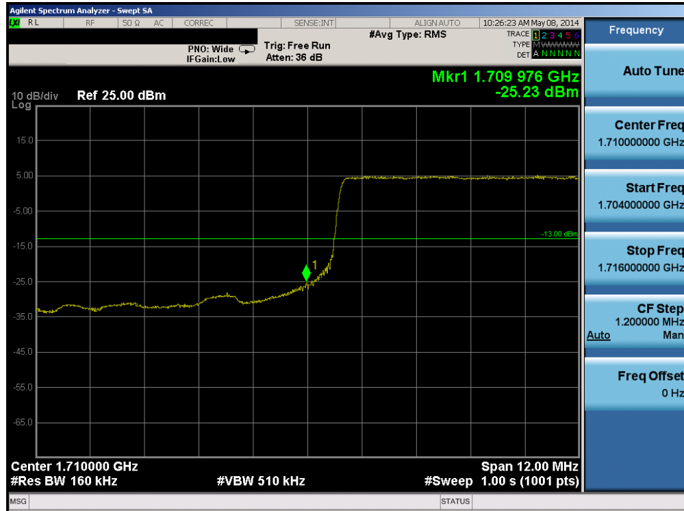
Plot 6-185. Lower Band Edge Plot (Band 4 – 15.0MHz QPSK – RB Size 75)
