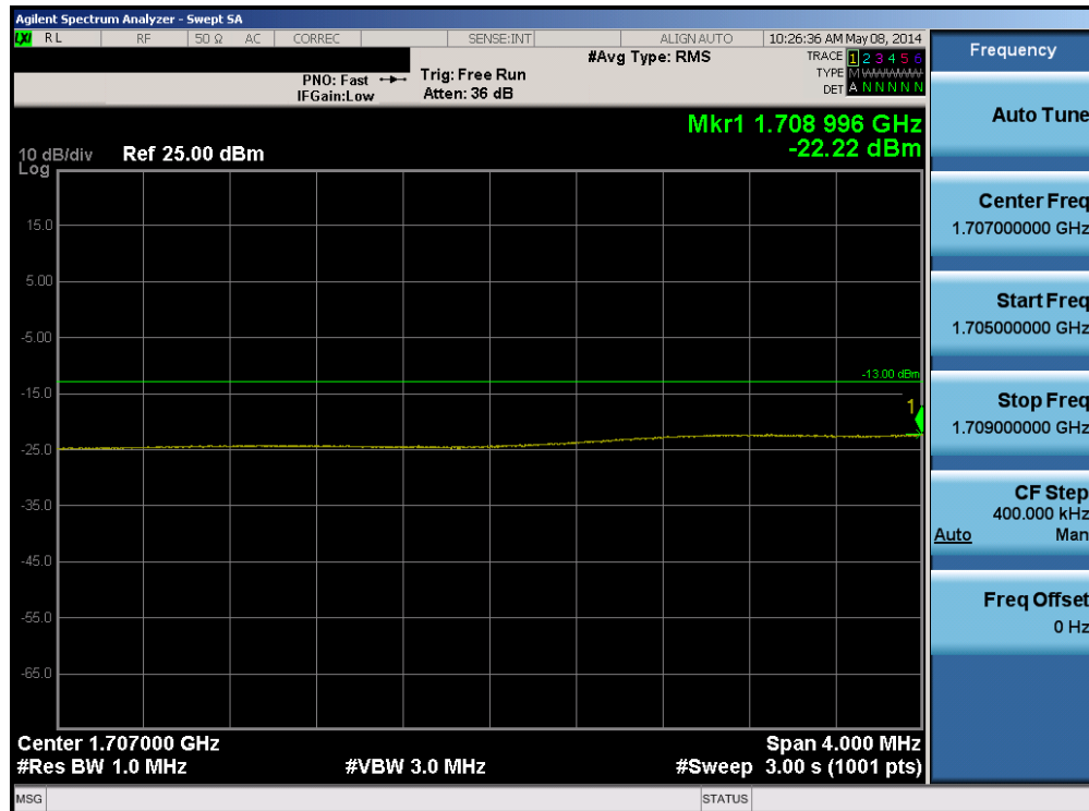
Plot 6-186. Lower Extended Band Edge Plot (Band 4 – 15.0MHz QPSK – RB Size 75)
