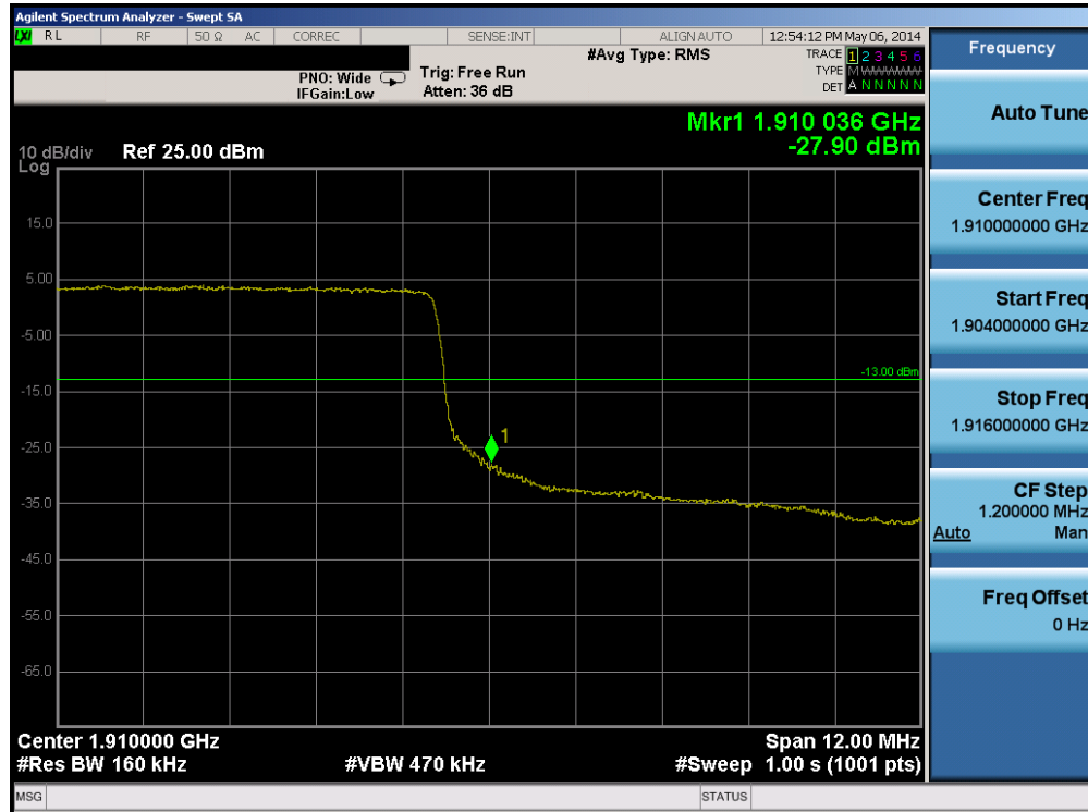
Plot 6-211. Upper Band Edge Plot (Band 2 – 15.0MHz QPSK – RB Size 75)
