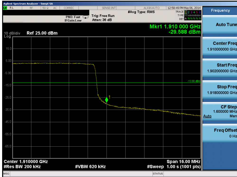
Plot 6-215. Upper Band Edge Plot (Band 2 – 20.0MHz QPSK – RB Size 100)
