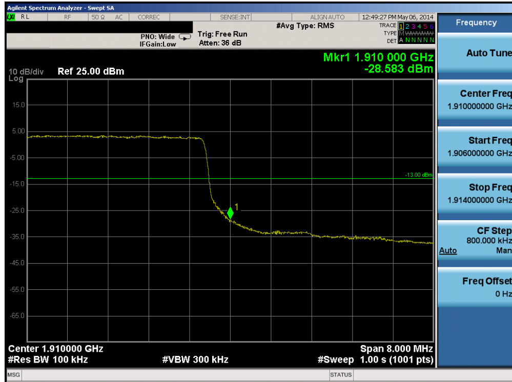
Plot 6-207. Upper Band Edge Plot (Band 2 - 10.0MHz QPSK - RB Size 50)
