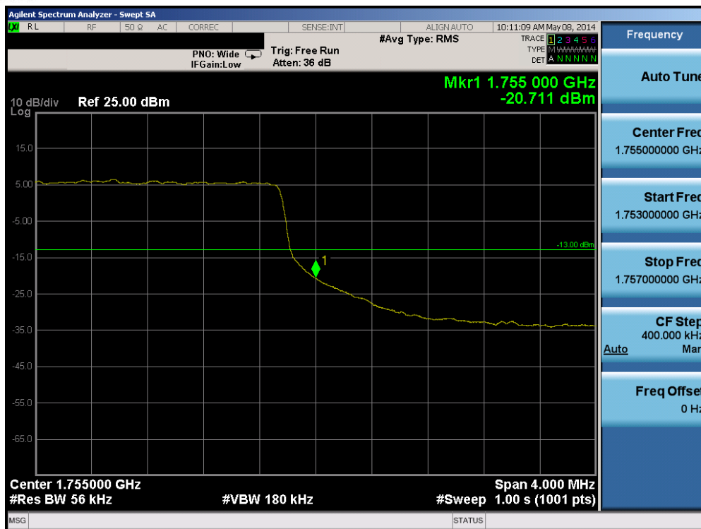
Plot 6-179. Upper Band Edge Plot (Band 4 – 5.0MHz QPSK – RB Size 25)
