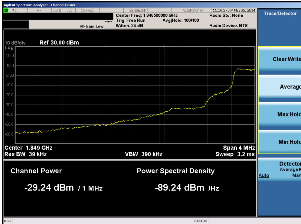
Plot 6-194. Lower Extended Band Edge Plot (Band 2 – 1.4MHz QPSK – RB Size 6)
