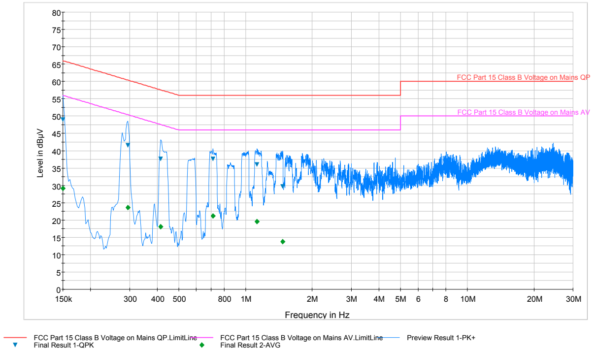
Plot 6-45. Line-Conducted Test Plot (N)
