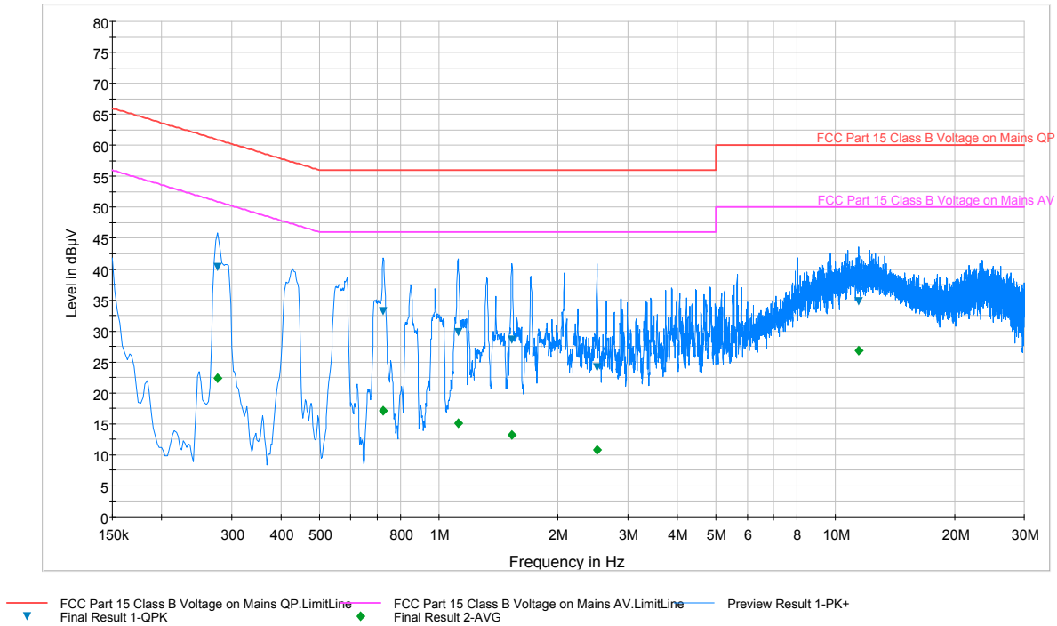
Plot 6-44. Line-Conducted Test Plot (L1)
