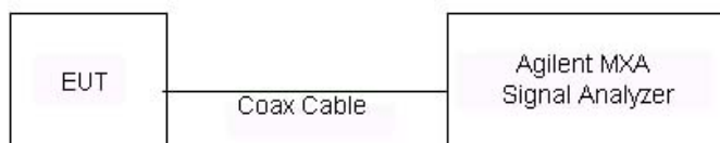
Figure 6-3. Test Instrument & Measurement Setup
