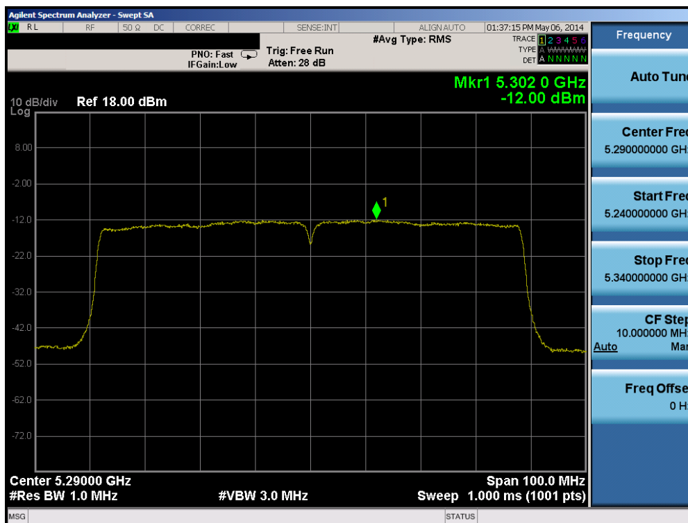
Plot 6-86. Peak Power Spectral Density Plot (80MHz BW 802.11ac (UNII Band 2A) – Ch. 58)
