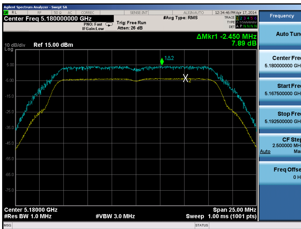
Plot 6-129. Peak Excursion Ratio Plot (802.11a (UNII Band 1) – Ch. 36)
