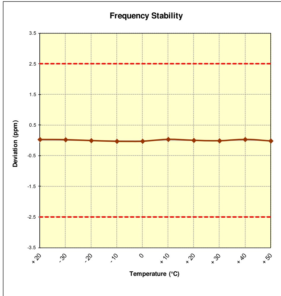
Figure 6-7. Frequency Stability Graph (Cellular GPRS Mode – Ch. 190)
