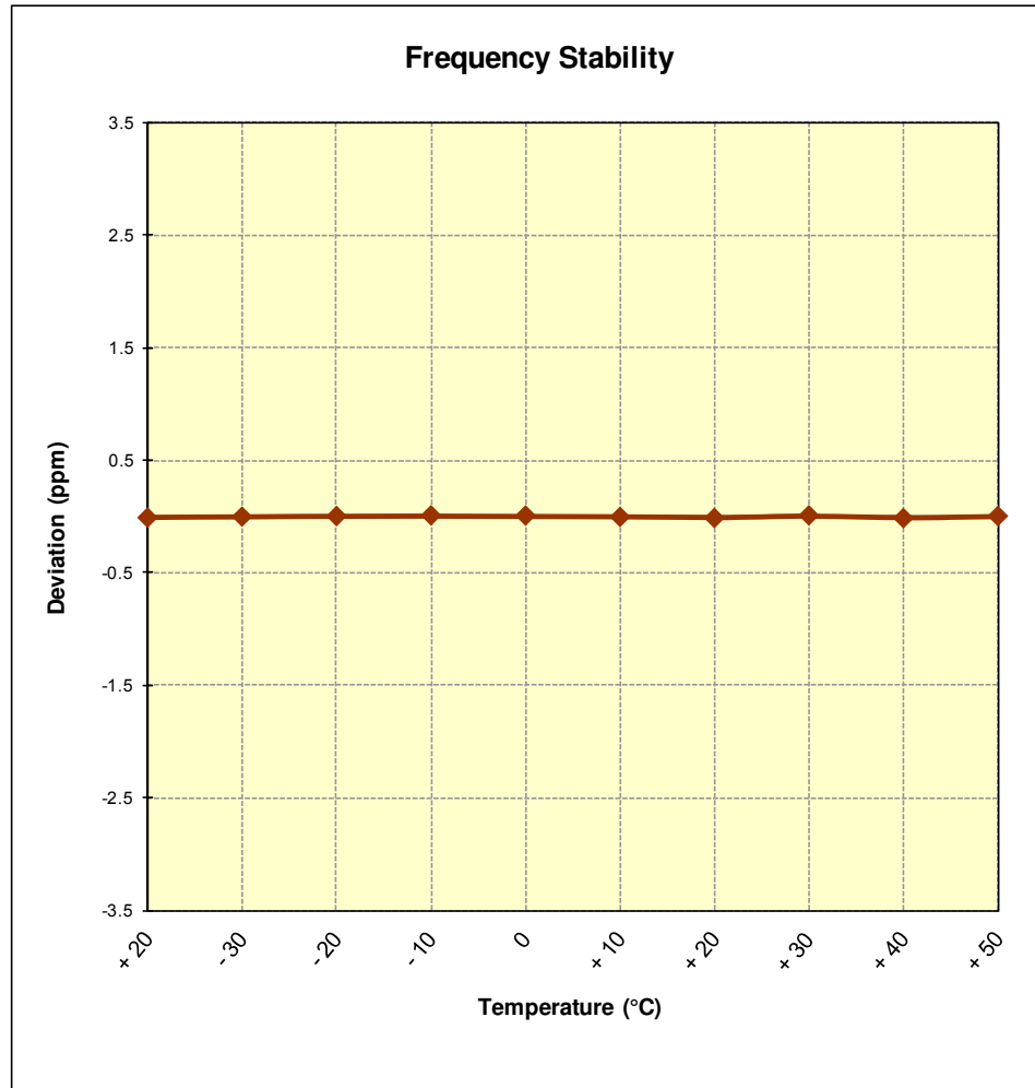
Figure 6-9. Frequency Stability Graph (PCS GPRS Mode – Ch. 661)
