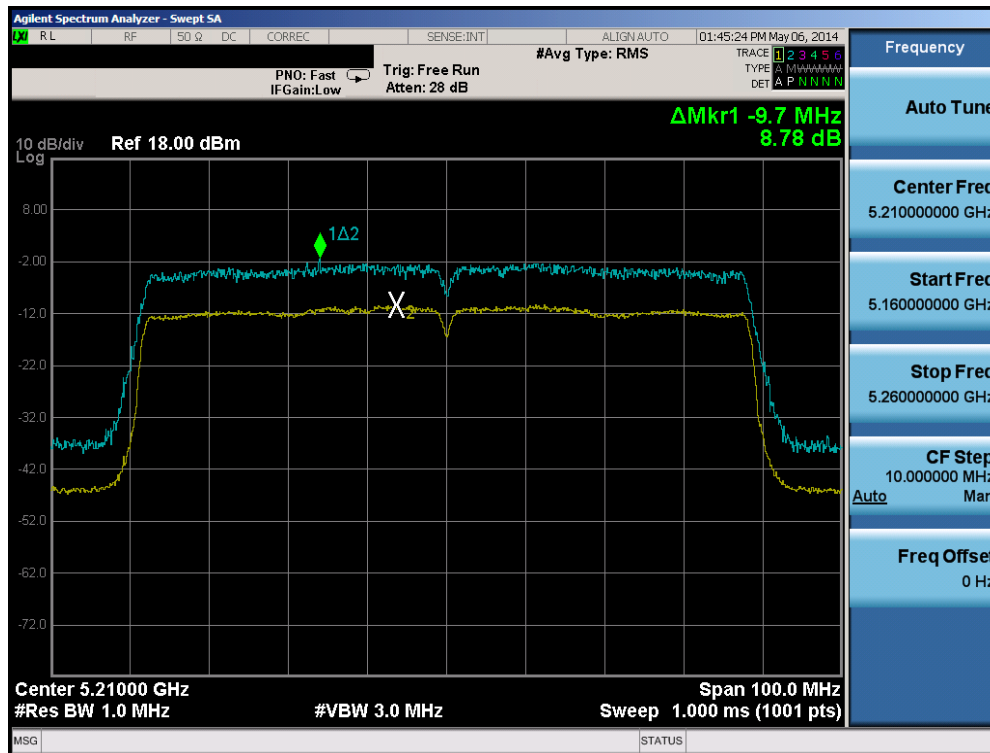
Plot 6-132. Peak Excursion Ratio Plot (80MHz BW 802.11ac (UNII Band 1) – Ch. 42)
