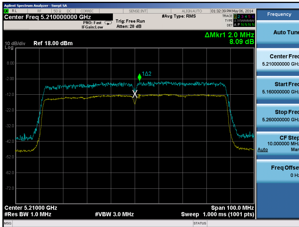
Plot 6-128. Peak Excursion Ratio Plot (80MHz BW 802.11ac (UNII Band 1) – Ch. 42)
