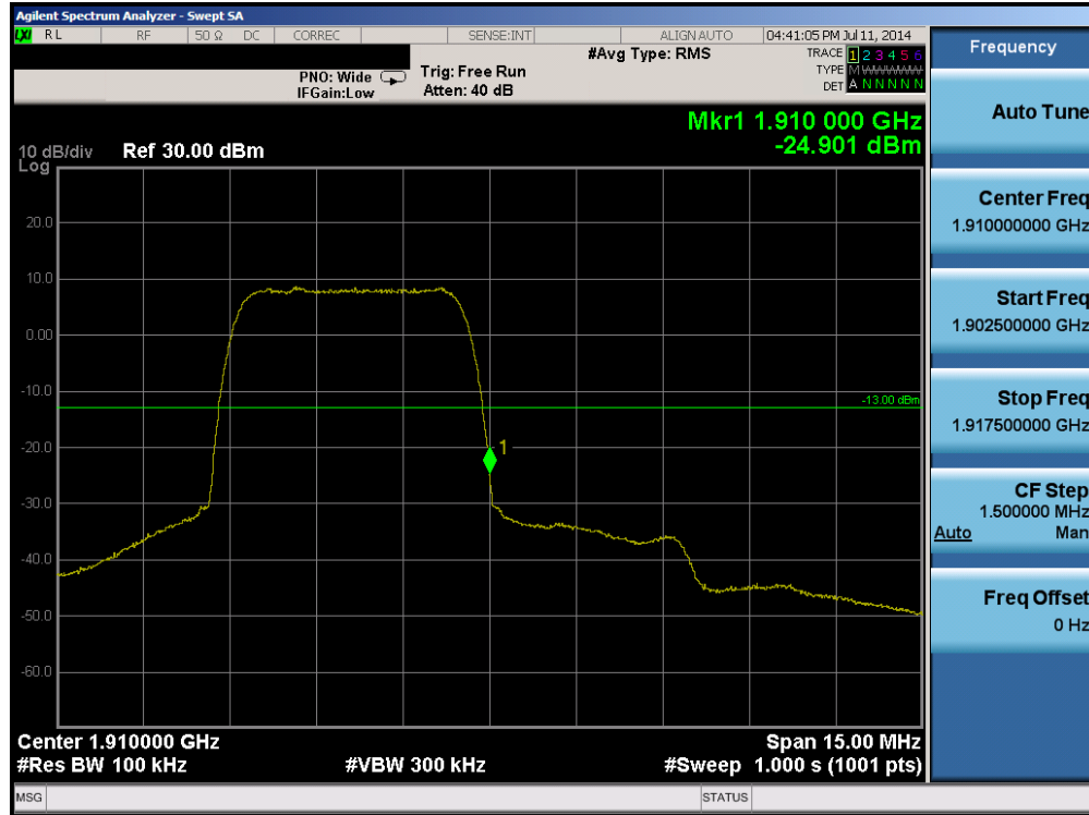
Plot 6-19. Band Edge Plot (PCS WCDMA Mode – Ch. 9538)
