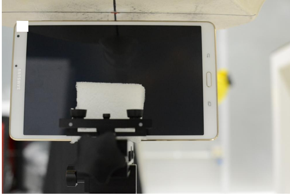
SAR Test Setup Photo 7 – Right Edge at 9 mm
