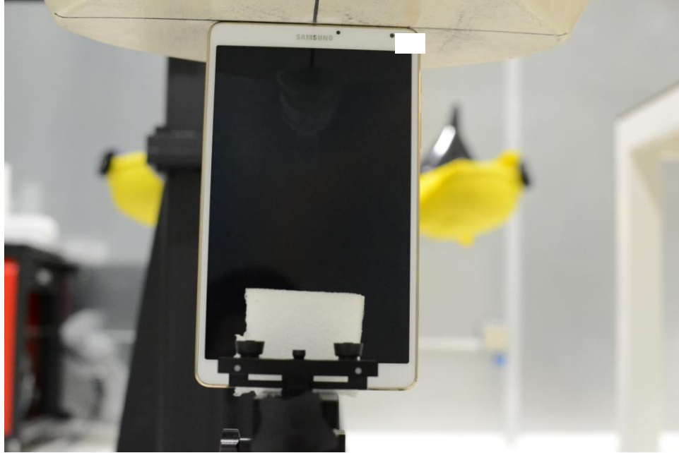
SAR Test Setup Photo 3 – Top Edge at 0.0 mm
