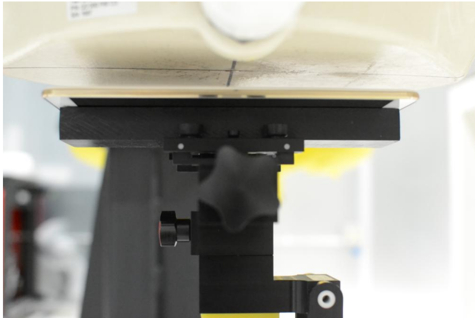
SAR Test Setup Photo 2 – Back Side at 18 mm
