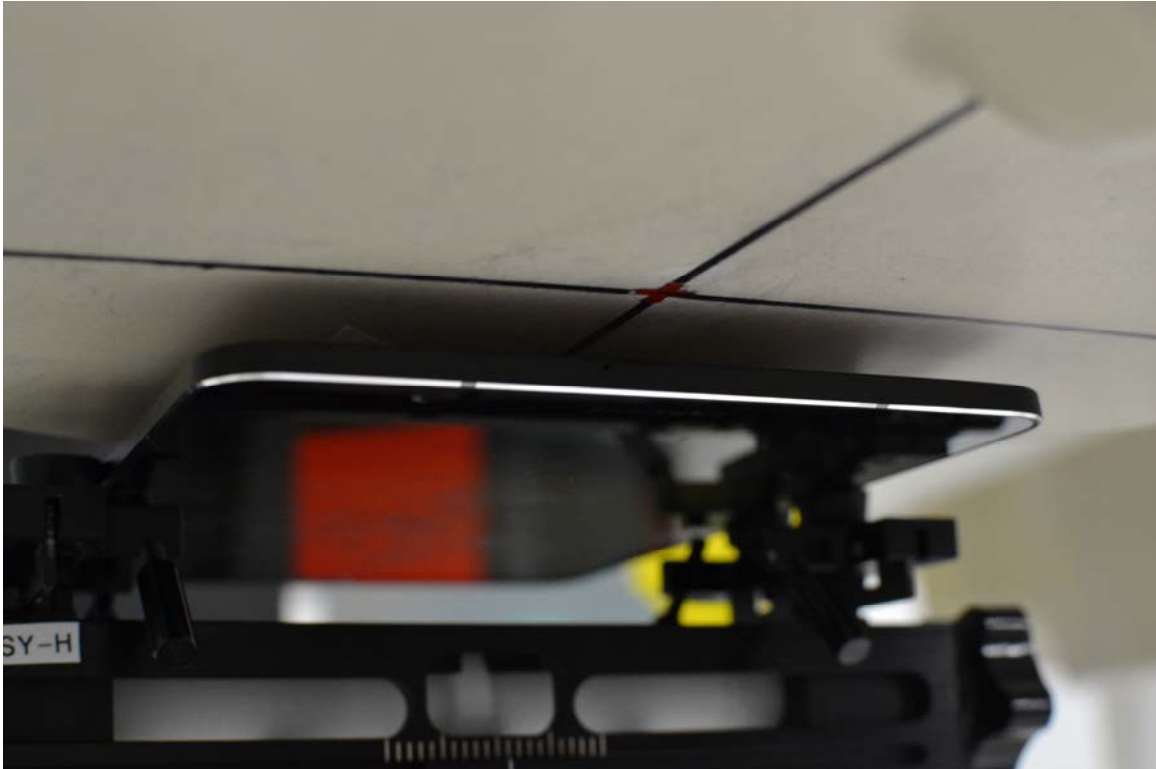
SAR Test Setup Photo 1 – Back Side at 0.7 cm
