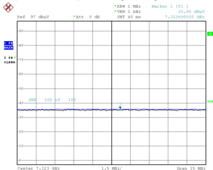
Radiated Spurious Emissions plot – Average Reading ( \pi /4QPSK, Ch.39 3rd Harmonic)
