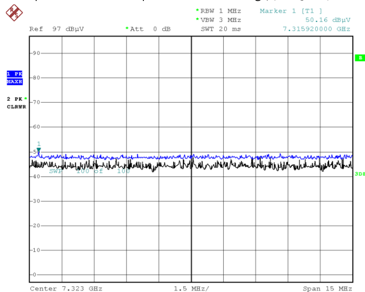
Radiated Spurious Emissions plot – Peak Reading ( \pi /4QPSK, Ch.39 3rd Harmonic)
