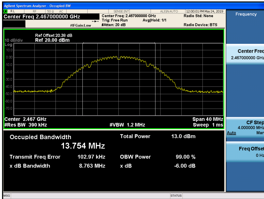
99% Bandwidth plot (802.11b-CH 12)
