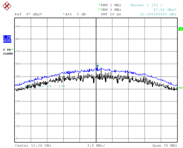
Peak Reading (802.11a, Ch.36 2nd Harmonic, X-V)
