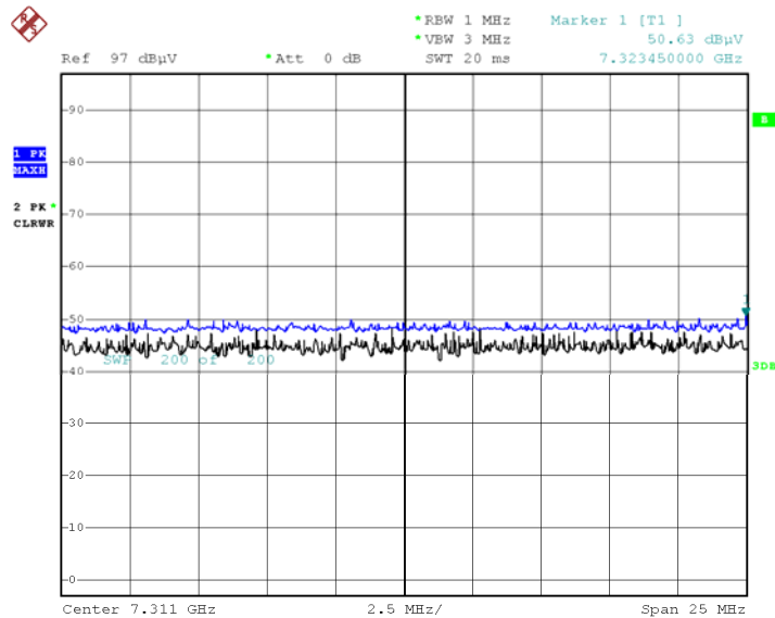
Radiated Spurious Emissions plot – Peak Reading (802.11g, Ch.6 3rd Harmonic, H)
