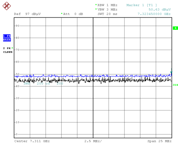
Radiated Spurious Emissions plot – Peak Reading (802.11g, Ch.6 3rd Harmonic, H)
