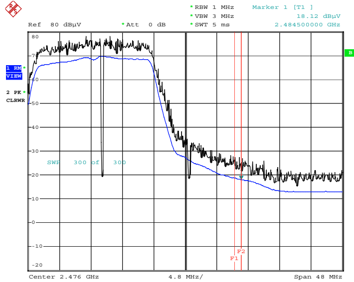
Radiated Restricted Band Edges plot – Average Reading (802.11n(HT20) Ch.11)_ 2484.5 MHz ~ 2.5 GHz
